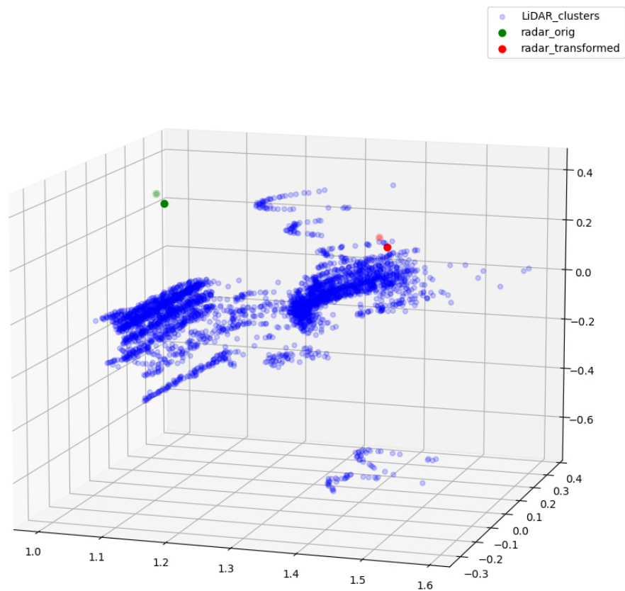
Figure 7. Relative locations of the original radar points (green), transformed radar points (red), and LiDAR point clusters of the moving object (blue).
