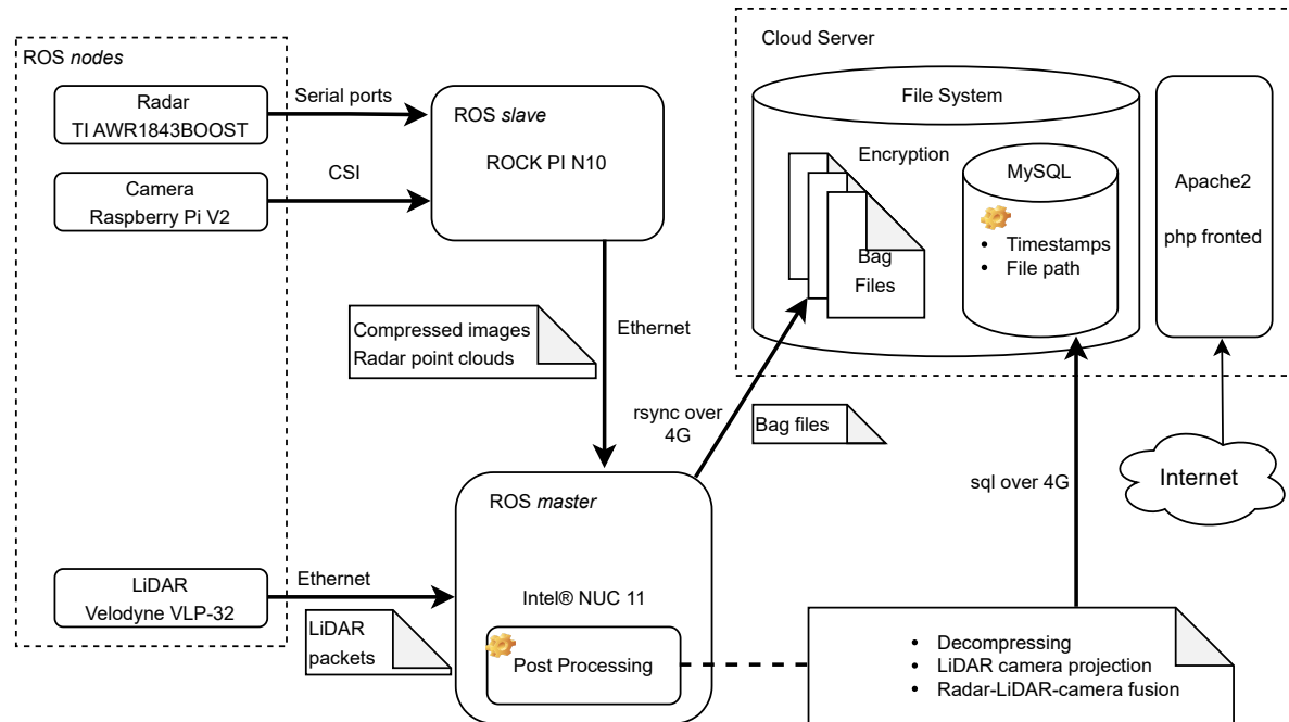
Figure 1. Overview of the framework architecture and data flow. The bold arrow-pointers denote data flow directions and corresponding protocols.
