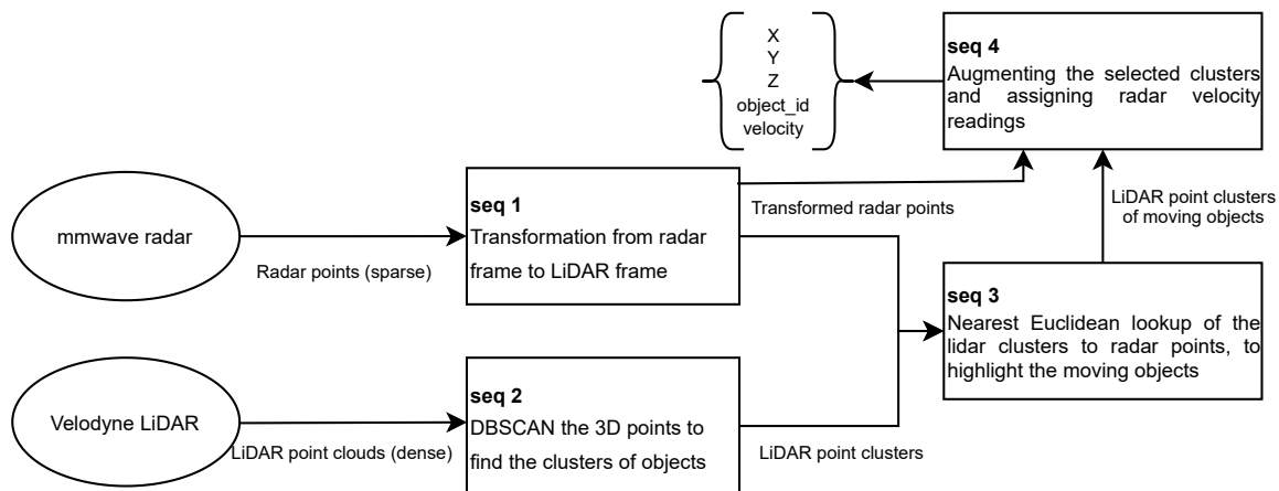
Figure 6. The workflow of radar-LiDAR fusion procedures
