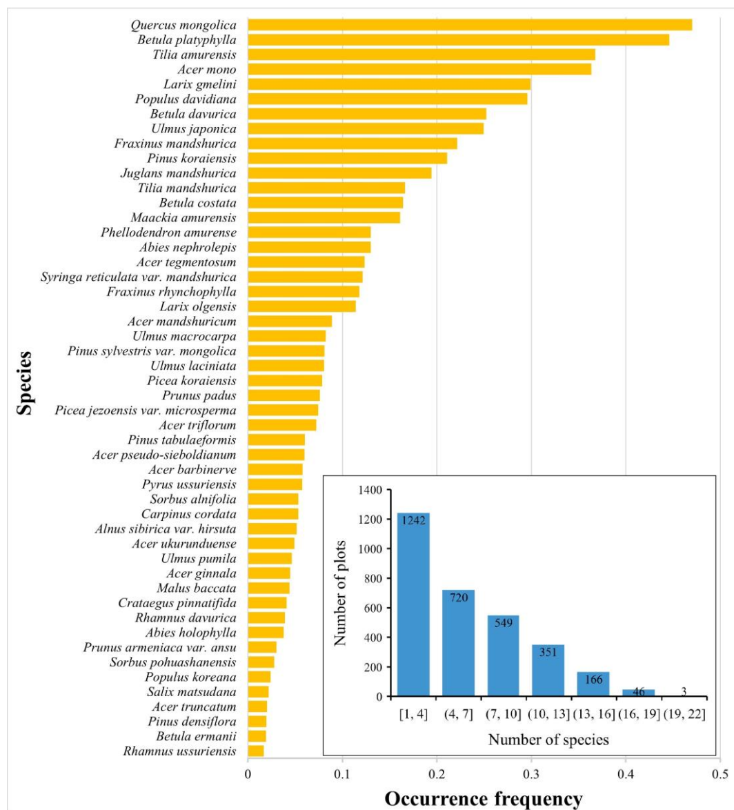
Figure S1 Frequency occurrences of top 50 of 155 species abundance distribution in the 3077 forest plots. The inset histogram is the species-richness distribution of the 3077 plots.
