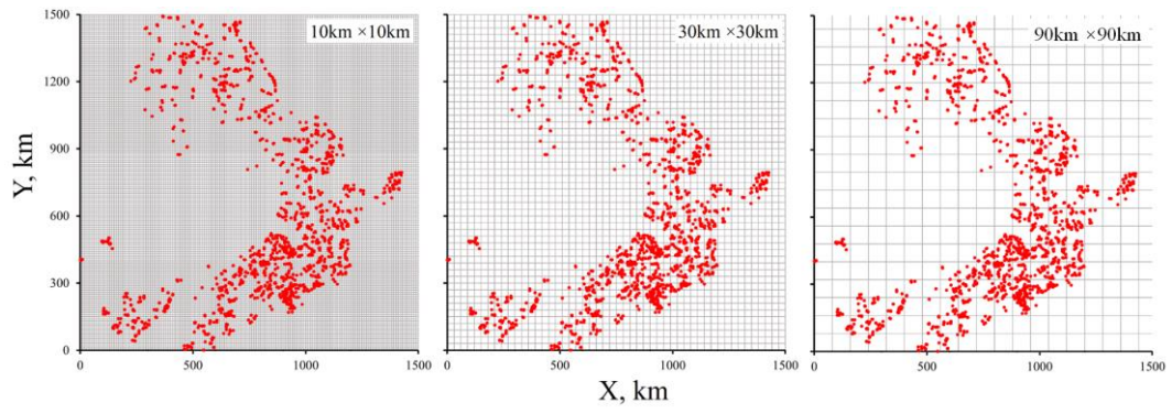
Figure S2 Sampling diagram across the study area. X is the distance of the sample point along the latitude. Y is the distance of the sample point along the longitude. The gray grids were the spatial scale for analysis.
