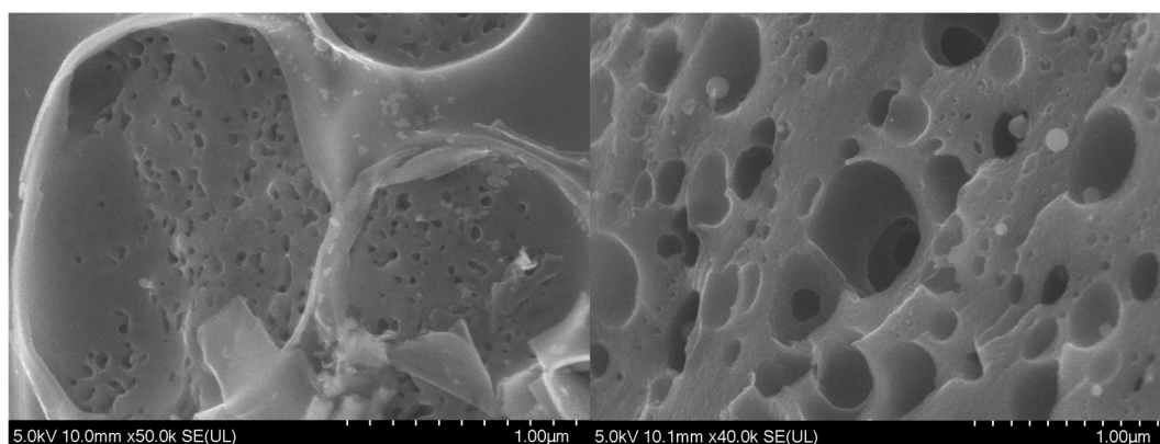
Figure S1. SEM images of (a) RSM-0.33-550 and (b) RSM-1-550.
