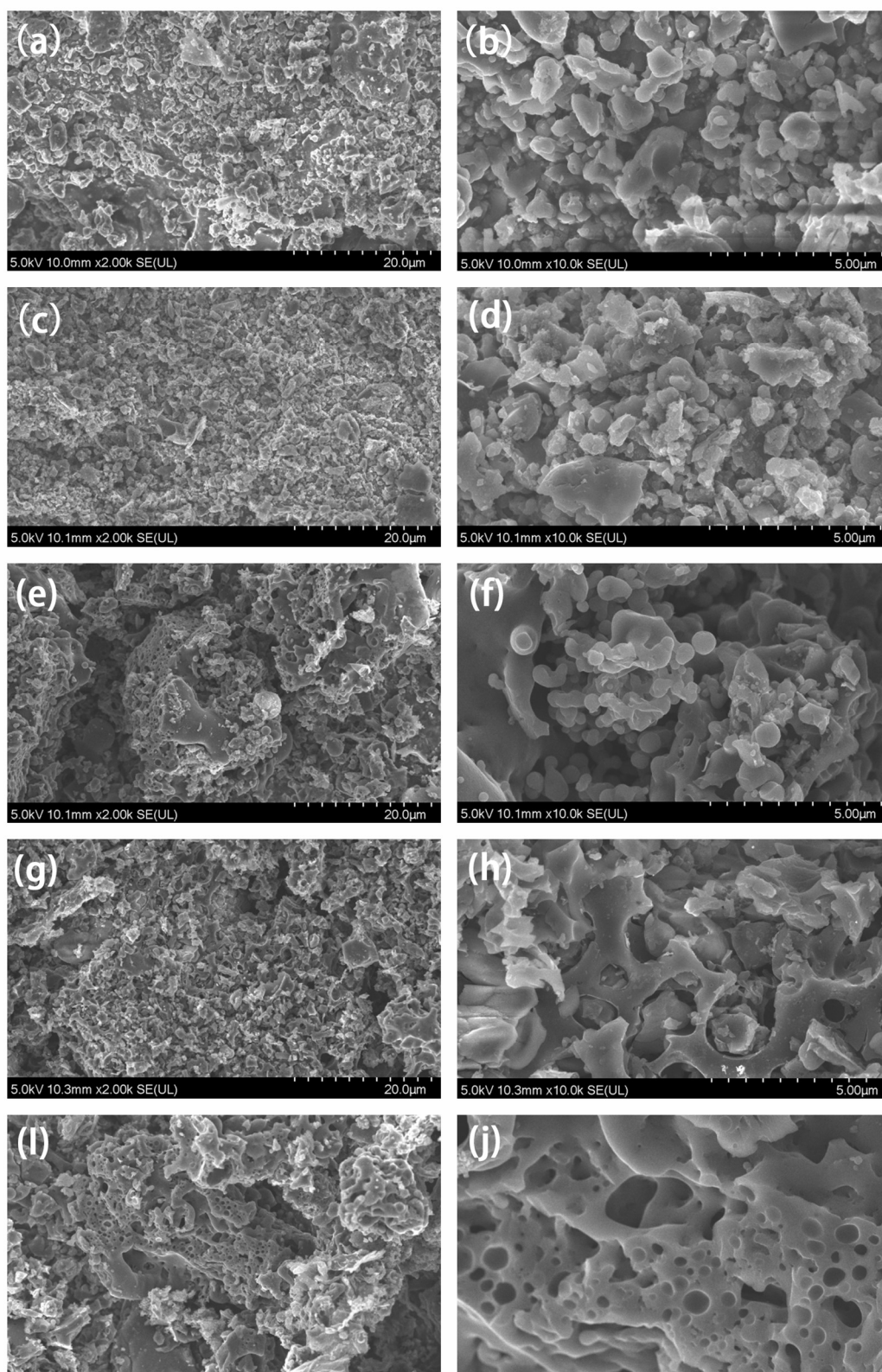
Figure S2. SEM images of (a, b) RSM-1-400, (c, d) RSM-1-500, (e, f) RSM-1-550, (g, h) RSM-1-600, and (i, j) RSM-1-650.
