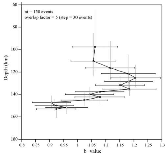
Figure 5. b -value variation with depth for the intermediate-depth Vrancea earthquakes. There are n_i = 150 events in a window that is shifted along the entire depth range with a step of 30 events. The horizontal bars show estimation uncertainties, while the vertical ones show the depth span of each window.
