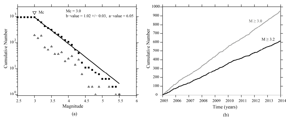
Figure 3. (a) Cumulative (full rectangles) and non-cumulative (empty triangles) number of earthquakes versus magnitude for the intermediate-depth Vrancea earthquakes (ROMPLUS catalog, 60 – 220 km depth), period 2005 – 2013, M \geq 3.0 . The earthquake data is complete above M_c = 3.0 . The black curve is a fit to the data, with the a and b -values of the frequency-magnitude relation determined using a maximum likelihood procedure. (b) Cumulative number of earthquakes with time (years), for two threshold magnitudes (3.0 and 3.2).
