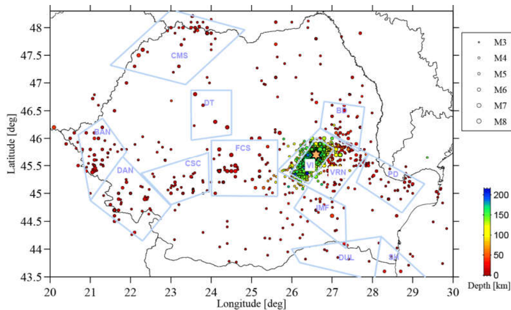
Figure 1. Seismicity of Romania ( M \geq 3.0 ), between 1984 and 2021, according to the ROMPLUS catalog ([4] and [21]). The epicenters of earthquakes are shown by circles, colored as a function of the hypocentral depth and with their size scaling with the magnitude of the earthquake. The yellow star represents the largest historic earthquake occurred in the Vrancea region in 1802, with an estimated magnitude of 7.9. The blue rectangles indicate seismic areas of Romania (modified after [22]): CMS: Crișana-Maramureș, DT: Transylvanian Depression, BAN: Banat, DAN: Danube Zone, FCS: Făgăraș-Câmpulung-Sinaia, VRN: Vrancea, VI: Vrancea subcrustal, IMF: Intra-Moesian Fault, PD: Depression Predoborjeană, BD: Bârlad Depression; SH: Shabla and DUL: Dulovo. We have added the CSC region (modified after [23]; see also [24]), where a recent M5.7 earthquake has occurred in 2023.
