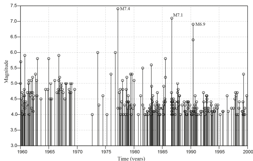
Figure 7. Magnitude versus time for the intermediate-depth Vrancea earthquakes, from 1960 – 2000. The threshold magnitude is M = 4.0 . The three largest earthquakes during the studied period are marked in the figure (1977 M7.4, 1986 M7.1 and 1990 M6.9 Vrancea earthquakes).
