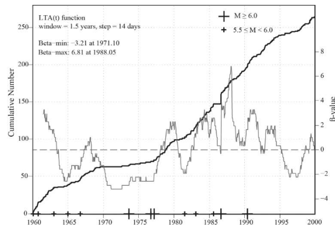
Figure 8. Cumulative number of earthquakes (black curve) and \beta -value variation (LTA(t) function, gray curve) for the Vrancea intermediate-depth earthquakes ( M \geq 4.0 , 1960 – 2000). The window-used to calculate the \beta -value is 1.5 years, moved along the entire time interval with a step of 14 days. The large and small crosses on the time axis indicate events with magnitudes M \geq 6.0 and 5.5 \leq M < 6.0 , respectively.
