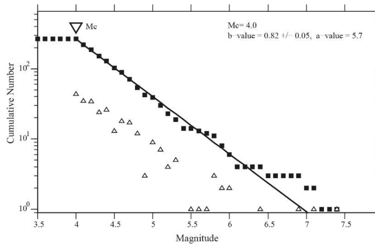
Figure 6. Cumulative (full rectangles) and non-cumulative (empty triangles) number of earthquakes versus magnitude for the intermediate-depth Vrancea earthquakes, ROMPLUS catalog, period 1960 – 2000, M \geq 4.0 . The earthquake data is complete above M_c = 4.0 . The black curve is a fit to the data, with the a and b -values of the frequency-magnitude relation determined using a maximum likelihood procedure.
