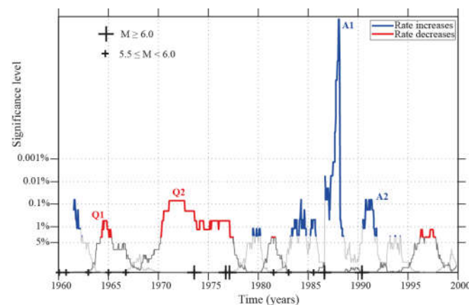
Figure 9. Significance of rate increases and decreases (same window length and step as in Figure 8; gray curves) for the Vrancea intermediate-depth earthquakes ( M \geq 4.0 , 1960 – 2000). Blue and red colors indicate windows of rate increase and decrease, respectively, that have significance levels below 5% (confidence levels above 95%).
