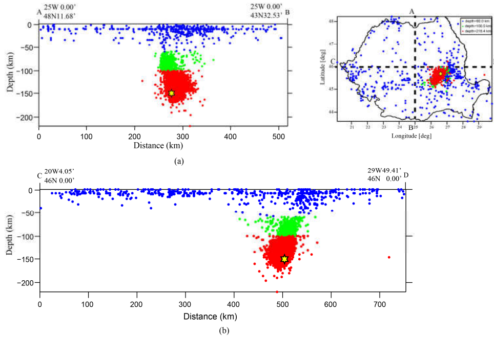
Figure 2. Transverse cross-sections (distance – depth) of seismicity ( M \geq 3.0 ) on the territory of Romania (1984 – 2022), oriented (a) N – S and (b) W – E. The profiles A-B and C-D are shown on the inset map (upper right). The epicenters in the inset map and cross-sections are colored function of depth, as indicated in the inset legend. Yellow star has the same meaning as in Figure 1.
