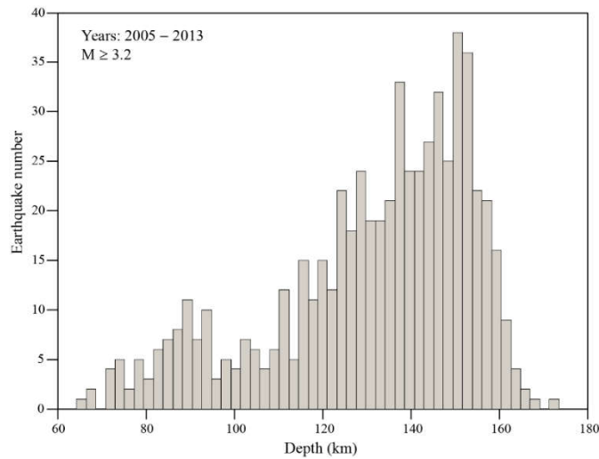
Figure 4. Histogram of earthquakes (2005 – 2013, M \geq 3.2 ) as a function of depth for Vrancea intermediate-depth earthquakes.
