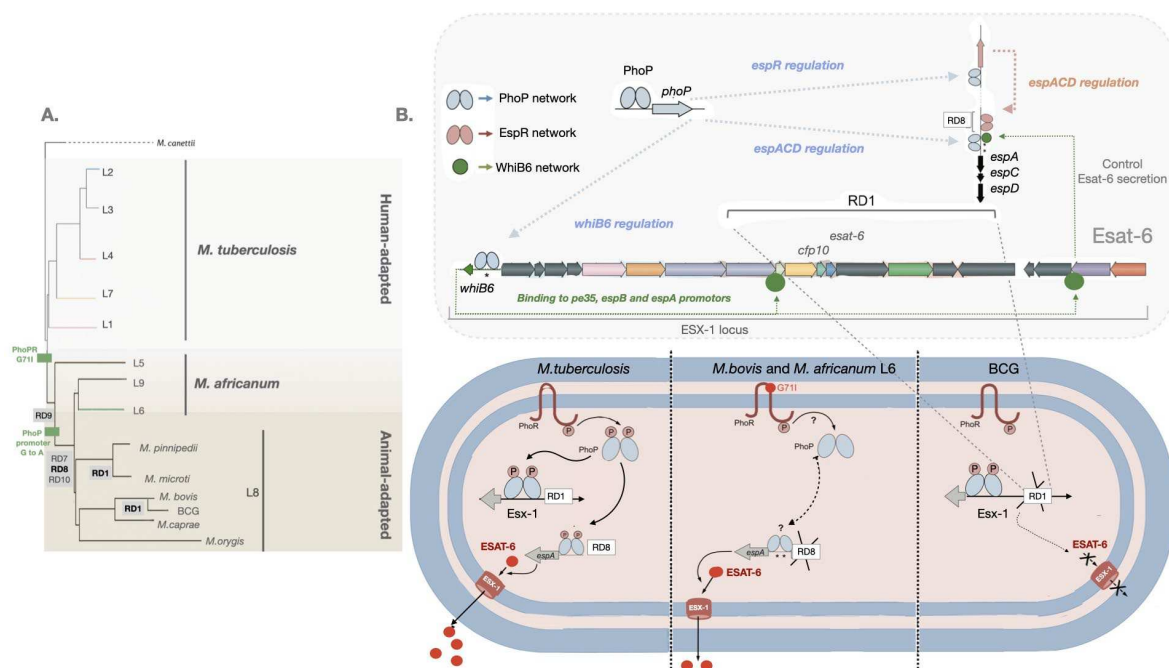
Figure 1. Control of ESAT-6 secretion by PhoP-dependent regulatory networks. (A) Lineages of the MTBC with the RD deletions and PhoPR mutations are highlighted [20,23,28,29]. (B) Several genes from the ESX-1 and the extended ESX-1 ( espACD and espR ) regions required for ESAT-6 protein synthesis and export are displayed. PhoP (blue ellipses) is a transcriptional activator and an effector of the signal transducer PhoR, that interacts with the espR , espA , and whiB6 promoters. In its phosphorylated form, PhoP binds to DNA with higher affinity. Mtb , carrying a functional PhoR, is able to sense a stress-like stimulus and subsequently phosphorylate PhoP. EspR (pink ellipses) activates the espACD locus. WhiB6 (green circles) also interacts with the promoter regions of the espA , pe35 , and espB genes. The espACD locus, is activated by all these circuits and the protein translated EspA is required for ESAT-6 secretion. The RD1, absent in BCG, and of RD8, absent in M. africanum L6 and L8 animal-adapted lineages (including M. bovis ), as well as polymorphisms in the espACD and whiB6 promoters (asterisks) are indicated. M. bovis and M. africanum L6, carrying a defective PhoR G711 allele, are expected to generate a low affinity binding effector due to phosphorylation impairment of PhoP. Nevertheless, ESAT-6 secretion in these species is restored to some extent by compensatory mutations in the espACD promoter region, including RD8 deletion and species-specific polymorphisms (asterisks) [62].
