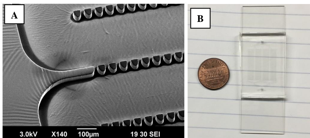
Figure S1. A) SEM image of the device. The image shows the main coil channel and the arrangement of side filters. B) Finished device.
