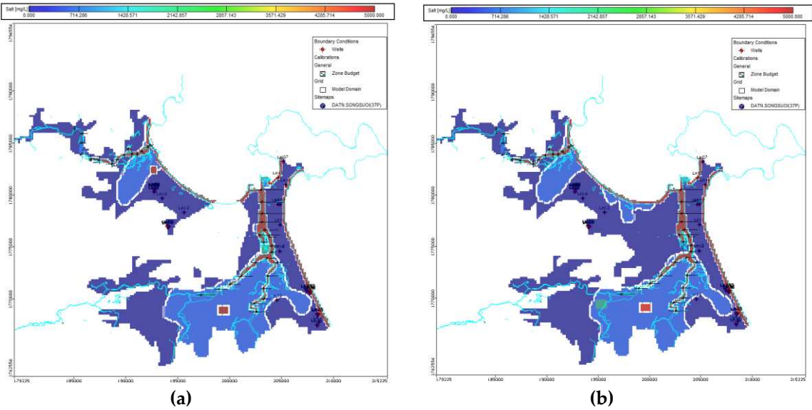
Figure 7. Saltwater intrusion distribution in groundwater of the study site in April 2020 (modeled using Visual MODFLOW) (a) Depicting the distribution in the Holocene aquifer; (b) Depicting the distribution in the Pleistocene aquifer.
