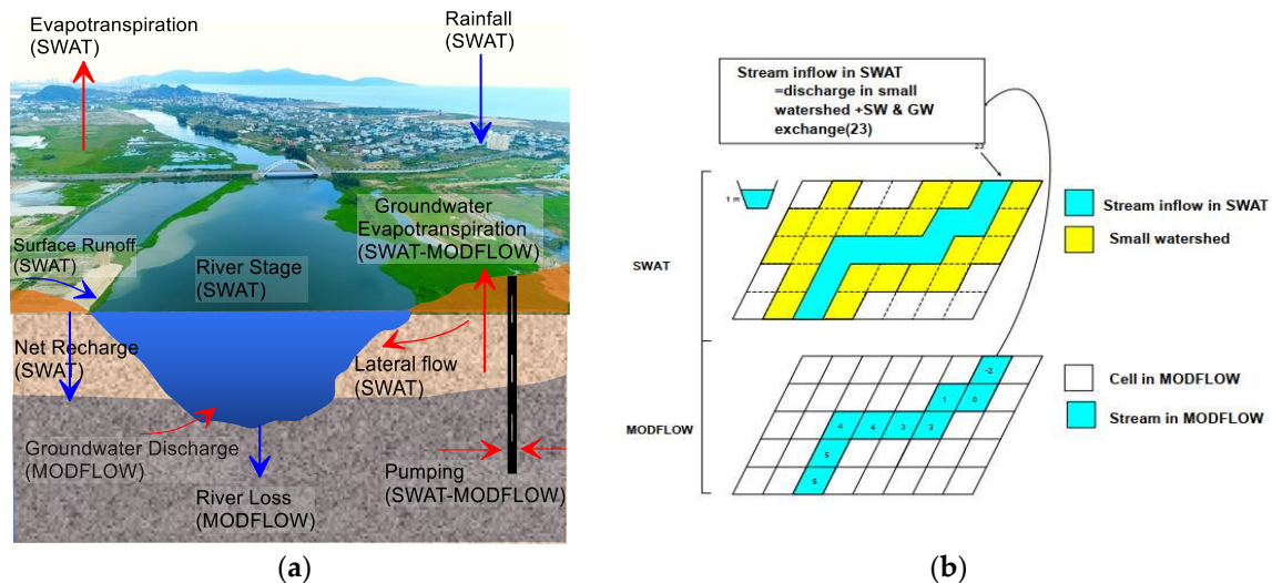
Figure 2. A combination of surface water and groundwater models for hydrological analysis in Da Nang coastal area (a) [6] and the linkage of a river in MODFLOW with SWAT (b) [19].
