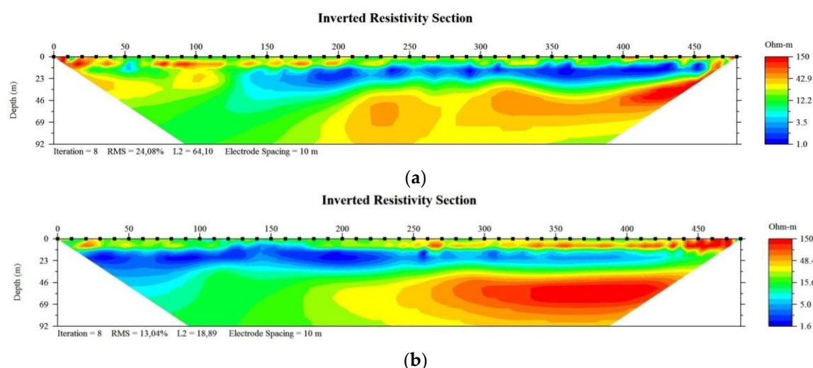
Figure 3. 2-D electrical resistivity tomography (ERT) of Section 2 (a) and Section 13 (b).
