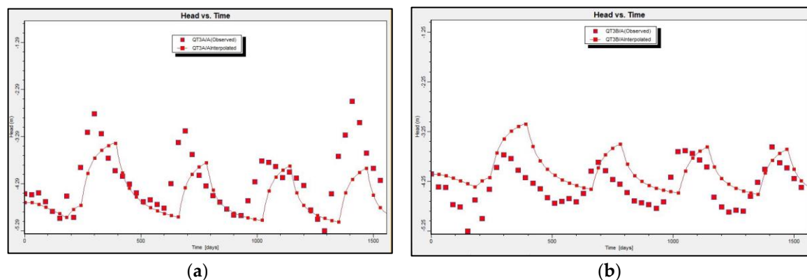
Figure 6. Simulated and observed groundwater head values at observation borehole QT3A (a) and QT3B (b).
