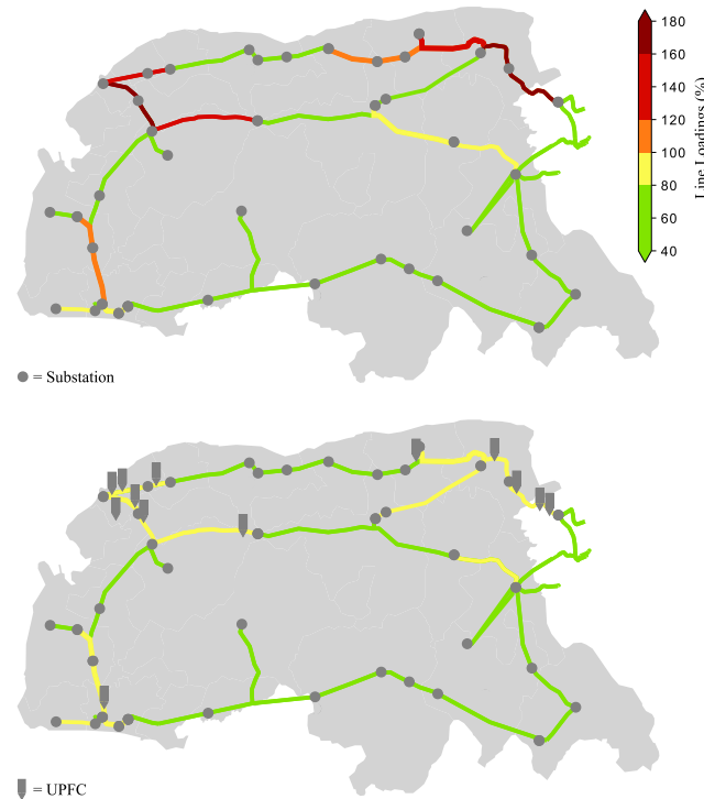
Figure 7. The reference case (above) and with the optimal UPFCs (beneath). Geographical information based on OpenEnergy project [30].
