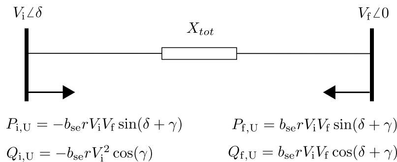
Figure 2. The PIM of UPFC on a line [16, fig. 6].
