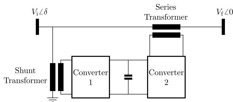
Figure 1. Basic setup of UPFC [16, Fig. 1].
