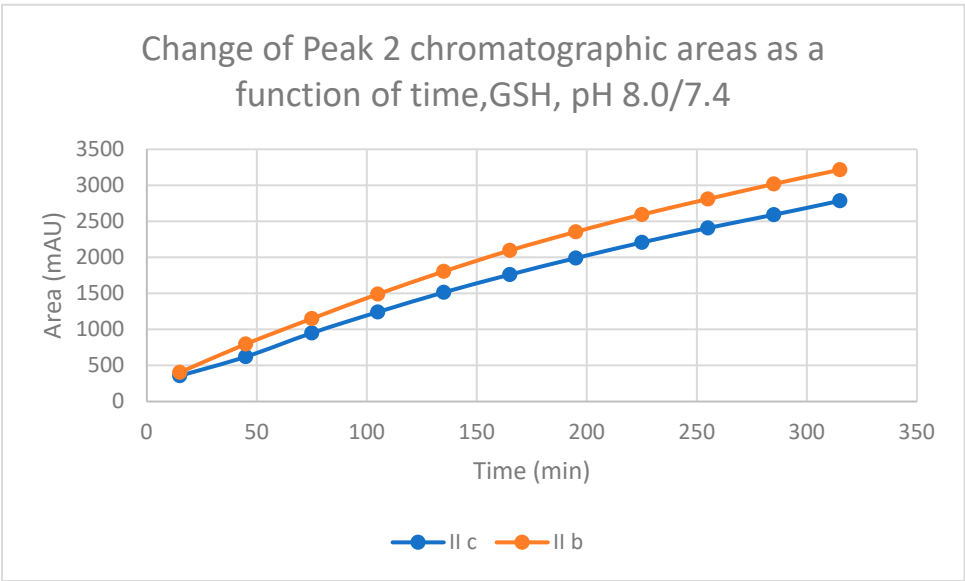
Figure 5. Change in the chromatographic peak area of adduct 2 of IIb and IIc in the chalcone-GSH incubations at pH 8.0/7.4.
