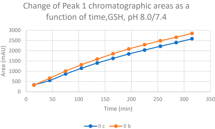
Figure 4. Change in the chromatographic peak area of adduct 1 of IIb and IIc in the chalcone-GSH incubations at pH 8.0/7.4.
