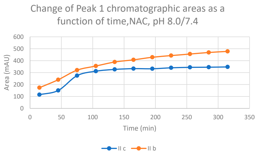
Figure 6. Change in the chromatographic peak area of adduct 1 of IIb and IIc in the chalcone-NAC incubations at pH 8.0/7.4.
