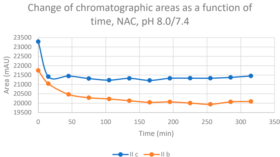
Figure 3. Change in the chromatographic peak area of chalcones IIb and IIc in the chalcone–NAC incubations at pH 8.0/7.4.
