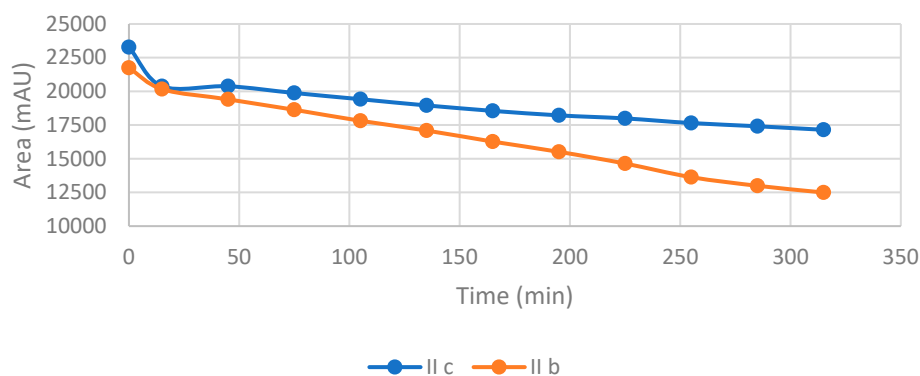
Change of chromatographic areas as a function of time, GSH, pH 8.0/7.4
