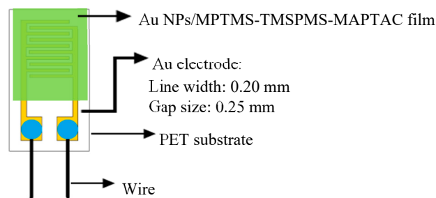
Figure 1. Schematic diagram of flexible humidity sensor.
