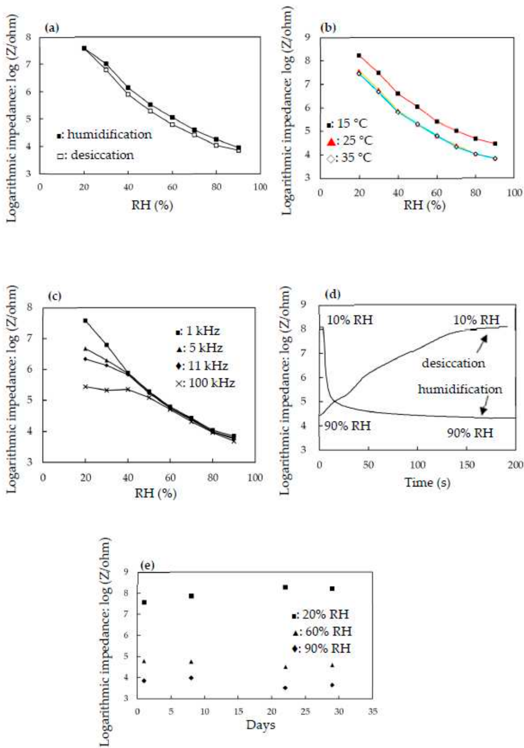
Figure 9. Humidity-sensing properties of the flexible humidity sensor based on Au NPS/ MPTMS-TMSPMA-MAPTAC composite film. (a) Hysteresis of the sensor, (b) effect of ambient temperature, (c) effect of applied frequency, (d) response/recovery times, (e) long-term stability.
