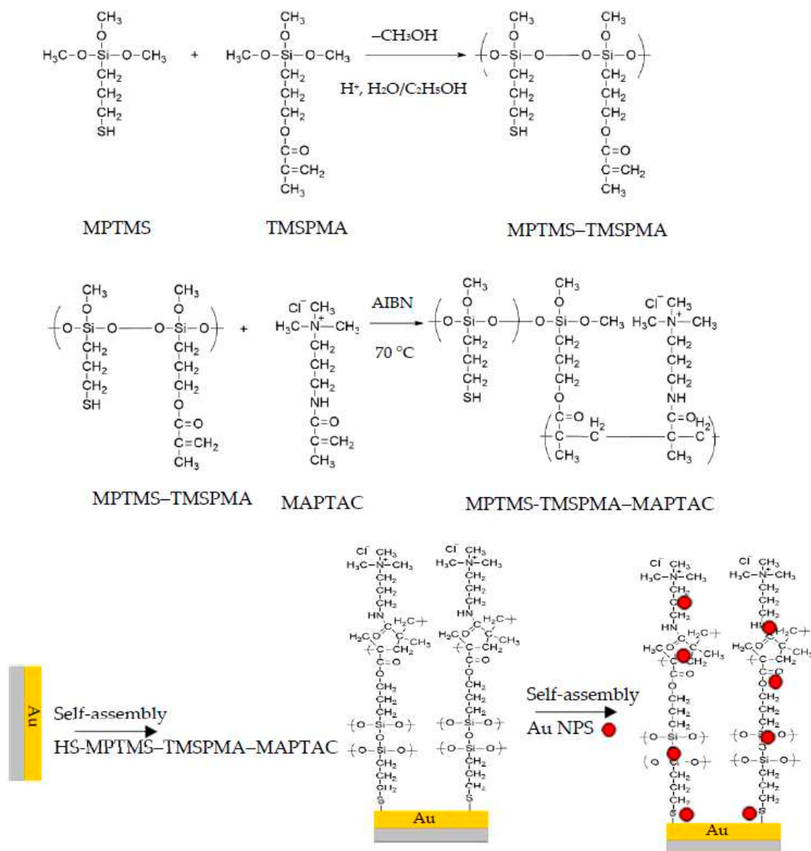
Figure 2. Fabrication of a flexible humidity sensor based on Au NPs/MPTMS-TMSPMA-MAPTAC film by combining the sol-gel process, free radical polymerization, and self-assembly method.
