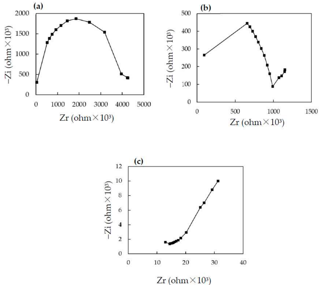
Figure 10. Complex impedance plots of the flexible humidity sensor based on Au NPs/MPTMS-TMSPMA-MAPTAC composite film at (a) 30% RH, (b) 40% RH (c) 90% RH.
