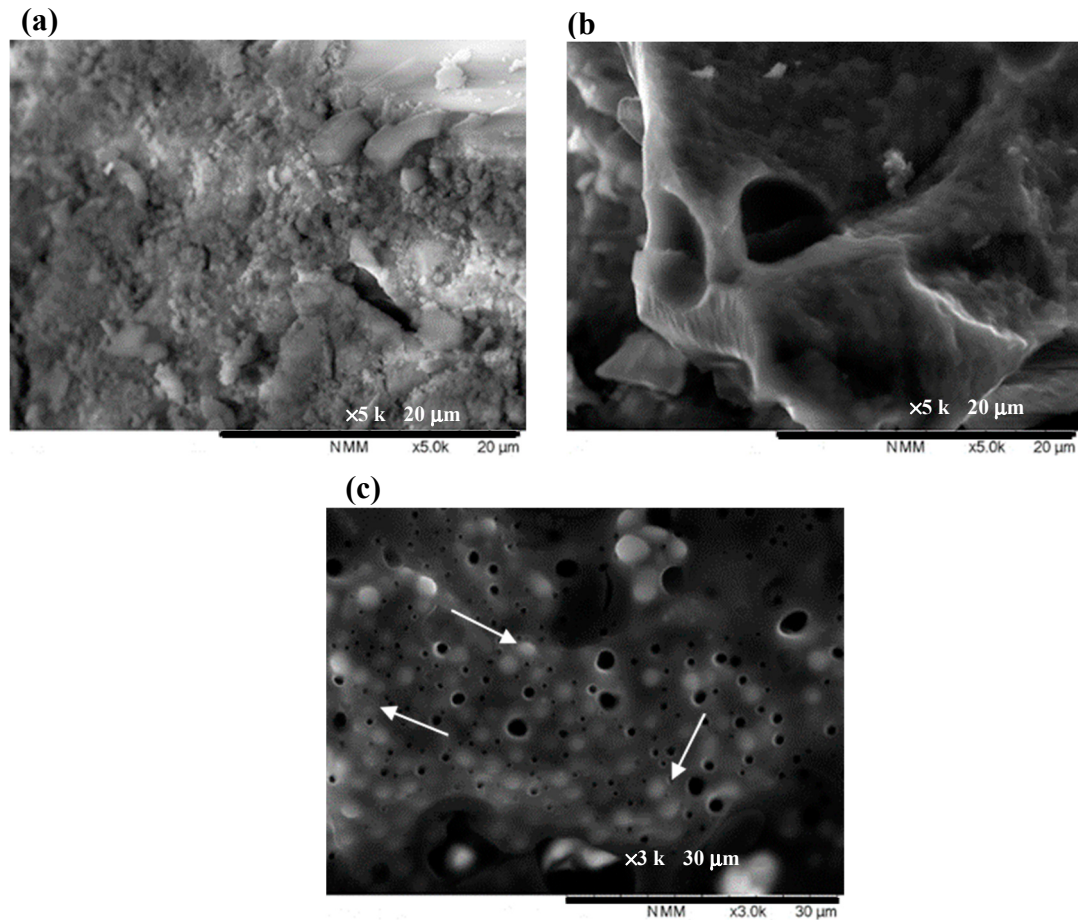
Figure 5. SEM images of (a) pristine SiO 2 film, (b) MPTMS-TMSPMA-MAPTAC film and (c) Au NPs/MPTMS-TMSPMA-MAPTAC composite film. (White arrows indicated the Au NPs).
