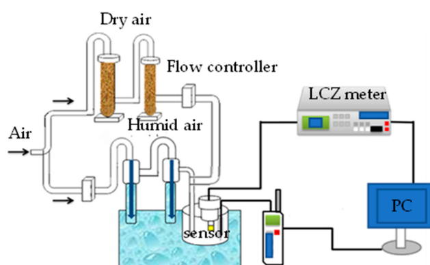
Figure 3. Schematically plots the humidity atmosphere controller system and impedance measurement of flexible humidity sensors.
