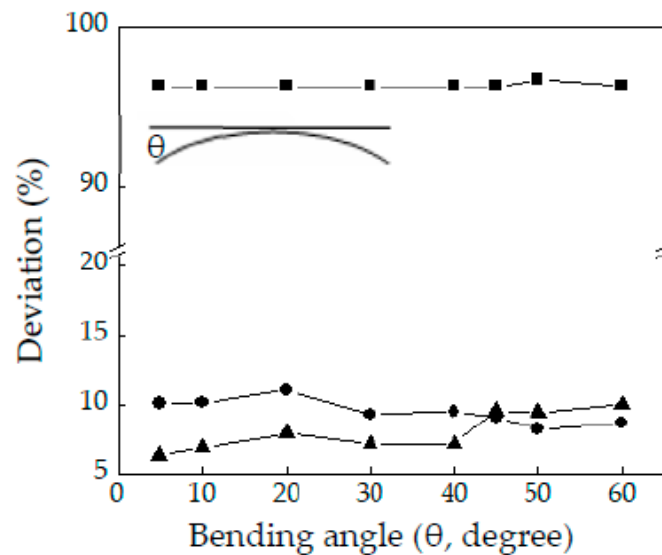
Figure 7. Flexibility of ■: pristine SiO 2 film, ▲: MPTMS-TMSPMA-MAPTAC film and ●: Au NPs/MPTMS-TMSPMA-MAPTAC composite film on PET substrate, measured at 1 V, 1 kHz and 25 °C.
