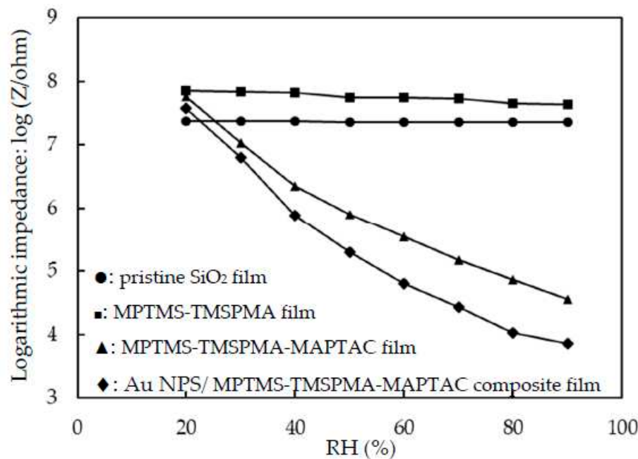
Figure 8. Impedance versus RH for flexible humidity sensors based on pristine SiO 2 , MPTMS-TMSPMA, MPTMS-TMSPMA-MAPTAC and Au NPs/MPTMS-TMSPMA-MAPTAC composite films, measured at 1 V, 1 kHz and 25 °C.
