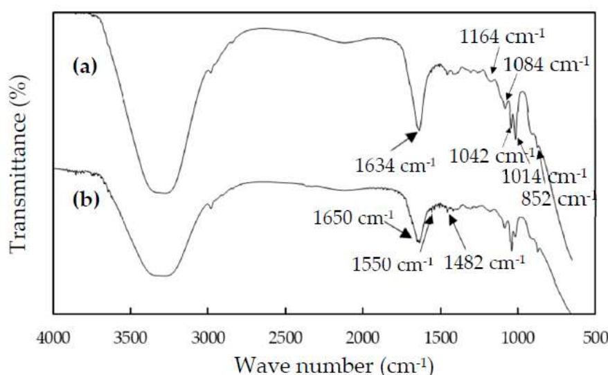
Figure 4. IR spectra of (a) MPTMS-TMSPMA and (b) MPTMS-TMSPMA-MAPTAC sol-gel.
