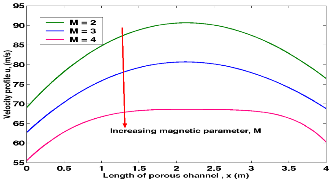
Figure 4.1: Velocity profile against Length of Porous channel at varying Magnetic parameter
