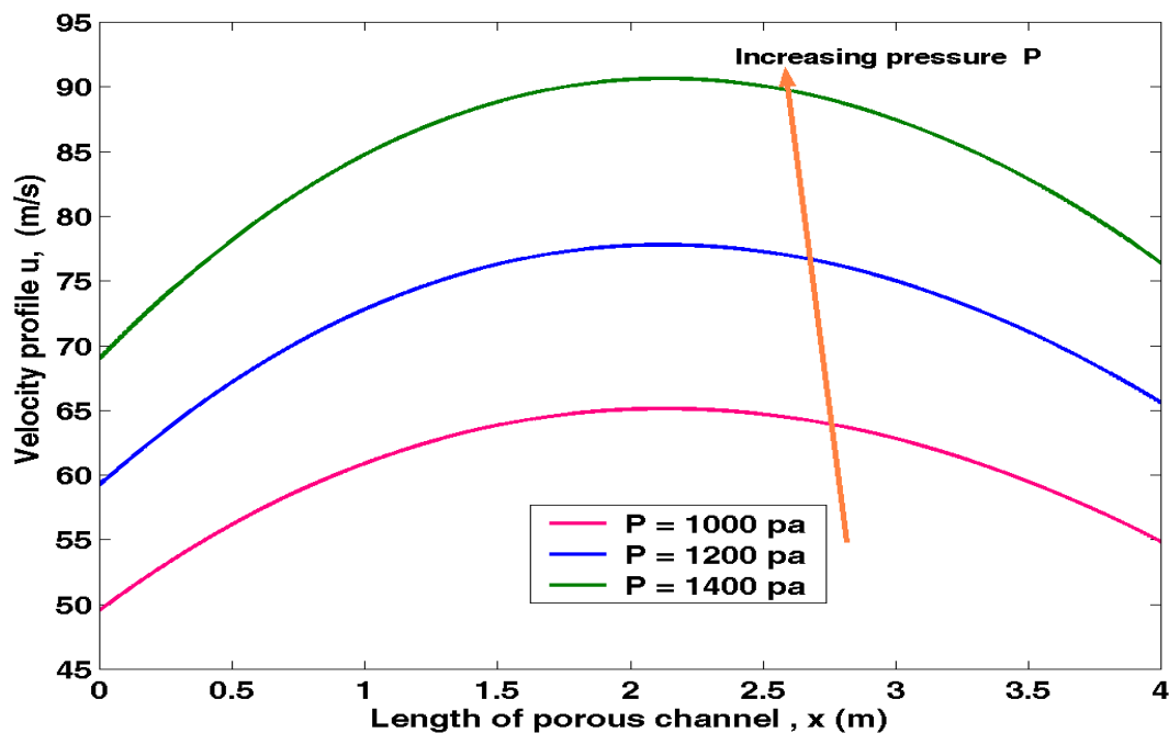
Figure 4.3: Graph of velocity profile against Length of Porous channel at varying fluid pressure.
