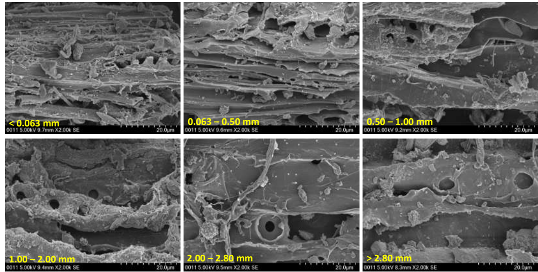
Figure 1. Representative SEM images of biochar by particle size fraction.
