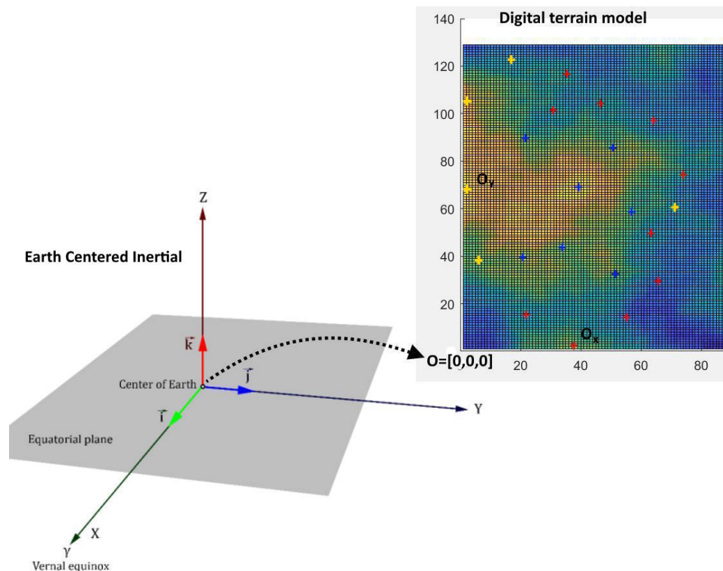
Figure 1. Digital terrain model and the origin O
