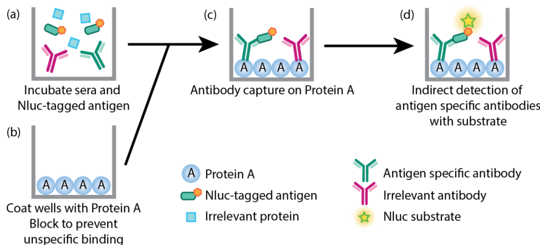
Figure 1. Schematic of modified LACA developed to study ASFV antigen specific antibody responses of immunized and challenged animals. (a) Sera samples are incubated with cell lysates containing a mixture of specific Nluc-tagged ASFV proteins of interest and irrelevant proteins. (b) Plates are coated with Protein A and blocked to prevent unspecific binding. (c) Nluc-tagged antigens bound to their respective antibodies are then captured on protein A and (d) the presence of antigen binding antibodies is indirectly measured through the Nluc activity. Irrelevant antibodies bound to Protein A are not detected since these do not bind the Nluc-tagged antigens.
