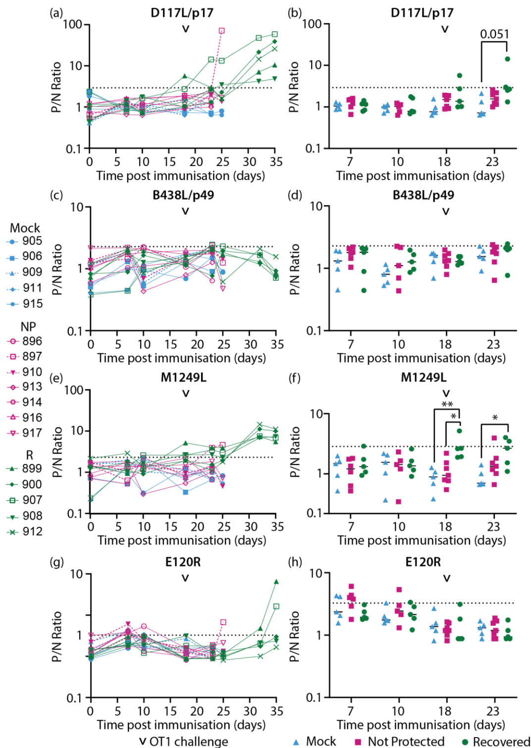
Figure 4. Longitudinal antibody responses of inbred Babraham pigs to ASFV recombinant capsid proteins (a-b) D117L/p17, (c-d) B438L/p49, (e-f) M1249L and (g-h) E120R/p14.5 detected with antigen specific LACAs at selected dpi. (a, c, e, g) Antigen specific antibody kinetics of each animal are plotted. (b, d, f, h) Antibody responses consolidated as a group at each relevant time point are plotted. Only time points where there were four data points or more were included in this analysis. Lines indicate the mean. Each data point corresponds to a single animal. The point of challenge with virulent OURT88/1 (OT1, 18 dpi) is denoted by the arrowhead in each graph. P/N Ratio: ratio of luciferase activity of each sample to the luciferase activity of the negative control. Dashed line indicates the cutoff determined from the mean and 3 \times standard deviation of all negative sera samples in each experiment. Blue, Mock: mock control animals immunized with PBS, Pink, NP:
