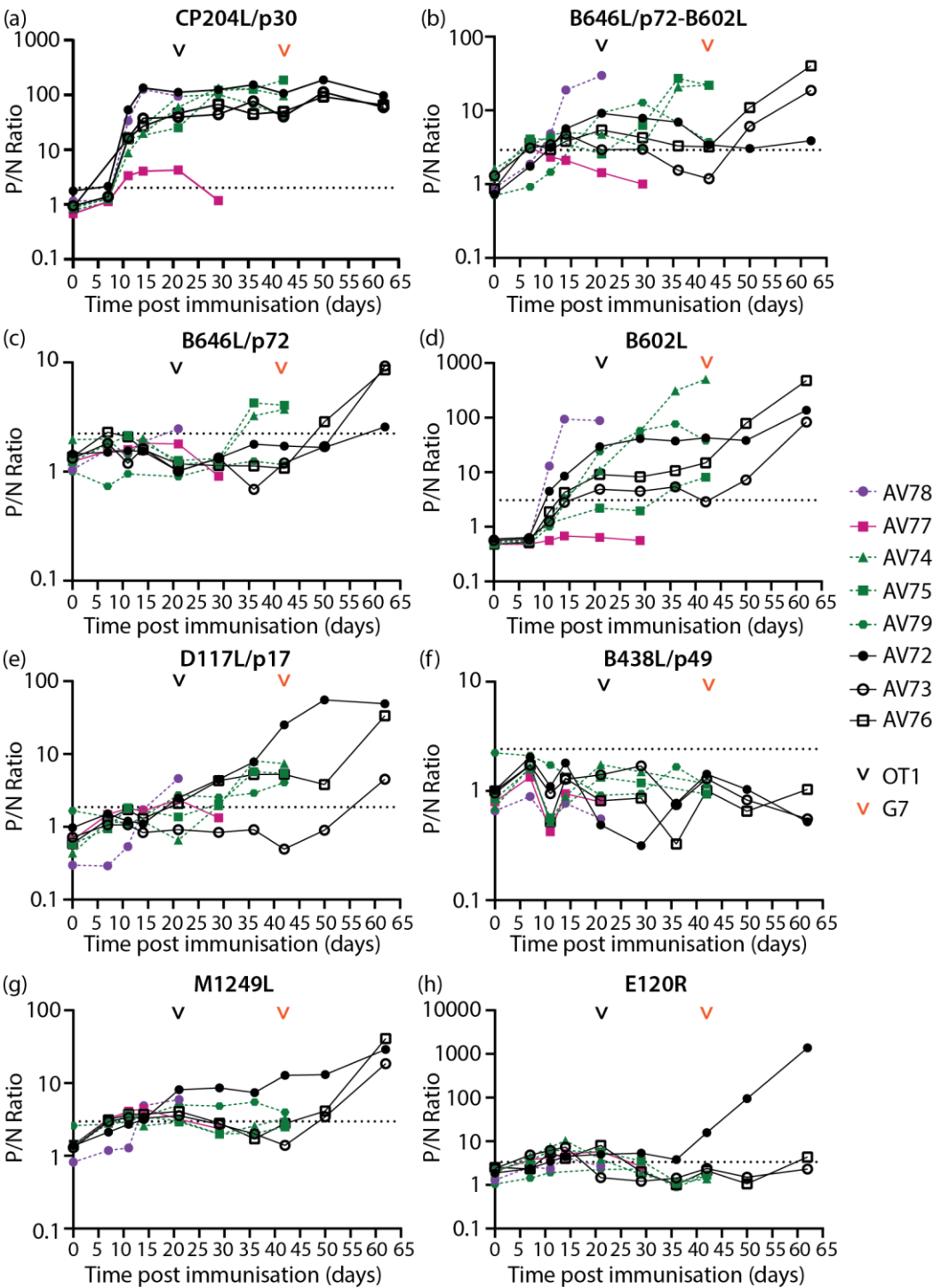
Chronic ASF OT1 Not Protected OT1 Recovered, G7 Not Protected OT1 Recovered, G7 Recovered Figure 7. Longitudinal antibody responses of outbred domestic pigs to ASFV recombinant proteins (a) CP204L/p30, (b) B646L/p72 co-expressed with chaperone B602L, (c) B646L/p72, (d) B602L chaperone, (e) D117L/p17, (f) B438L/p49, (g) M1249L and (h) E120R/p14.5 detected with protein specific LACAs at selected dpi. Antigen specific antibody kinetics of each animal are plotted. Each data point corresponds to a single animal. The point of challenge with virulent OURT88/1 (OT1, 21 dpi) and virulent Georgia 2007/1 (G7, 42 dpi) is denoted by the black and orange arrowheads, respectively. P/N Ratio: ratio of luciferase activity of each sample to the luciferase activity of the negative
