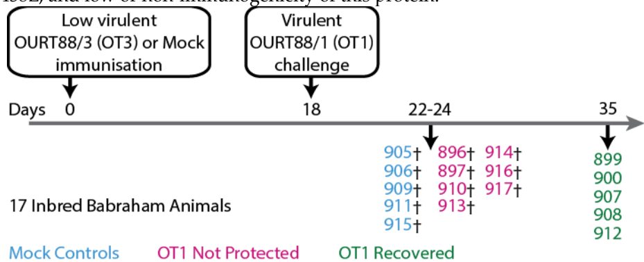
Figure 2. Schematic representation of experiment involving large-white inbred Babraham pigs that were immunized with low virulent OURT88/3 (OT3) before challenge with virulent OURT88/1 (OT1) as published previously [51]. Partial protection from challenge with related ASFV was observed.
