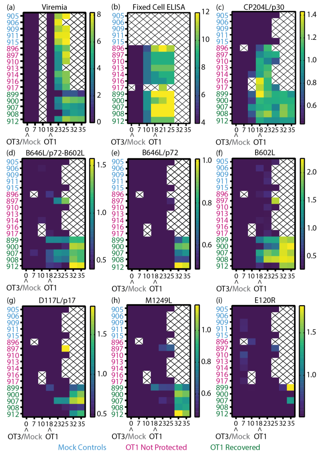
Figure 5. Heatmaps of the virological and immunological parameters of inbred Babraham animals. (a-b) Data reported previously [51], (a) viremia, (b) anti-ASFV antibody titer as determined by fixed cell ELISA on BA71V infected Vero cells [51], and (c-i) recombinant ASFV protein specific LACAs targeting (c) CP204L/p30, (d) B646L/p72 co-expressed with B602L chaperone, (e) B646L/p72, (f) B602L chaperone, (g) D117L/p17, (h) M1249L and (i) E120R/p14.5. Data plotted as (a) Log10 genome copy numbers/ml, (b) Log2 antibody titer, (c-i) Log10 of P/N ratio. Each row denotes the responses of a single animal. The negative cutoff for each protein specific LACA was determined from the mean and 3x standard deviation of all negative sera samples in each experiment. Animal
