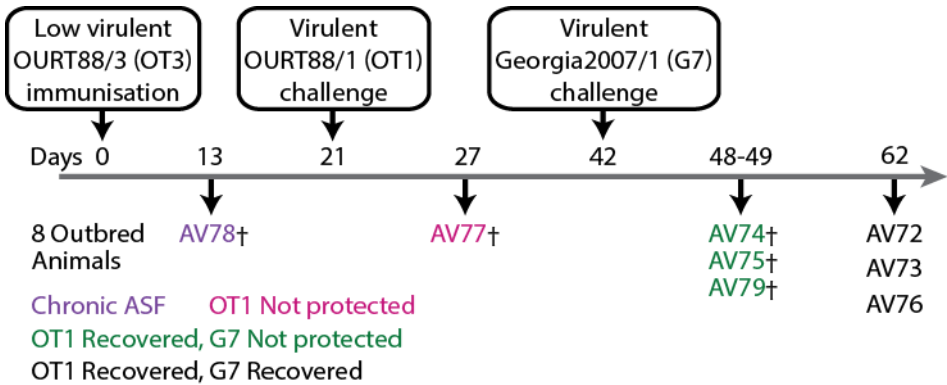
Figure 6. Schematic representation of experiment involving outbred domestic pigs that were immunized with low virulent OURT88/3 and challenged with the related virulent OURT88/1.
