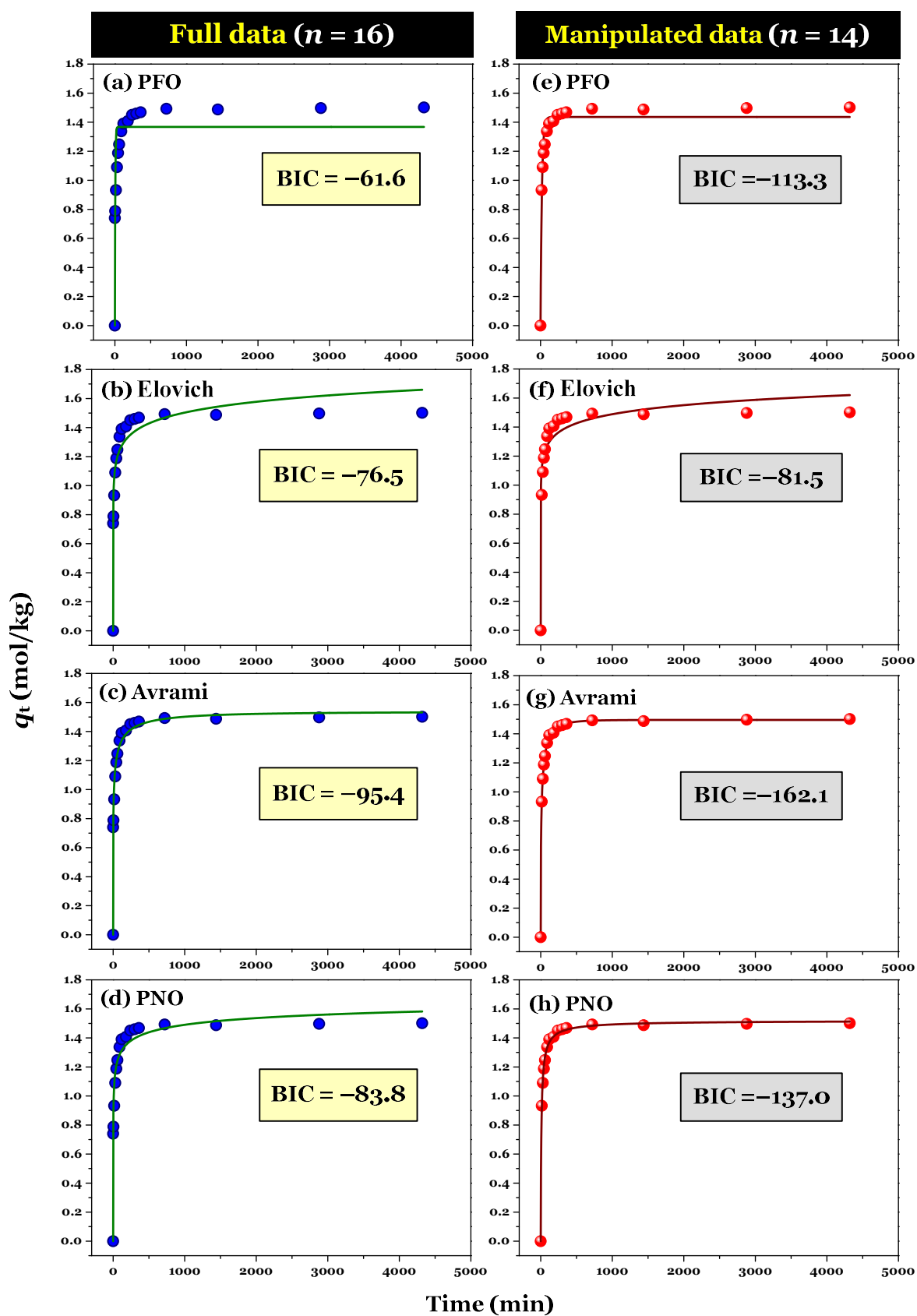
Figure S3. Adsorption kinetic of paracetamol by commercial activated carbon fitted by various adsorption kinetic models
