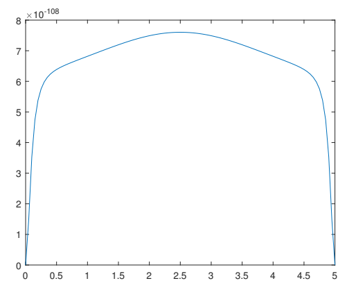
Figure 12. Solution \phi_S(x) for the \omega = 1.8 .
