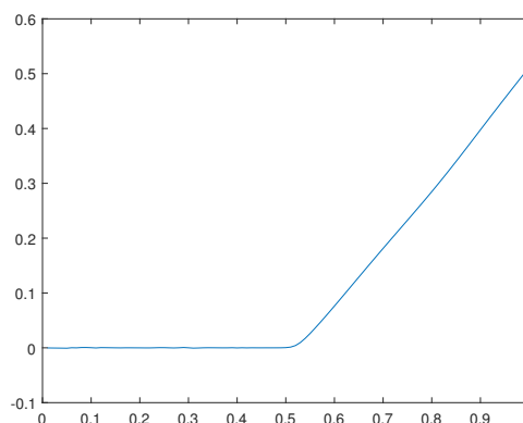
Figure 38. Optimal solution u(x) for the case f(x) = 0 .
