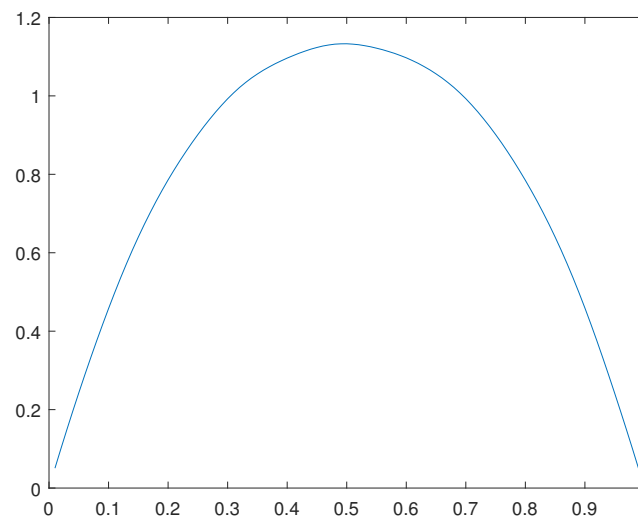
Figure 44. Solution \hat{u}_0(x) through the dual functional for \varepsilon = 0.1 .
