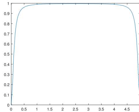
Figure 14. Solution \phi_S(x) for the \omega = 1.0 .
