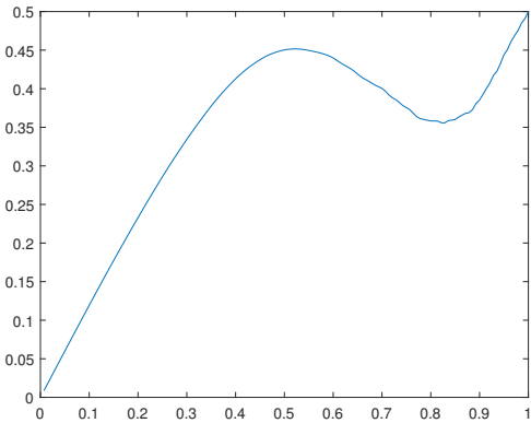
Figure 29. Optimal solution u_0(x) for the case f(x) = \sin(\pi x)/2 .
