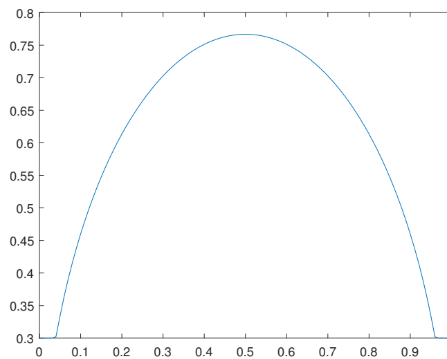
Figure 39. Optimal solution L_1(x) for the case A.
