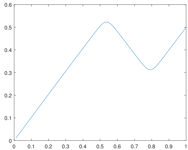
Figure 34. Optimal solution u(x) for the case f(x) = \sin(\pi x)/2 .
