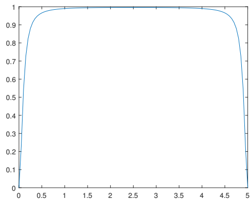
Figure 11. Solution \phi_N(x) for the \omega = 1.8 .
