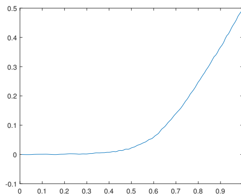
Figure 31. Optimal solution u_0(x) for the case f(x) = 0 .
