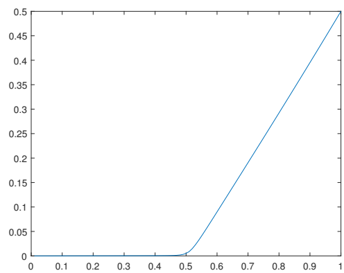
Figure 28. Optimal solution u(x) for the case f(x) = 0 .
