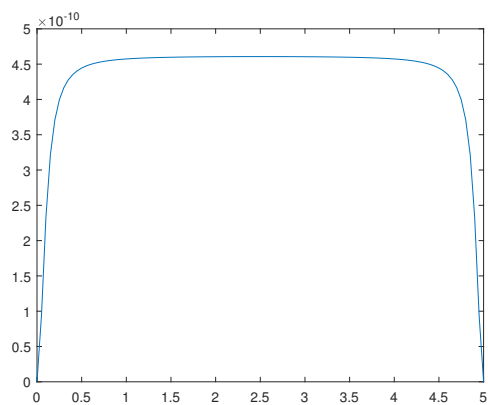
Figure 13. Solution \phi_N(x) for the \omega = 1.0 .
