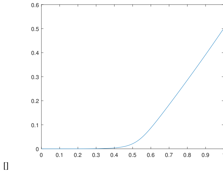
Figure 3. solution u_0(x) for the case f(x) = 0 .
