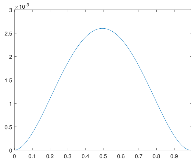
Figure 19. Solution u(x) for the example B.
