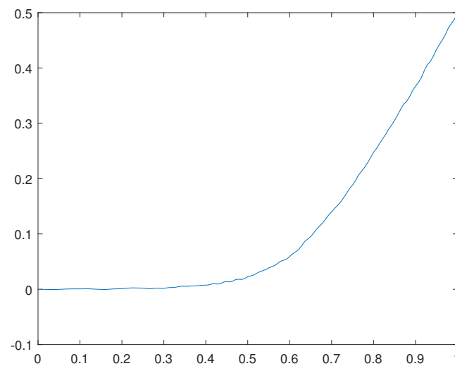
Figure 31. Optimal solution u_0(x) for the case f(x) = 0 .
