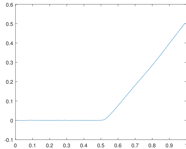
Figure 38. Optimal solution u(x) for the case f(x) = 0 .
