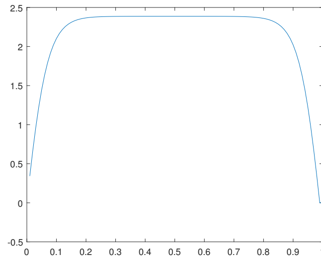
Figure 36. Optimal solution u(x) for the case A.
