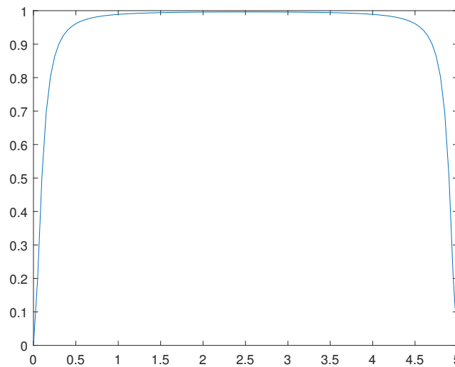
Figure 14. Solution \phi_5(x) for the \omega = 1.0 .
