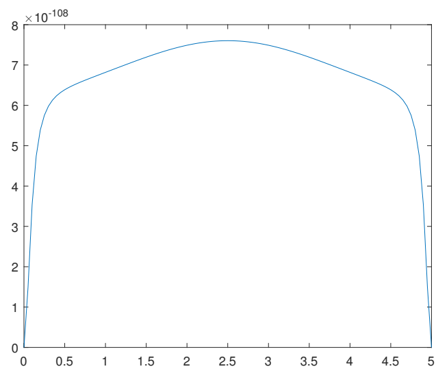
Figure 12. Solution \phi_5(x) for the \omega = 1.8 .
