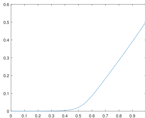
Figure 3. solution u_0(x) for the case f(x) = 0 .
