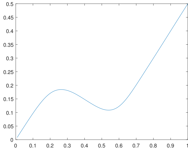
Figure 9. Solution u_0(x) for the example A.
