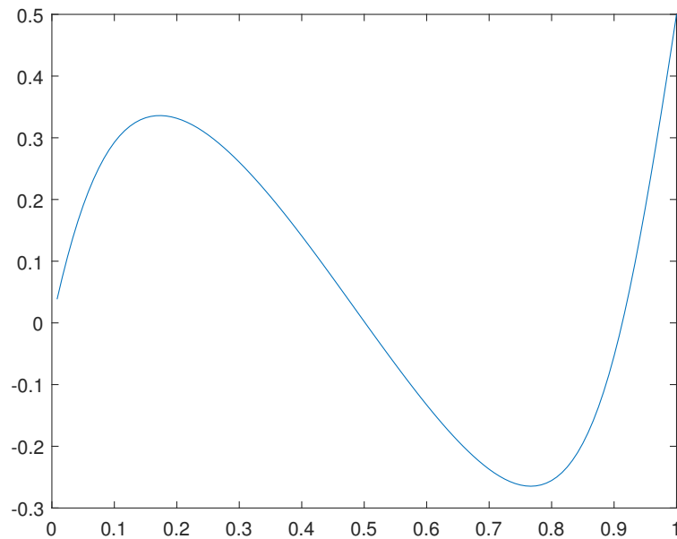
Figure 10. Solution u_0(x) for the example B.
