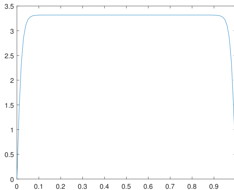
Figure 8. Solution u(x) = v_3^*(x)/\beta for the example 2.
