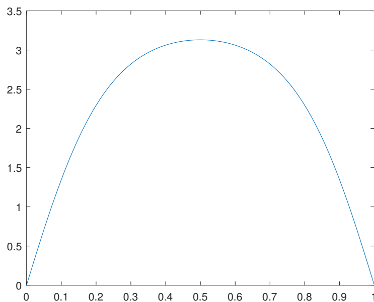
Figure 7. Solution u(x) = v_3^*(x)/\beta for the example 1.
