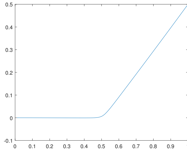
Figure 35. Optimal solution u(x) for the case f(x) = 0 .
