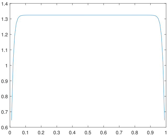
Figure 49. Solution u_0(x) through the dual functional for the case C, \varepsilon = 0.001 .
