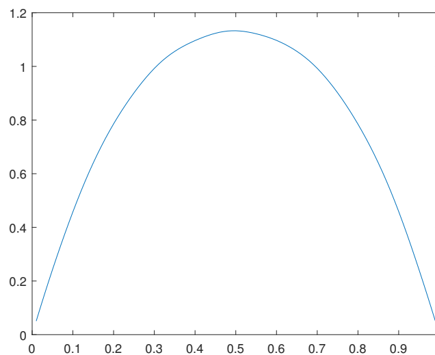
Figure 45. Solution \hat{u}_0(x) through the dual functional for \varepsilon = 0.1 .
