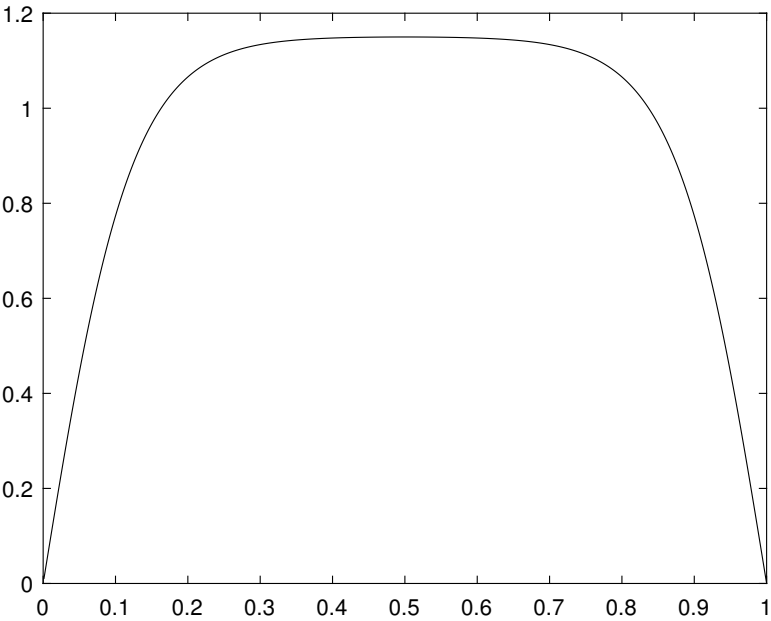
Figure 43. Solution u(x) for \varepsilon = 0.01
