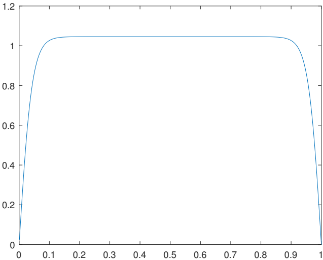
Figure 44. Solution u(x) for \varepsilon = 0.001
