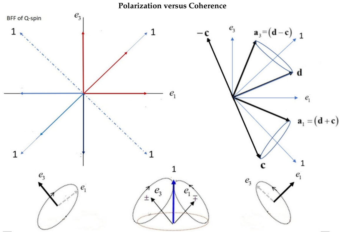
Figure 5. Top Left: Alice's spin (red lines in the (1,1) quadrant) and Bob's spin (blue lines in the (-1,-1) quadrant) are oriented anti-parallel in the BFF. All vectors are unit. The superposition of the two axes of spin \frac{1}{2} , e_3 and e_1 creates the Q-spin of magnitude 1.
