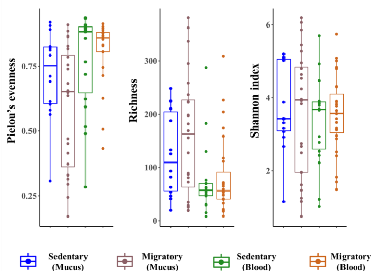
Figure 3. Alpha diversity analysis of both S. trutta phenotypes for circulating and mucosal microbiomes. Species evenness, observed richness and Shannon diversity indexes were calculated for each group. No significant differences were observed between migratory and sedentary specimens for the same compartment.
