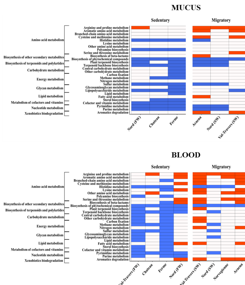
Figure 8. Heatmaps show the relative abundance (natural logarithm base) of metabolic pathways based on 16S rRNA data in migratory and resident trout collected in different sites.
