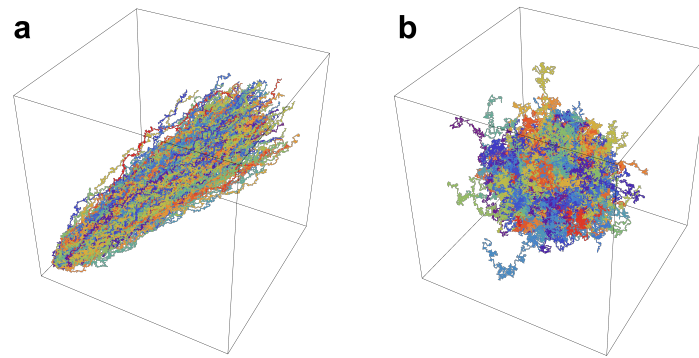
Figure 1. Simulation results of the trajectories of 300 particles randomly moving for 10 s ( c = 10 , u = 6 and \sigma = 2 ). a , group speed of u . b , group speed of 0.
