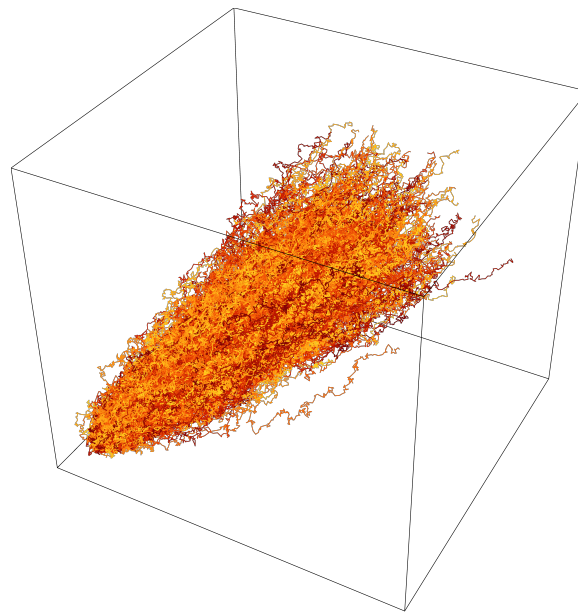
Figure 1. Simulation results of the trajectories of 500 particles randomly moving for 50 s ( c = 1 , u = 0.6 and \sigma = 1 ).
