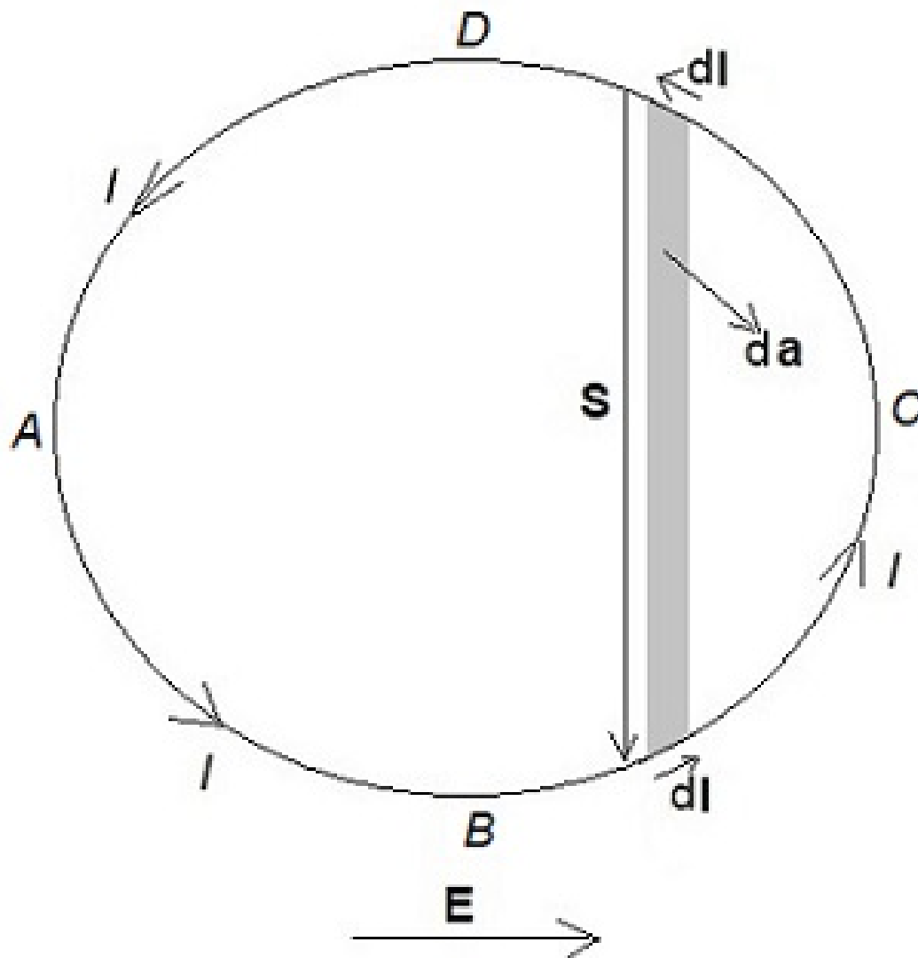
Figure 3. A current loop ABCD is carrying current I . There is an electric field \mathbf{E} , uniform over the current loop. The electric field \mathbf{E} does positive work, I\mathbf{E} \cdot d\mathbf{l} on a current element d\mathbf{l} in the arc ABC of the current loop and an equal and opposite work on a similar current element d\mathbf{l} in the arc CDA , the two current elements separated by a distance S , on two opposite sides of the current loop. This implies transfer of an infinitesimal electromagnetic energy, between two current elements across the shaded area da of the circuit, which represents an element of electromagnetic momentum in the system.
