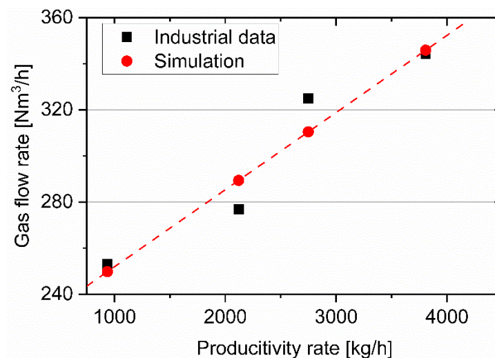
Figure 2. Simulated values of gas consumption in roller kiln for firing cycle compared to industrial data for different productivity.
