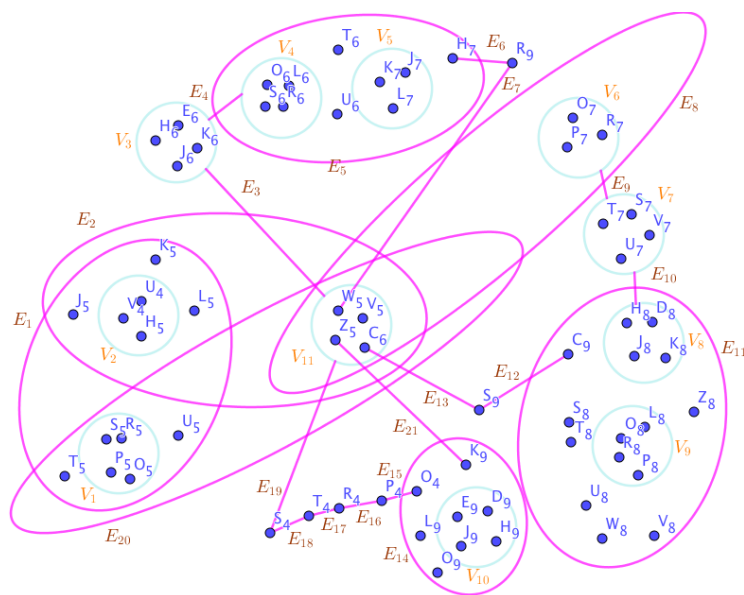
Figure 1. A SuperHyperGraph, is called “SuperHyperFlower”, Associated to the Notions of SuperHyperGirth in the Example (2.3)
