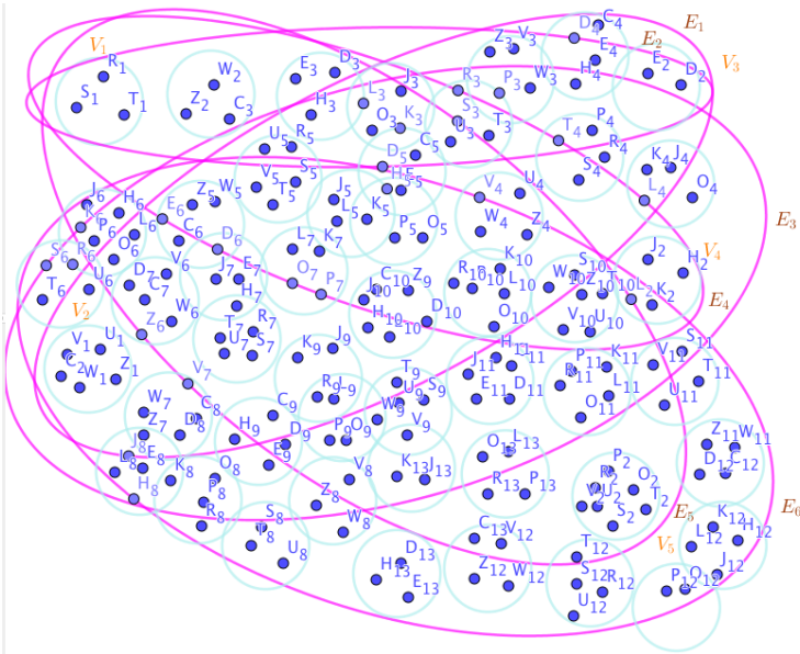
Figure 17. A SuperHyperBipartite Associated to the Notions of SuperHyperGirth
