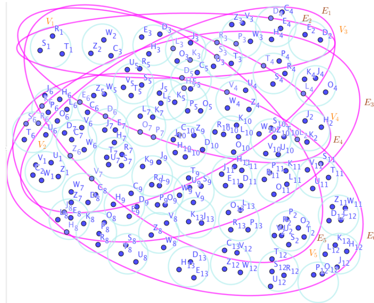
Figure 8. A SuperHyperBipartite Associated to the Notions of SuperHyperGirth in the Example (4.8)
