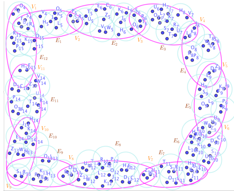
Figure 6. A SuperHyperCycle Associated to the Notions of SuperHyperGirth in the Example (4.4)
