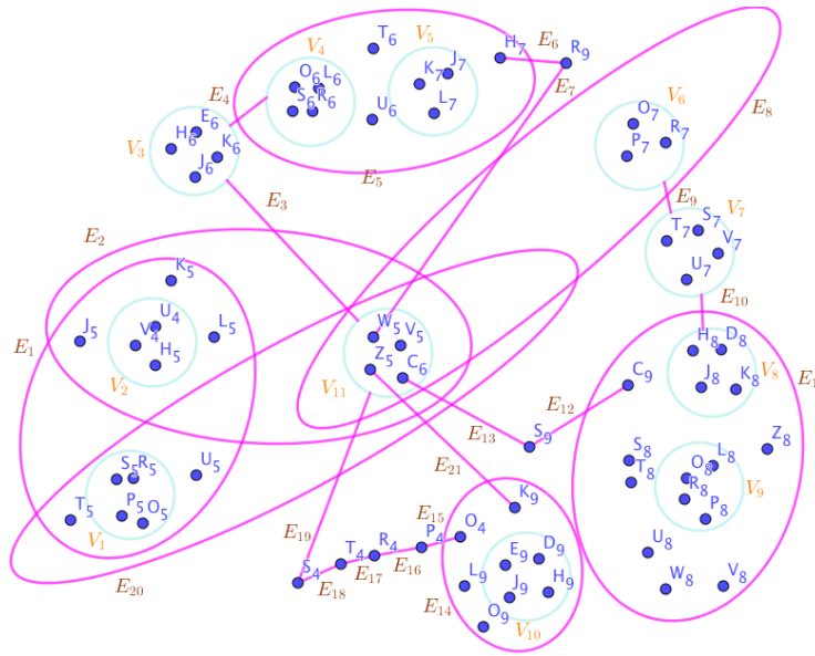
Figure 3. A SuperHyperGraph, is called “SuperHyperFlower”, Associated to the Notions of SuperHyperGirth in the Example (3.2)
