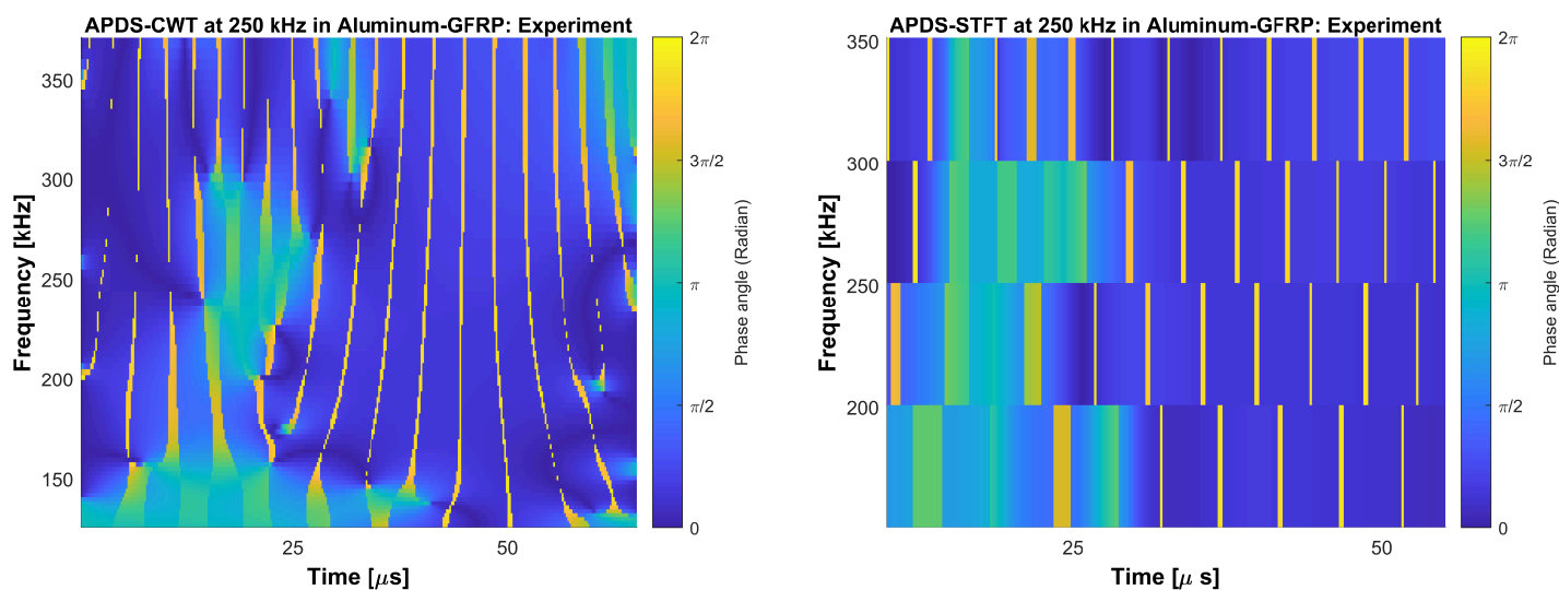
(a) APDS-CWT of the aluminum-GFRP plate at 250 kHz.
