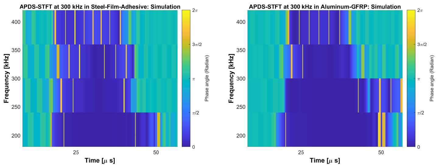
(a) APDS-STFT of the steel-film-adhesive plate at 300 kHz.
