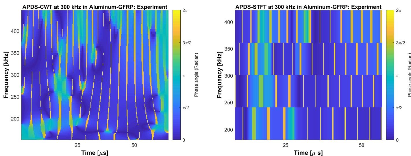
(a) APDS-CWT of the aluminum-GFRP plate at 300 kHz.
