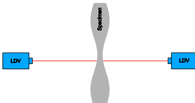
Figure 8. A sketch of the experimental setup illustrates to congruence of the measurement points on the top and bottom surface of a specimen.
