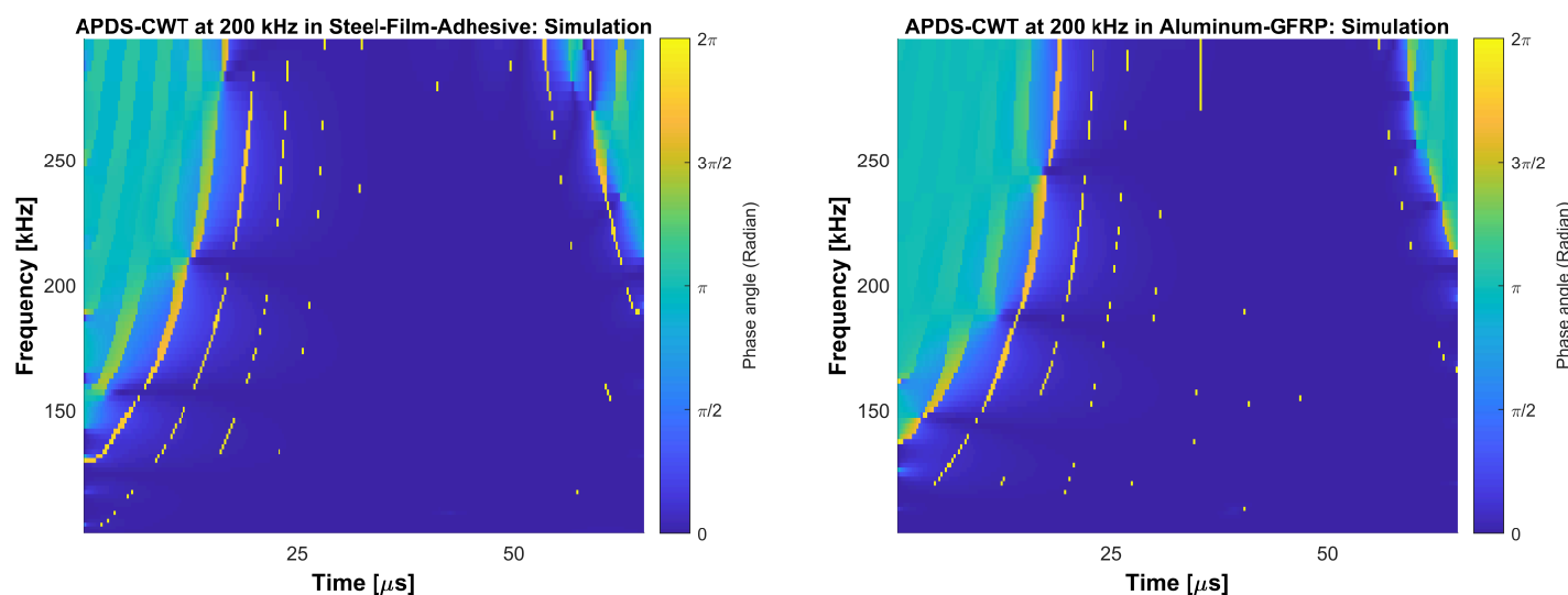
(a) APDS-CWT of the steel-film-adhesive plate at 200 kHz.
