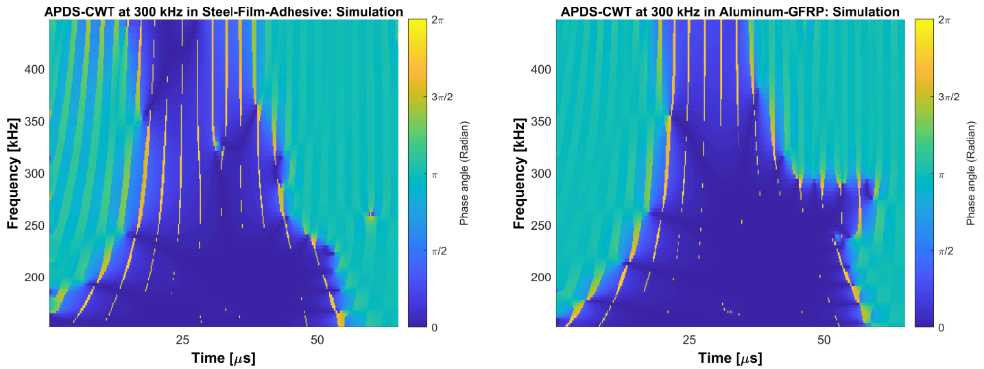
(a) APDS-CWT of the steel-film-adhesive plate at 300 kHz.
