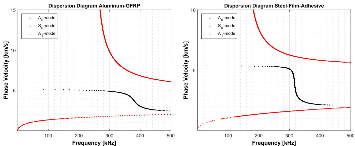
(a) The dispersion diagram for the phase velocities in the aluminum-GFRP laminate indicating a cut-off frequency of higher order modes at approx. 270 kHz.
