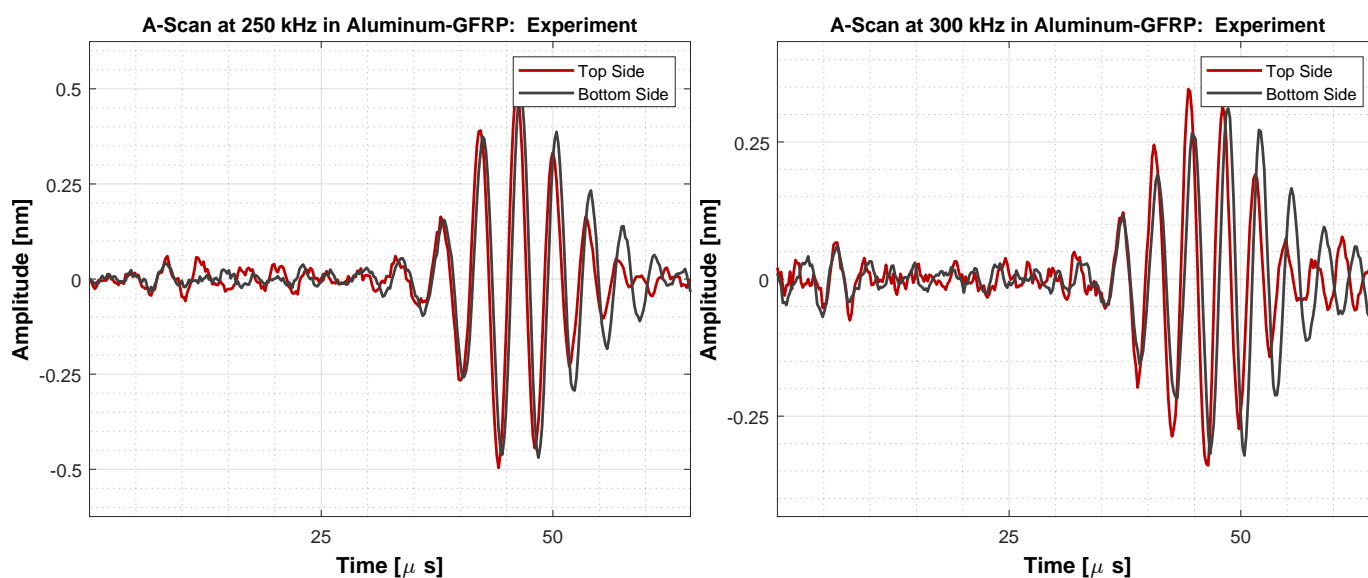
(a) Time signals of the aluminum-GFRP plate at 250 kHz.
