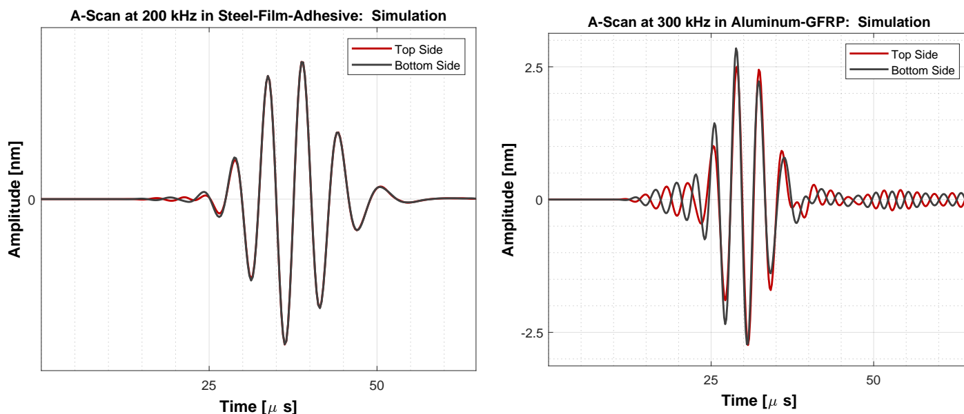
(b) Out-of-plane time signals of the wave propagation in aluminum-GFRP at 300 kHz as example for signal group 2.
