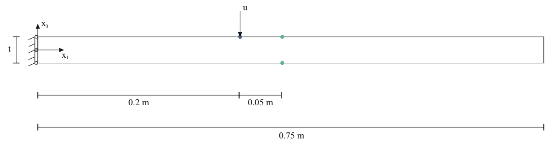
Figure 1. Graphical representation of the numerical model and its boundary conditions as described in Section 3.1.
