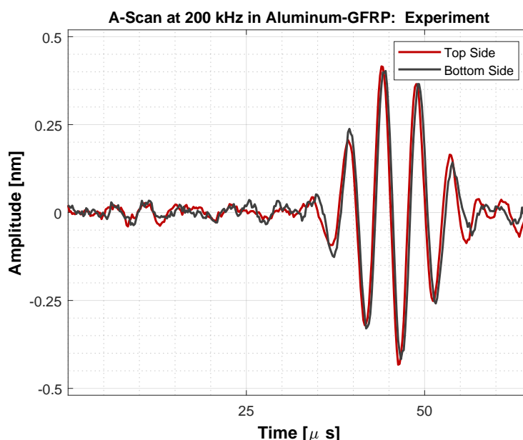
Figure 9. The captured time signals in the aluminum-GFRP plate on the top and bottom surface at 200 kHz.
