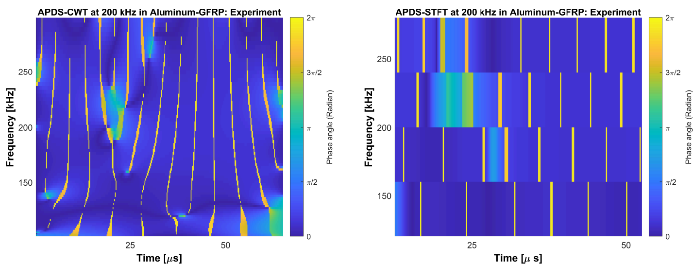
(a) APDS-CWT of the aluminum-GFRP plate at 200 kHz.
