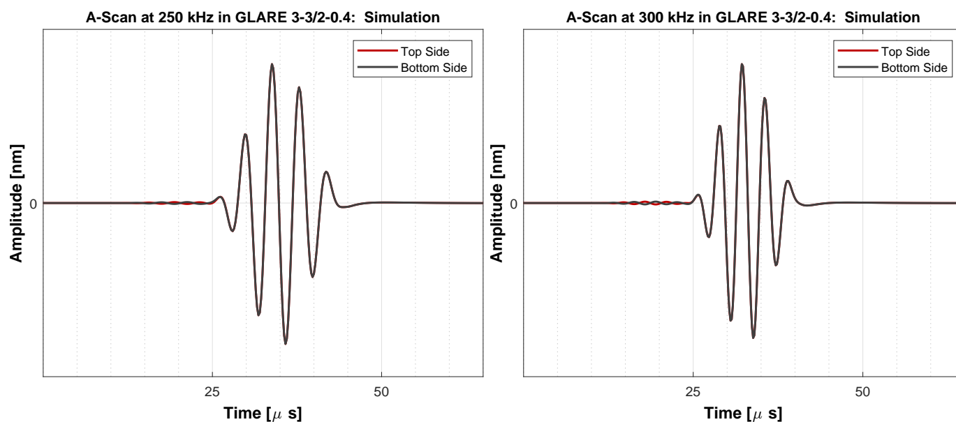
(a) Time signals of the GLARE plate at 250 kHz.
