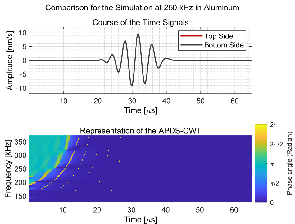
Figure 11. Juxtaposed time signals and the APDS-CWT in Aluminum at 250 kHz. (a) Time-domain: The course of the time signals. (b) Frequency-domain: The APDS-CWT.
