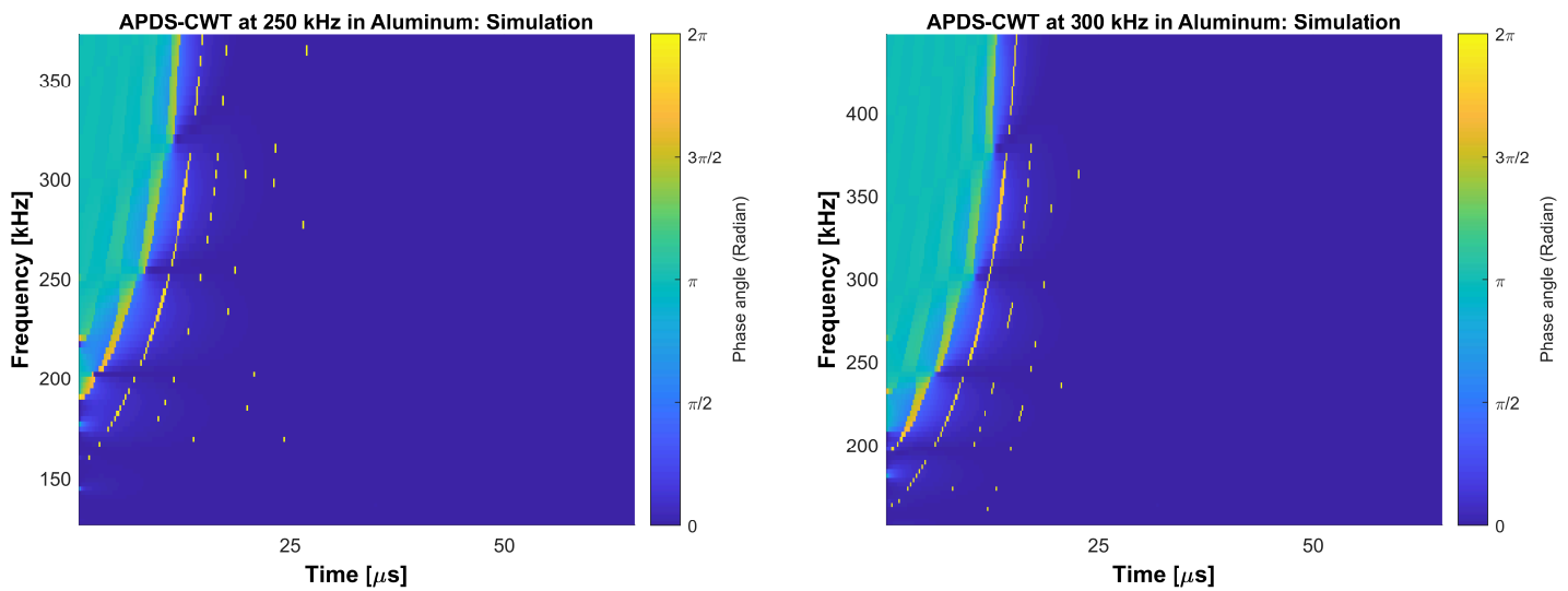
(a) APDS-CWT of the Aluminum plate at 250 kHz.
