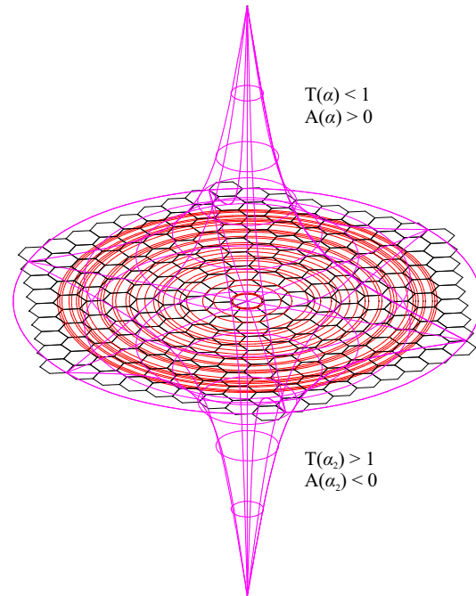
Figure 4. Illustration of the concepts of negative absorptance and excessive transmittance of EMR under normal incidence on MLG.
