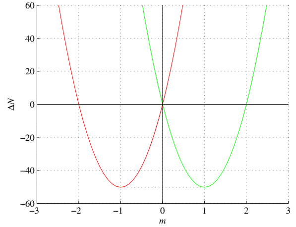
Figure 3. BB information capacity variations \Delta N after absorption (red) or emission (green) of energy m ( k = 2 , \hat{m} = 1 ).
