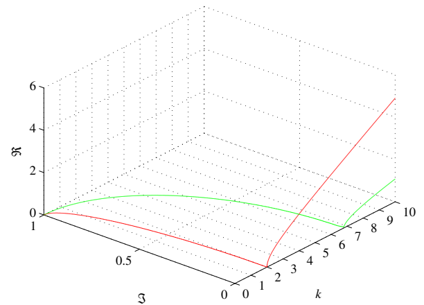
Figure 2. Ratios of imaginary mass M_{iBB} to real mass M_{BB} (green) and real charge q_{BB}/m_P \sqrt{\alpha} to M_{BB} (red) of a BB as a function of the size-to-mass ratio 0 \leq k \leq 10 . The mass M_{iBB} is imaginary for k \lesssim 6.79 . The charge q_{BB} is real for k \geq 2 .
