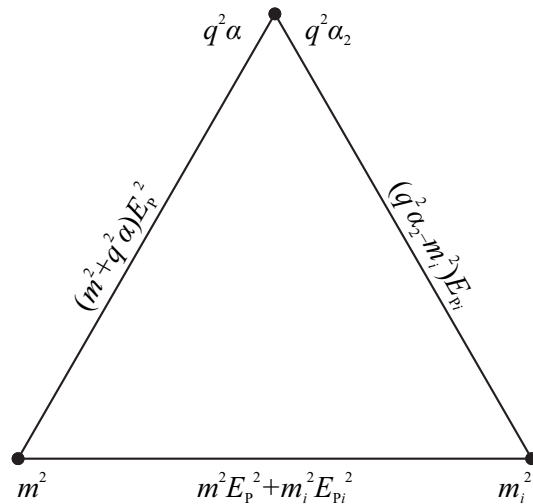
Figure 1. Illustration of three complex energies linking mass m , imaginary mass m_i , and charge q .
