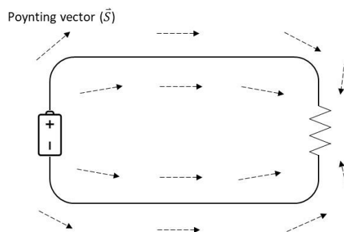
Fig. 1. Energy flow around a DC circuit. The dashed arrows represent Poynting vectors. The concept is explained by Kraus and Carver [4].
