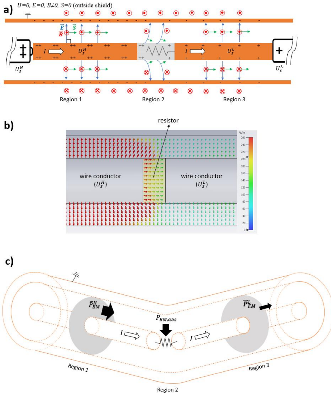
Fig. 4. Electric and magnetic fields around the circuit for Case 2. a): cross-section of the wire along and perpendicular to the wire's longitudinal axis, respectively. The resistor is visualized in grey with the lumped element symbol. The electric potential ( U ), electric field ( \vec{E} ), magnetic field ( \vec{B} ), and Poynting vector ( \vec{S} ) are denoted. r and \theta are radius and angle. b): cross-section view of simulated electric fields, where U_s^H = 3V and U_s^L = 1V are used. The electric field strength, in V/m, is represented by color. Structure dimensions are same as the one in Fig. 3d. c): electromagnetic power flow ( \vec{P}_{EM} ) in Regions 1 and 3 and power absorbed ( P_{EM,abs} ) in the resistor. The thickness of the power flow arrows represents relative power magnitude.
