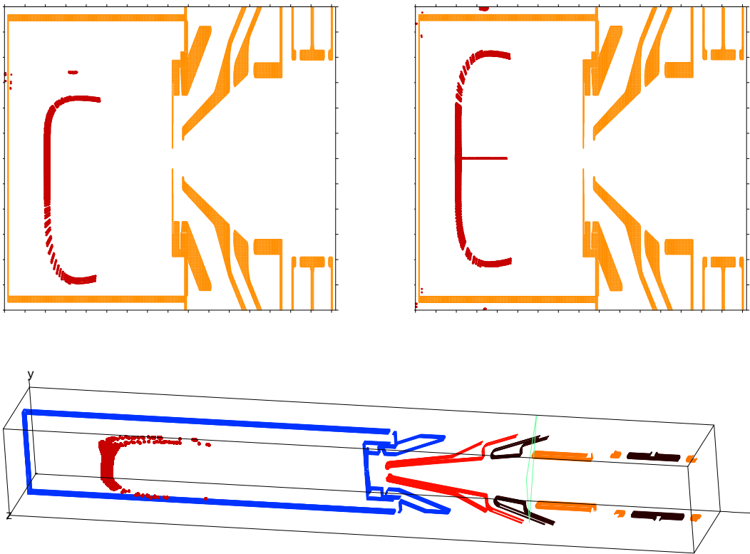
Figure 8. Ions are started in the same B region as in Fig. 7 but here the second intersection of constant B and a field line is used. Top left: vertical projection. Top right: horizontal projection. Bottom: 3D projection. In this figure only the initial coordinates of trajectories are shown.
