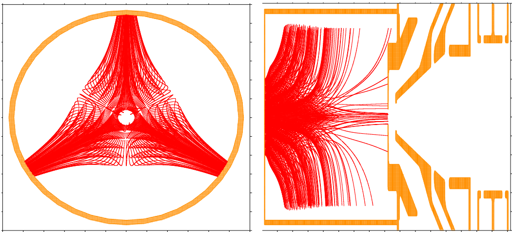
Figure 11. Projection of electron trajectories, started at the disc, biased to -200 V. Left: cut perpendicular to beam direction within the plasma chamber. Right: cut in beam direction. The structure is caused by discretization in radius and azimuth of the electron ‘beam’.
