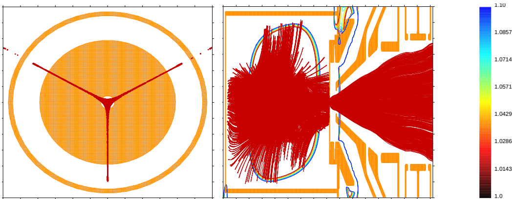
Figure 9. Left: projection of initial positions of trajectories in longitudinal direction at x=0.4 m. Right: trajectories in a transverse projection, at 6 cm with \pm 6 cm projection depth. Lines of constant B from 1.0 T to 1.1 T are shown together with the trajectories.
