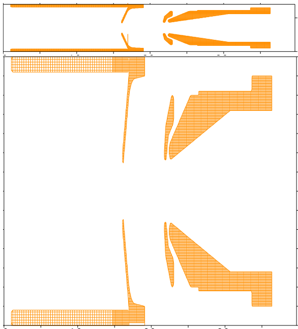
Figure 4. CAPRICE computer model. Top: correct aspect ratio. Bottom: enlarged scale.
