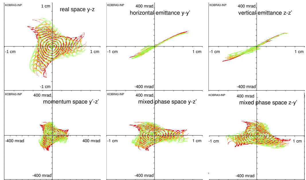
Figure 12. Different projections of the 6D-phase-space behind the extraction electrode ( x=0.45 m in Figure 5). Top row: real space, horizontal and vertical emittance. Bottom row: momentum space, horizontal and vertical mixed phase-spaces (horizontal angle against vertical position and vice versa). Scaling \pm 1 cm, \pm 400 mrad. Green: \text{Ar}^+ , brown \text{Ar}^{2+} and red \text{Ar}^{3+} . Each of these six projections contains 465,688 trajectories.
