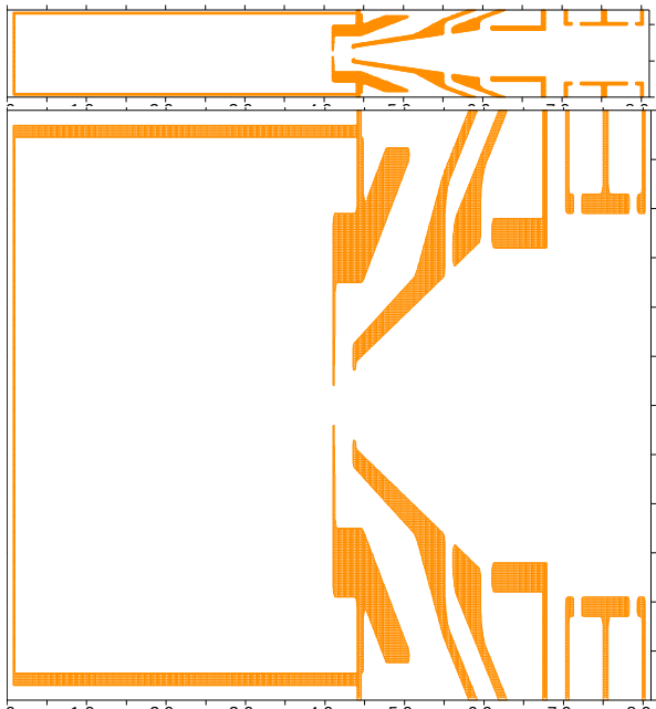
Figure 5. HIISI computer model. Top: correct aspect ratio, bottom: enlarged scale.
