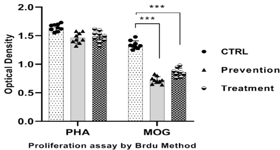
Figure 3. Oral administration of MOG suppresses T-cell proliferation. Splenocytes and lymph nodes were harvested on day 25 post-immunization and cultured in PHA (20 \mu g/mL), as a positive control, or with MOG (20 \mu g/mL) for 72h on 96-well plates. Proliferation responses were tested using a Cell Proliferation ELISA, BrdU (colorimetric) kit (Roche Applied Science, Indianapolis, USA). The proliferation assay was done in triplicates. Data presented as mean optical density \pm SEM. * p <0.05, ** p <0.01, *** p <0.001, when compared with control group. Mice were divided into three groups: 1. Control group (CTRL, n =9); 2. Prevention group with MOG ( n =9); 3. Treatment group with MOG ( n =9).
