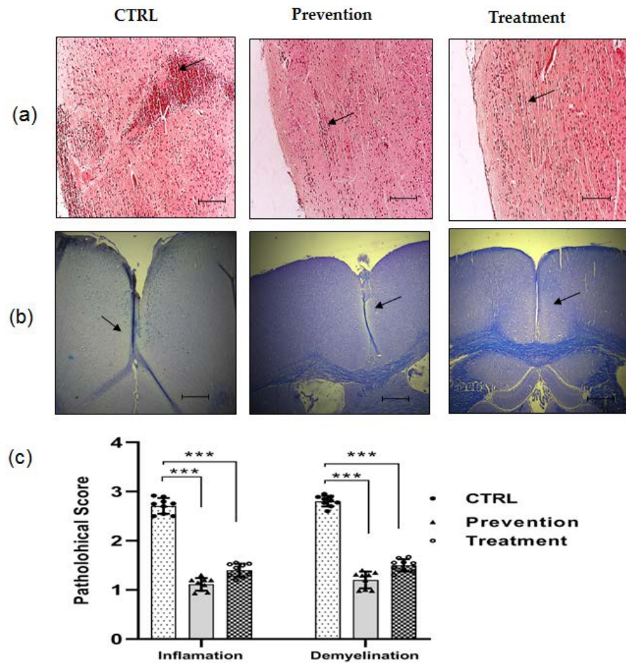
Figure 2. MOG administration ameliorates CNS inflammation and demyelination. Histopathological evaluation of CNS from all the mice was performed. Brain sections from each group were collected on day 25 post-immunization, fixed in paraformaldehyde, and embedded in paraffin. Five \mu\text{m} sections from different regions of the brain from each of the groups were stained with (a) Hematoxylin and eosin, to enumerate infiltrating leukocytes, and (b) Luxol fast blue to assess demyelination. Scale bars: 100 \mu\text{m} . (C) CNS inflammatory foci and infiltrating inflammatory cells were quantified. Pathological scores, including inflammation and demyelination, were analyzed and shown as mean scores of pathological inflammation or demyelination \pm SEM. * p < 0.05 , ** p < 0.01 , *** p < 0.001 , when compared with control group. Mice were divided into three groups: 1. Control group (CTRL, n=9 ); 2. Prevention group with MOG ( n=9 ); 3. Treatment group with MOG ( n=9 ).
