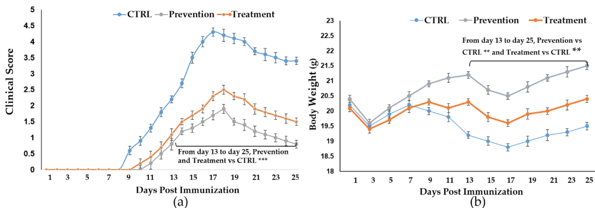
Figure 1. Oral administration of MOG inhibited the development of EAE in C57BL/6 mice. Prevention group received 250 \mu g of MOG 35-55 orally two weeks before EAE induction until 14 days after EAE induction, every day, and treatment group received MOG 35-55 orally after EAE induction until 14 days post-immunization. Mice were monitored for signs of EAE, and the results for all mice, were presented as (a) mean clinical score; and (b) body weight. Results were expressed as mean \pm SEM. * p < 0.05 , ** p < 0.01 , *** p < 0.001 , compared with control group. Mice were divided into three groups: 1. Control group (CTRL, n=9 ); 2. Prevention group with MOG ( n=9 ); 3. Treatment group with MOG ( n=9 ).
