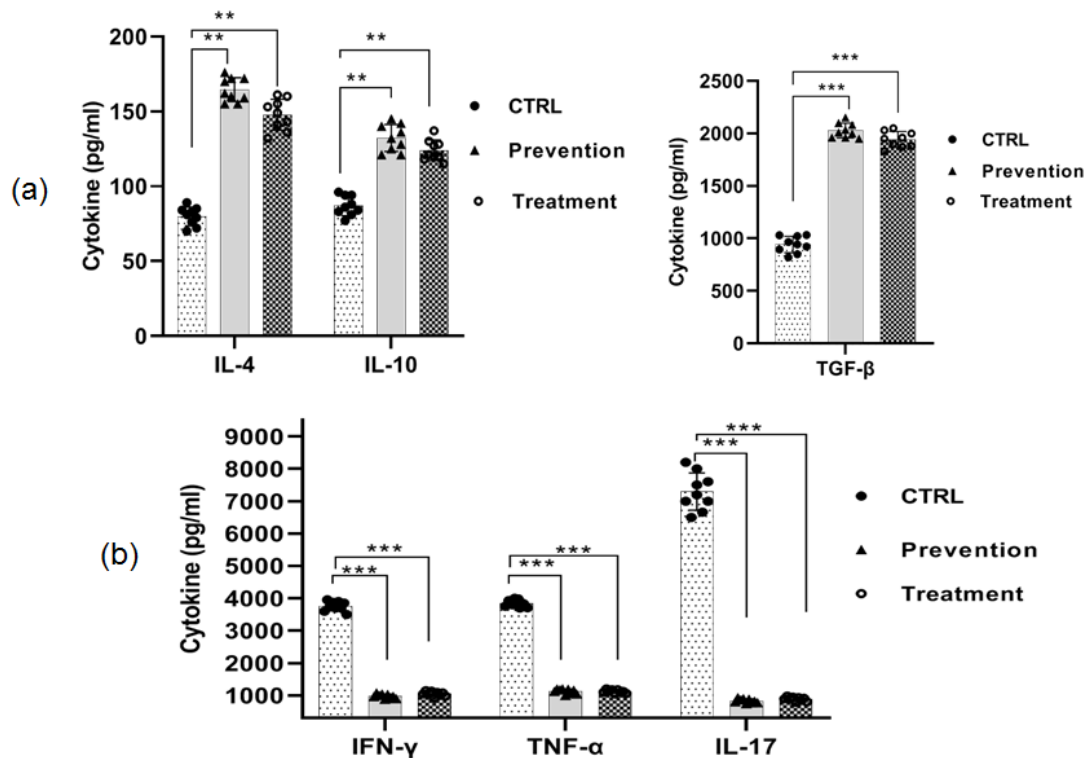
Figure 4. Oral administration of MOG suppressed pro-inflammatory cytokines production and enhanced anti-inflammatory cytokines production in splenocytes and lymph nodes from EAE mice. Splenocytes and lymph nodes from immunized mice from all groups were isolated on day 25 post-immunization and re-stimulated with MOG35–55 (20 \mu g/mL) for 72 h. Cell culture supernatants were collected and indicated cytokine levels were measured by ELISA. Cytokine assays were conducted in duplicate wells. (a) Anti-inflammatory cytokines IL-4, IL-10, and TGF- \beta ; (b) pro-inflammatory cytokines IFN- \gamma , TNF- \alpha , and IL-17 released by splenocytes in culture, \pm SEM. Results from lymph nodes were similar to splenocytes (not shown). * p < 0.05 , ** p < 0.01 , *** p < 0.001 , when compared with control group. Mice were divided into three groups: 1. Control group (CTRL, n=9 ); 2. Prevention group with MOG ( n=9 ); 3. Treatment group with MOG ( n=9 ).
