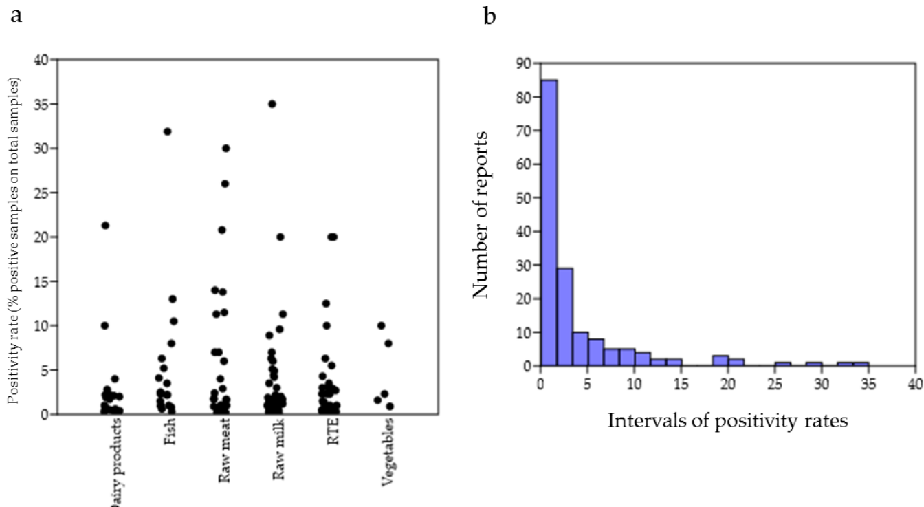
Figure 1. (a) Jitter plot representation of the distribution of the percentages of positive samples per food category. Each circle corresponds to a report. (b) Histogram showing the number of reports falling in different intervals of percentage of L. ivanovii positive samples for all food categories (B). Plots were obtained with the Past Statistical software 4.03 downloadable at https://past.en.lo4d.com/windows [147].
