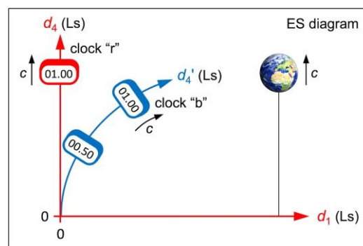
Figure 4. ES diagram of two identical clocks “r” (red) and “b” (blue). Clock “r” and Earth move in the d_4 axis of “r” at the speed c . Clock “b” accelerates in the d_1 axis of “r” toward Earth.
