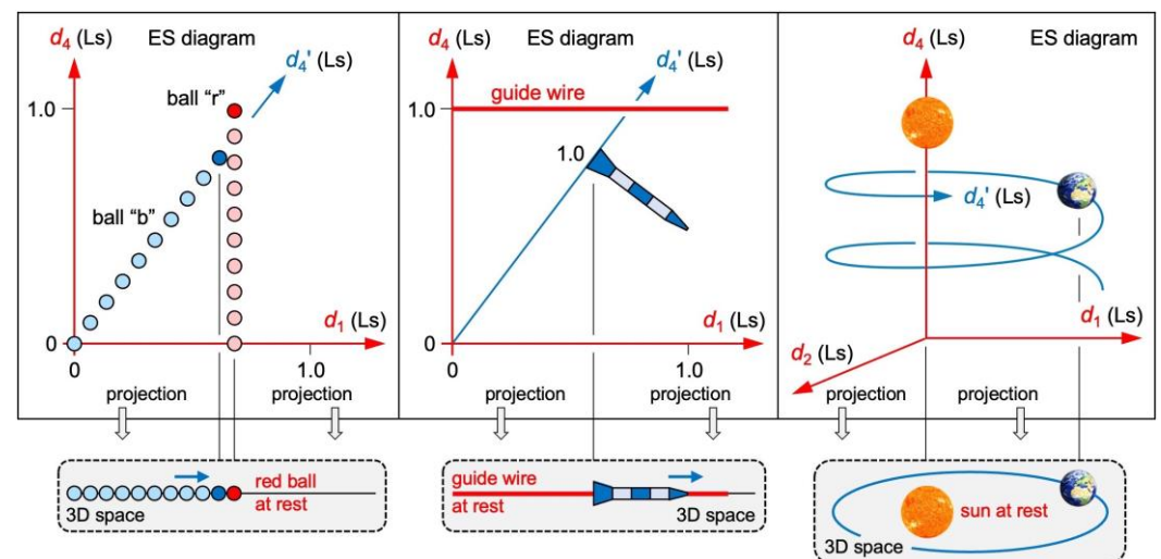
Figure 5. Solving three instructive problems in ER. Each snapshot shows one instant in cosmic time. Left: The blue ball “b” is approaching the red ball “r”. In the projection to the 3D space of the red ball, the balls collide. Center: A rocket moves along a guide wire. In the projection to the 3D space of the guide wire, the wire does not escape from the rocket. Right: Earth orbits the sun. In the projection to the 3D space of the sun, the sun does not escape from Earth.
