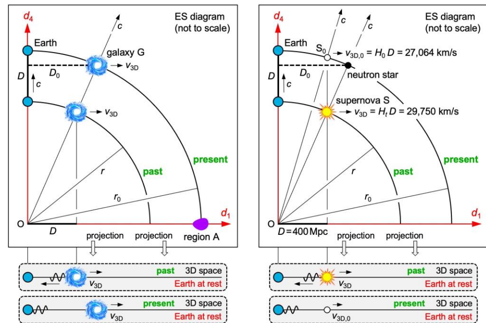
Figure 5. ER-based model of cosmology. The circular arcs are part of an expanding 3D hypersurface. Left: Galaxy G recedes from Earth at the 3D speed v_{3D} . Right: If star S_0 happens to be at the same distance from Earth today as the supernova of star S in the past, S_0 recedes more slowly than S .
