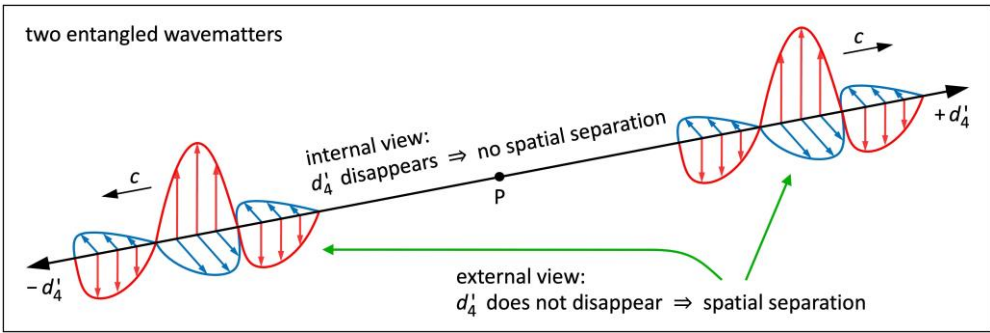
Figure 8. Two wavematters moving in \pm d_4' at the speed c are spatially separated for an observer moving in any direction other than \pm d_4' (external view). For each wavematter (internal view), the d_4' axis disappears. From the internal view, the twins have never been separated spatially.
