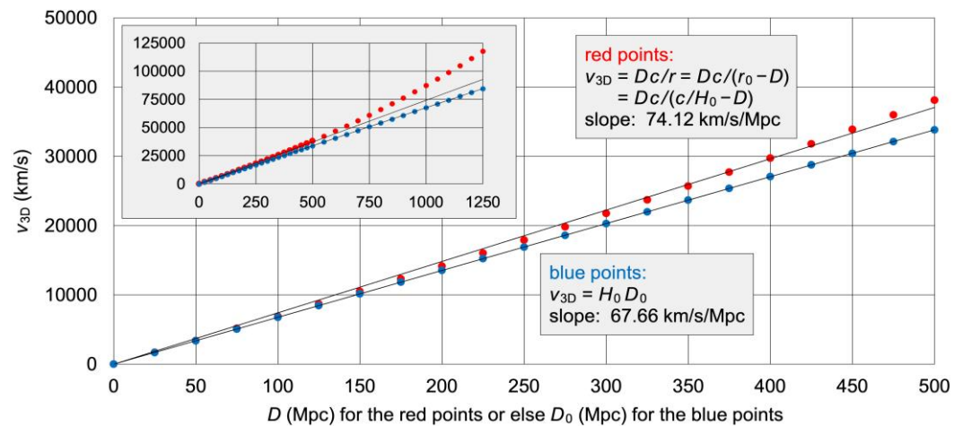
Figure 6. Hubble diagram of simulated supernovae at distances up to 1250 Mpc. The horizontal axis is D for the red points or else D_0 for the blue points. Eq. (19) does not yield a straight line because H_t is not a constant. Only Eq. (20) yields a straight line.
