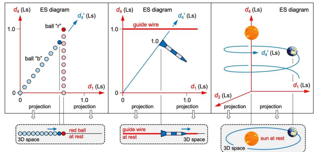
Figure 4. Solving three instructive problems in ER. Each snapshot shows one instant in cosmic time. Left: The blue ball "b" is approaching the red ball "r". In the projection, the balls collide. Center: A rocket moves along a guide wire. In the projection, the wire does not escape from the rocket. Right: Earth orbits the sun. In the projection, the sun does not escape from Earth's orbit.
