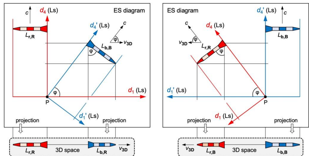
Fig. 2 ES diagrams and 3D projections for two rockets “r” (red) and “b” (blue). Top: Both rockets move in different 4D directions at the speed c . Bottom left: Projection to the 3D space of R. Rocket “b” contracts to L_{b,R} . Bottom right: Projection to the 3D space of B. Rocket “r” contracts to L_{r,B}
