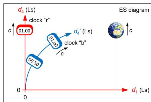
Fig. 3 ES diagram for two clocks "r" (red) and "b" (blue). Clock "r" and Earth move in the d_4 axis of "r" at the speed c . Clock "b" accelerates in the d_1 axis of "r" toward Earth
