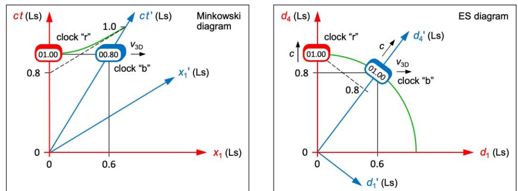
Fig. 1 Minkowski diagram and ES diagram for two clocks “r” (red) and “b” (blue). Left: In SR, “b” is slow with respect to “r” in t' . Coordinate time is relative (“b” is not at the same positions in ct and ct' ). Right: In ER, “b” is slow with respect to “r” in d_4 . Cosmic time is absolute (“r” is in d_4 at the same position as “b” in d_4' ). Only the ES diagram is rotationally symmetric
