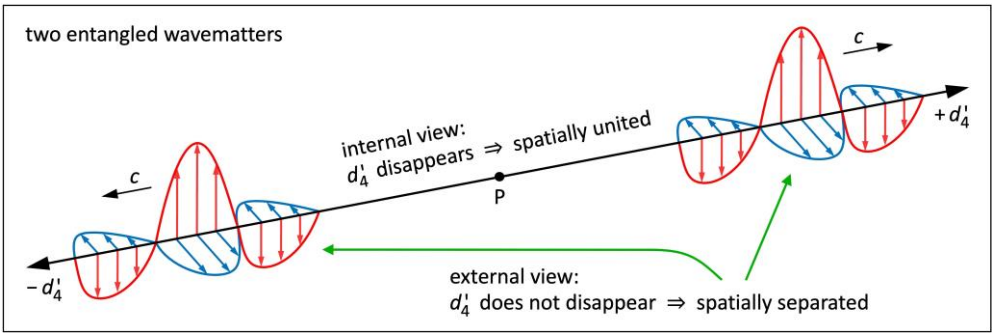
Fig. 8 Two wavematters moving in \pm d'_4 are spatially separated objects for an observer who moves in any direction other than \pm d'_4 (external view). For each wavematter (internal view), the \pm d'_4 axis disappears. In their common proper space, both wavematters remain spatially united
