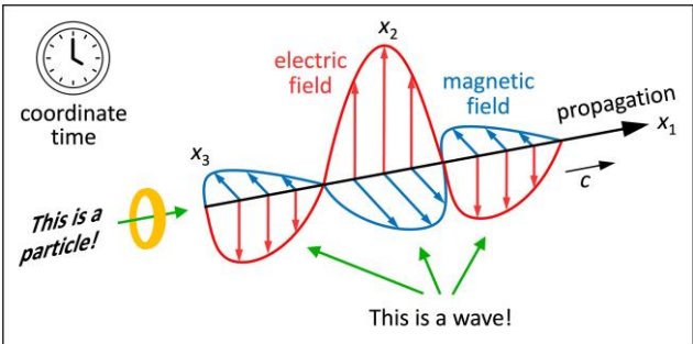
Fig. 7 Illustration of a wavematter. In an observer’s reality (external view, coordinate spacetime!), a wavematter may appear as a wave packet or as a particle. As a wave, it propagates and oscillates as a function of coordinate time. In its own reality (internal view), the axis of the wavematter’s 4D motion disappears because of length contraction at the speed c . It deems itself particle at rest
