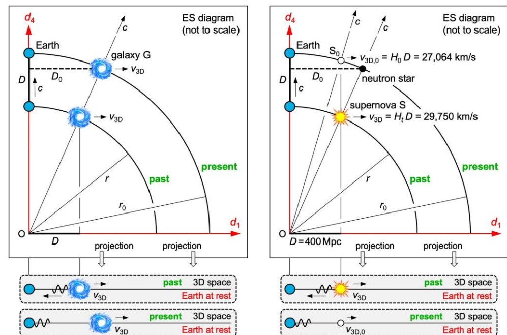
Fig. 5 Solving the mysteries 5.6, 5.7, 5.10, and 5.11. The circular arcs are part of an expanding 3D hypersurface. Left: The galaxy G recedes from Earth at the 3D speed v_{3D} . Right: The supernova of a star S occurred at a distance of D = 400 Mpc from Earth. If another star S_0 happens to be at the same distance D today, S_0 recedes more slowly from Earth than S
