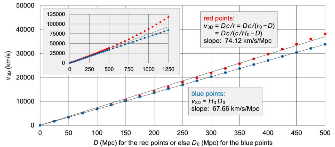
Fig. 6 Hubble diagram for simulated supernovae at distances up to 1250 Mpc. The horizontal axis is D or else D_0 . Only Eq. (20) yields a straight line. Eq. (19) does not because H_t is not a constant
