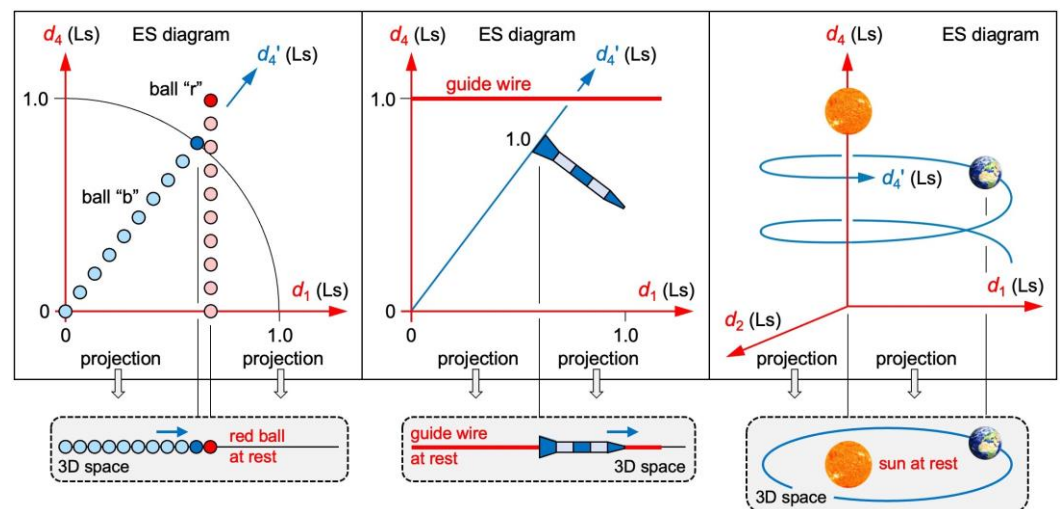
Fig. 4 Solving three instructive problems. Each snapshot shows one instant in cosmic time, which serves as the parameter in ER. The left ES diagram shows ten snapshots at once. Left: The blue ball “b” is hit toward the red ball “r”. In the projection, the two balls collide. Center: Some rocket moves along a guide wire. In the projection, the wire does not escape from the rocket. Right: Earth orbits the sun. In the projection, the sun does not escape from the orbital plane
