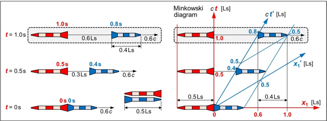
Figure 4. Two identical rockets in MS. Left: Both rockets have a length at rest of 0.5\text{ Ls} . Their relative speed is 0.6\text{ c} . At t = 0.5\text{ s} and t = 1.0\text{ s} , clocks inside the blue rocket display less time because of time dilation. The blue rocket is shorter because of length contraction. Right: A Minkowski diagram transfers the geometry from the left into a time–distance graph. In this diagram at ct = 1.0\text{ Ls} , clocks in the rear end and tip of the blue rocket display different times ( 0.8 and 0.5 printed in blue). This is not in line with experimental physics as observers in the blue rocket will synchronize their clocks.
