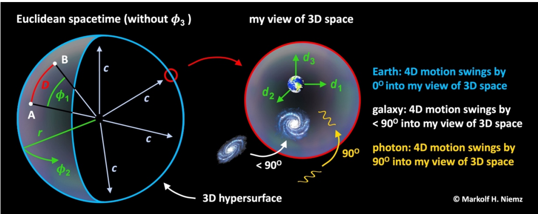
Figure 7. Model of cosmology based on ES (not to scale). Artwork illustrating how a hypersurface is expanding in ES. Left: Non-observable ES in hyperspherical coordinates (\phi_1, \phi_2, \phi_3, r) . \phi_3 can’t be displayed. Hubble’s law is derived from the geometry of the hypersurface. Right: My view of 3D space in Cartesian coordinates (d_1, d_2, d_3) . d_4 disappears because of length contraction. The right red circle doesn’t only show an enlargement of the left red circle, but also another set of coordinates.
