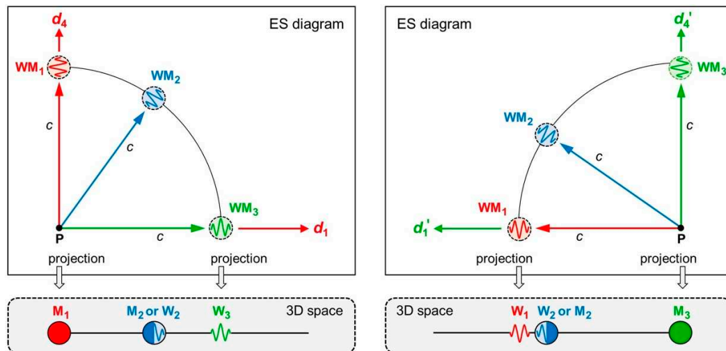
Figure 7. ES diagrams and 3D projections for three wavematters. Top left: ES in coordinates where WM_1 moves in d_4 . Top right: ES in coordinates where WM_3 moves in d'_4 . Bottom left: Projection to WM_1 ’s 3D space. WM_1 deems itself matter at rest ( M_1 ) and WM_3 wave ( W_3 ). Bottom right: Projection to WM_3 ’s 3D space. WM_3 deems itself matter at rest ( M_3 ) and WM_1 wave ( W_1 )
