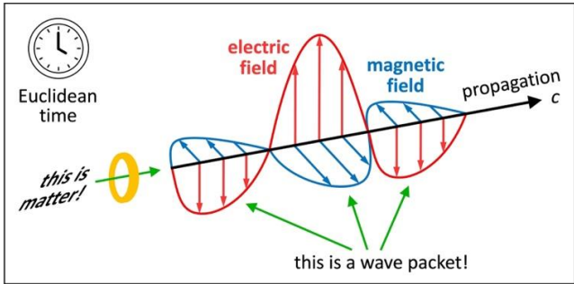
Fig. 7 Concept of wavematter. Artwork illustrating how one object can be deemed wave or matter. Wavematter comes in four orthogonal dimensions: propagation, electric field, magnetic field, and Euclidean time. Each wavematter deems itself matter at rest (internal or in-flight view). If it is observed by some other wavematter (external view), it is deemed wave
