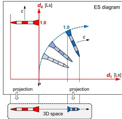
Fig. 3 ES diagram and 3D projection for two identical rockets. Top: In the ES diagram, the red rocket moves in the steady axis d_4 . The blue rocket accelerates in the axis d_1 . Its speed u_1 increases at the expense of its speed u_4 . Bottom: Projection to the 3D space of R. The red rocket is “at rest”. The blue rocket accelerates against the red rocket
