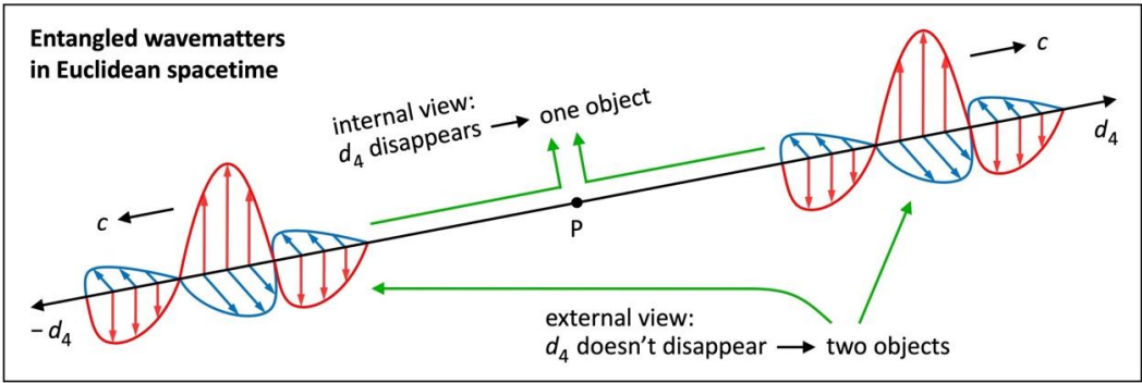
Fig. 9 Quantum entanglement in ES. Artwork illustrating internal view and external view. For each displayed wavematter, the axis d_4 disappears because of length contraction. It deems its twin and itself one object (internal view). For a third wavematter that is moving in a direction other than d_4 , the axis d_4 doesn't disappear. It deems the displayed wavematters two objects (external view)
