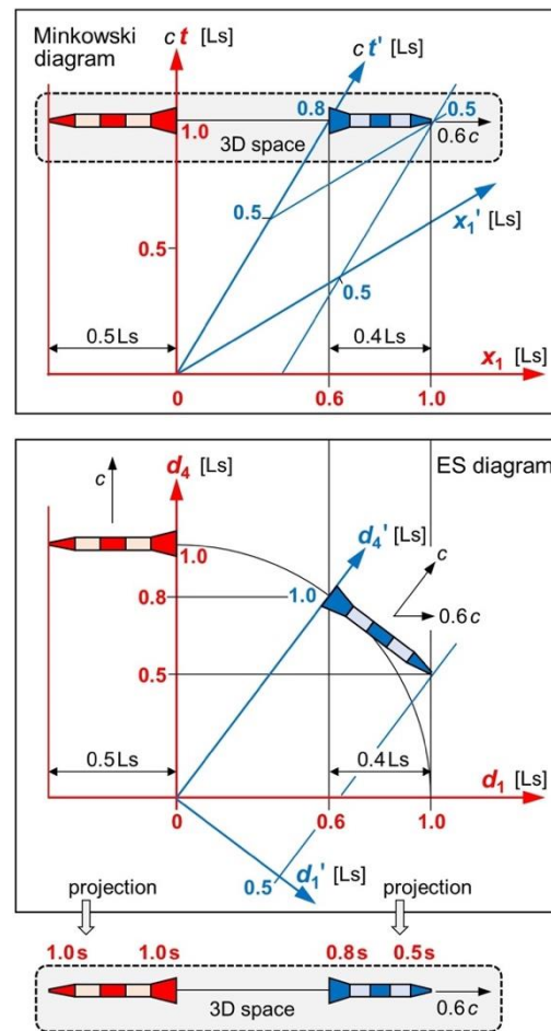
Fig. 1 Minkowski diagram, ES diagram, and 3D projection for two identical rockets. Top: The Minkowski diagram depicts the reality of just one observer (here: of R who synchronizes all clocks inside both rockets). Our diagram doesn't depict the reality of B who would also synchronize these clocks. Center: The ES diagram can be projected to either reality. Bottom: Projection to the 3D space of R
