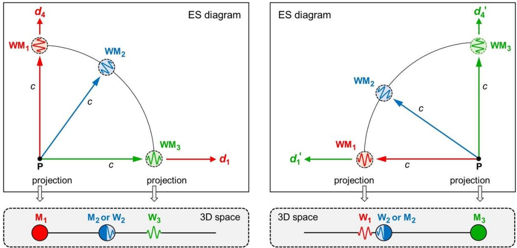
Fig. 8 ES diagrams and 3D projections for three wavematters. Top left: ES in coordinates where WM_1 moves in d_4 . Top right: ES in coordinates where WM_3 moves in d'_4 . Bottom left: Projection to WM_1 ’s 3D space. WM_1 deems itself matter at rest ( M_1 ) and WM_3 wave ( W_3 ). Bottom right: Projection to WM_3 ’s 3D space. WM_3 deems itself matter at rest ( M_3 ) and WM_1 wave ( W_1 )
