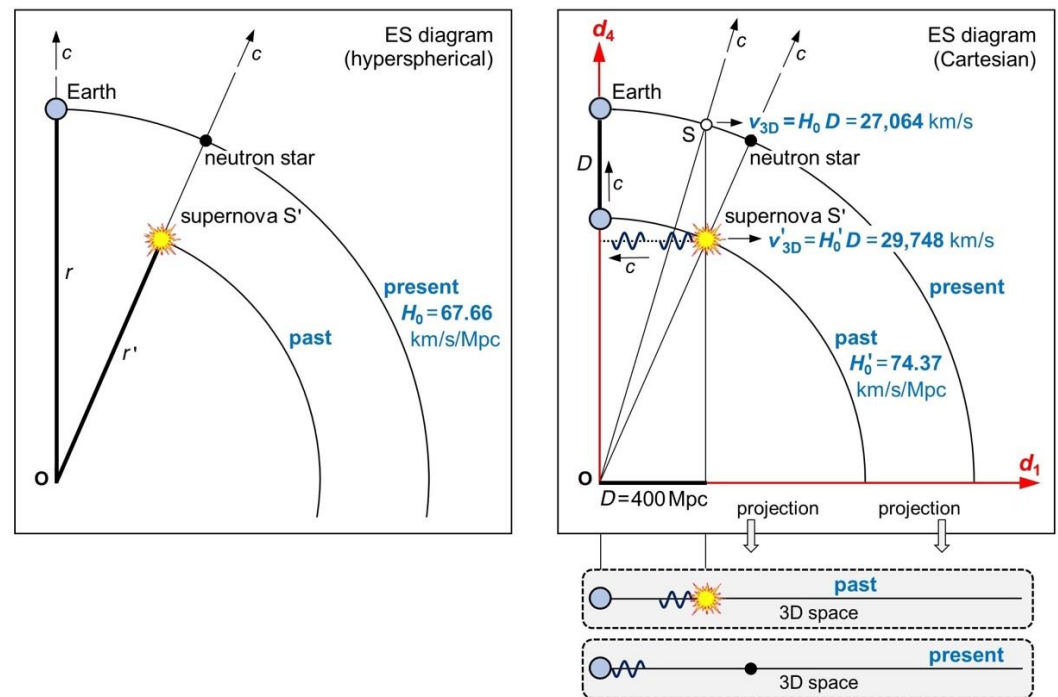
Fig. 6 ES diagrams for team B’s calculation of the Hubble constant. The location of the Big Bang serves as the origin O. Left: We assume that 67.66 km/s/Mpc would be today’s value of the Hubble constant H_0 (present). A supernova S' occurred in the past when the radius r' of the hypersurface was smaller than today’s radius r . Right: Team B observes S' and measures a distance of 400 Mpc. Since the occurrence of S' , Earth has also moved 400 Mpc, but in the axis d_4 . Team B calculates a Hubble constant H'_0 of the past (74.37 km/s/Mpc). A supernova S occurring today (same distance, small white circle) recedes slower (27,064 km/s) than a supernova S' in the past (29,748 km/s)
