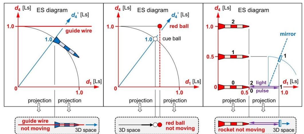
Fig. 4 Graphical solutions to three geometric paradoxes. Left: A rocket moves along a guide wire. In 3D space, the guide wire remains within the rocket. Center: A cue ball is hit to collide with the red ball. In 3D space, the cue ball collides with the red ball. Right: An observer in a rocket’s tip tries to detect the reflection of a light pulse. Between two snapshots (0–1 or 1–2), rocket, mirror, and light pulse move 0.5 Ls in ES. In 3D space, the light pulse is reflected back to the observer
