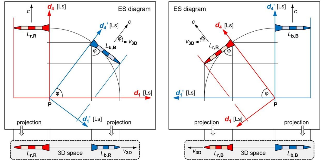
Fig. 2 ES diagrams and 3D projections for two identical rockets. All axes are in Ls (light seconds). Top left and top right: In the ES diagrams, both rockets are moving at the speed c , but in different directions. Bottom left: Projection to the 3D space of R. The relative speed is v_{3D} . The blue rocket contracts to L_{b,R} . Bottom right: Projection to the 3D space of B. The red rocket contracts to L_{r,B} .
