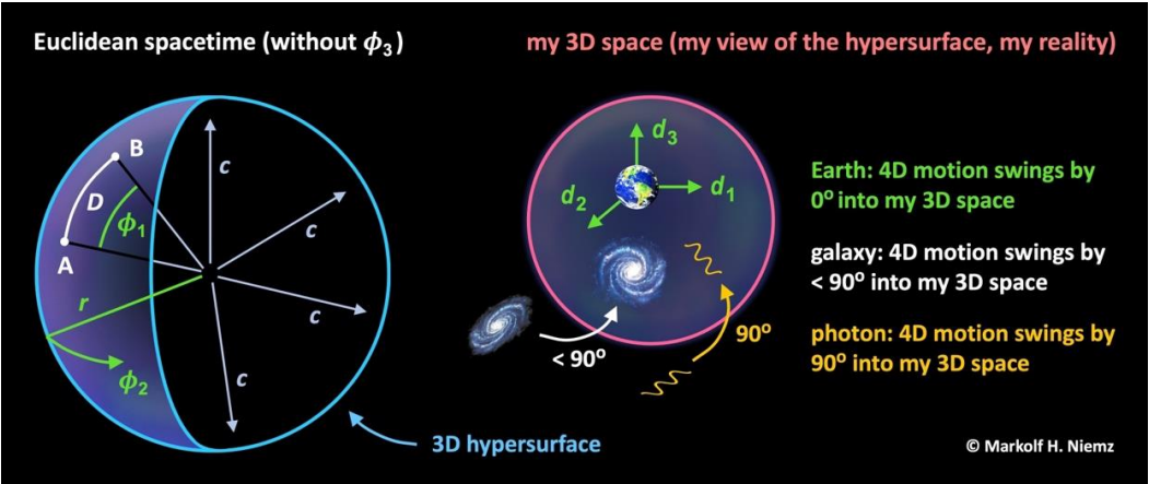
Fig. 5 Model of cosmology based on ER (not to scale). Artwork illustrating how a 3D hypersurface is expanding in ES. Left: Non-observable ES in hyperspherical coordinates ( \phi_1, \phi_2, \phi_3, r ). The angle \phi_3 can’t be displayed here. Hubble’s law is derived from the geometry of the hypersurface. Right: My 3D space in Cartesian coordinates ( d_1, d_2, d_3 ), which is my view of the hypersurface and my reality. The axis d_4 (related to time) disappears because of length contraction
