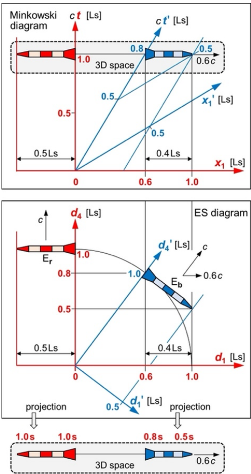
Figure 6. Comparing a Minkowski diagram with an ES diagram. Top: A Minkowski diagram can't display the time of the blue rocket correctly in both the red and the blue frame. In the blue frame, clocks inside the blue rocket display different times. Center: In an ES diagram, no frame is prioritized. The time of the blue rocket is displayed correctly in both frames. Bottom: R's view of 3D space.
