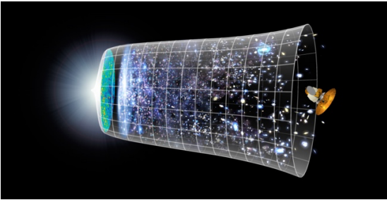
Figure 1. Timeline of the universe according to NASA/WMAP. Artwork illustrating the expansion of space over an assumed 13.8 billion years. Time and space are depicted by the horizontal and vertical extent of the grid, respectively. The universe is supposed to have started in a Big Bang (left). Space is supposed to have undergone different stages of expansion, while time has been running uniformly. Credit: NASA/WMAP.
