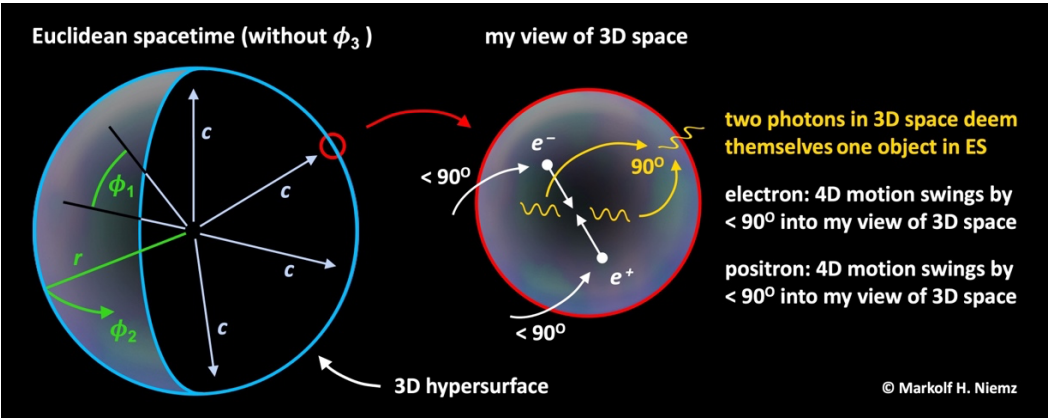
Figure 12. Annihilation process in ES. Artwork illustrating how an electron and a positron convert into two gamma photons. Left: Non-observable ES in hyperspherical coordinates. Right: My view of 3D space in Cartesian coordinates. The two entangled photons deem themselves one object in ES.
