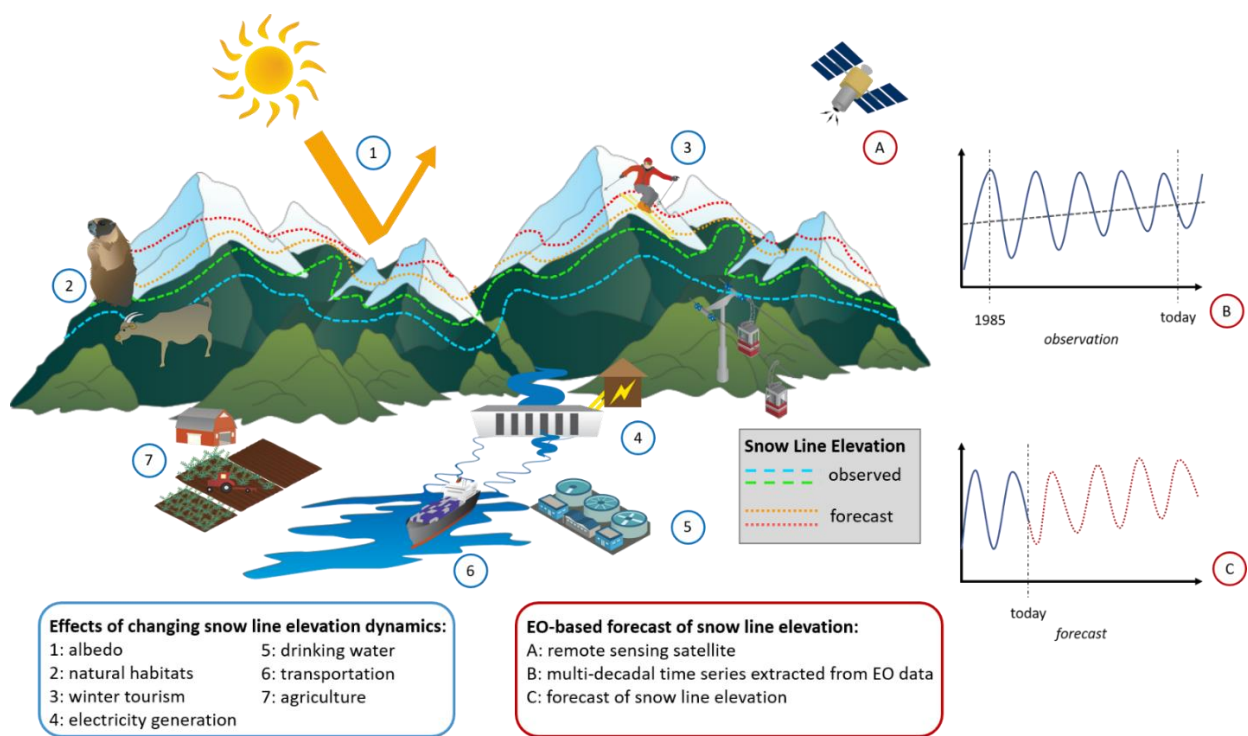
Figure 1. Environmental, societal and economic effects of snow line elevation (SLE) dynamics in mountainous regions. Multi-decadal time series of SLE dynamics observed from remote sensing satellites can be used to forecast future SLE. The forecasts can be used by stakeholders and policy and decision makers to adapt to future SLE dynamics caused by climate change. Several graphics modified courtesy of the Integration and Application Network, University of Maryland Center for Environmental Science ( ian.umces.edu/symbols/ ).
