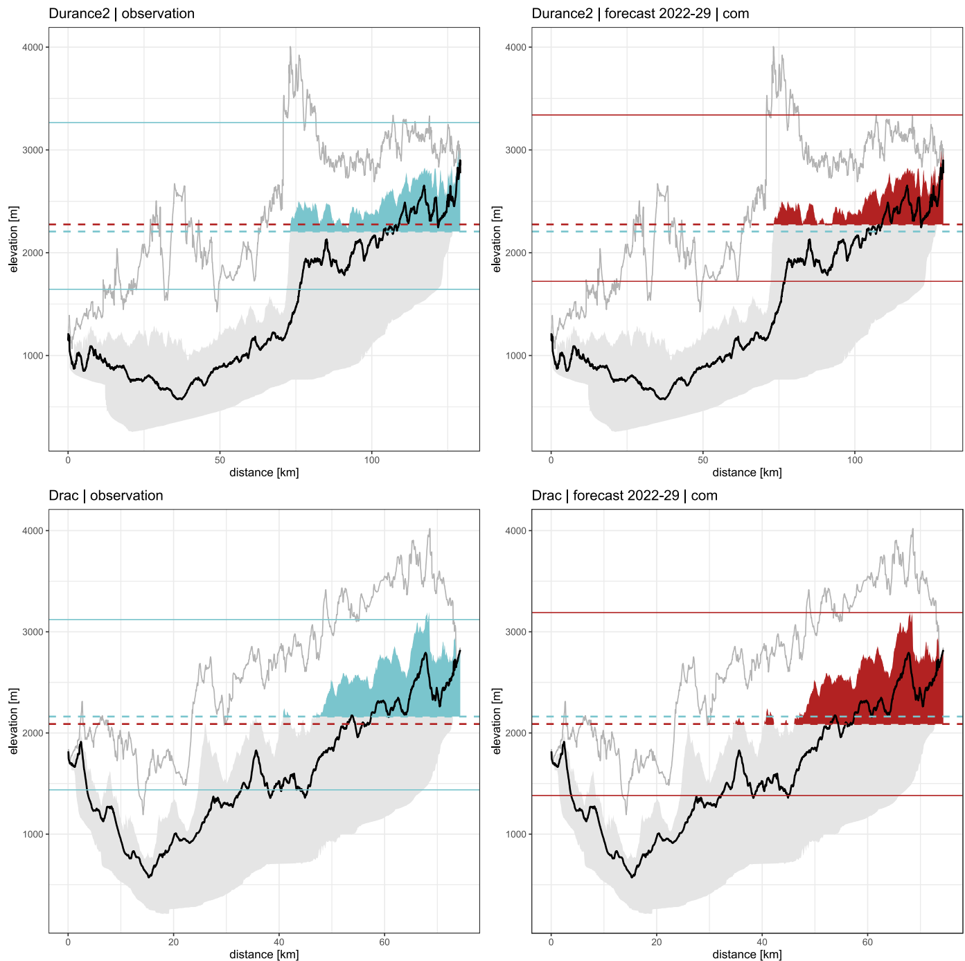
Figure 15. West-to-East swath profiles of the elevation distribution in selected catchments and location of the observed (left, blue) and forecast (right, red) SLE therein. For each North-South transect perpendicular to the swath the maximum (grey line) and median (black line) elevation are given, as well as the elevation range in which 80% of the DEM pixels are located (grey area). Colored lines indicate the median (dashed) and 20 th and 80 th percentile (solid) of the SLE. Areas within the 80 th elevation percentile that are covered in snow more than 50% of the time (i.e. above the SLE median) are highlighted in color.
