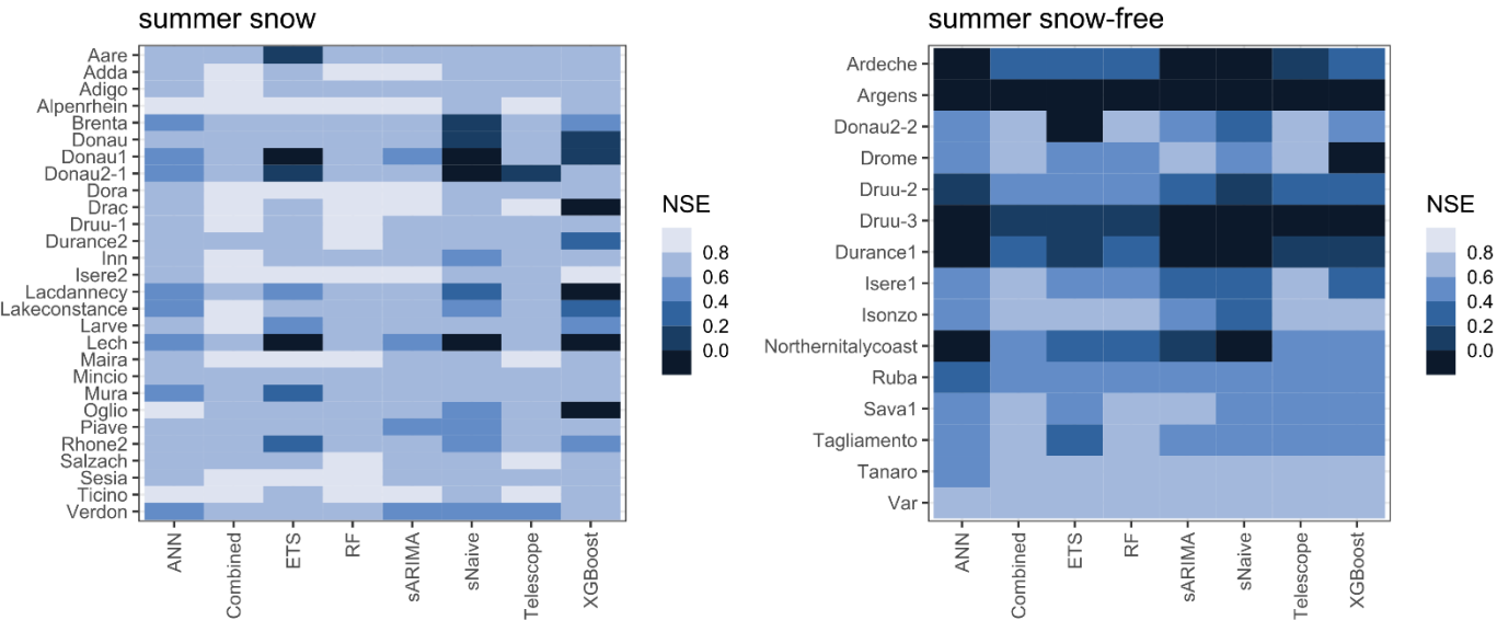
Figure 7. Nash-Sutcliffe efficiency (NSE) of the evaluated forecasting approaches in catchments where the SLE is not maxed-out (left) and where it is maxed-out (right) in the summer months. Lighter colors indicate better performance. An NSE of 1 is a perfect forecast, while an NSE < 0 indicates that the mean of all observations would yield a better forecast than the model.
