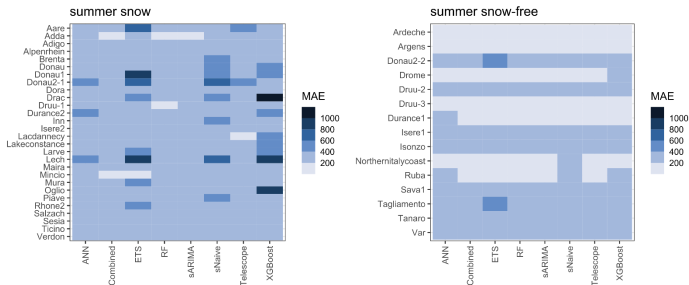
Figure 9. Mean Absolute Error (MAE) of the evaluated forecasting approaches in catchments where the SLE is not maxed-out (left) and where it is maxed out (right) in the summer months. Lighter colors indicate better performance. The MAE can be interpreted as the mean absolute deviation of the predicted data from the observations in Meters.
