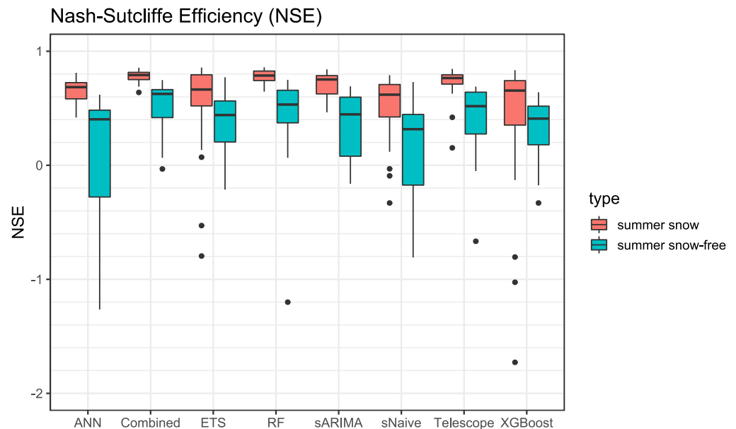
Figure 8. Nash-Sutcliffe efficiency (NSE) of the evaluated forecasting approaches across all catchments. A major negative outlier of XGBoost in one summer snow-free catchment ( NSE \approx -4 ) is not displayed. An NSE of 1 is a perfect forecast, while an NSE < 0 indicates, that the mean of all observations would yield a better forecast than the model.
