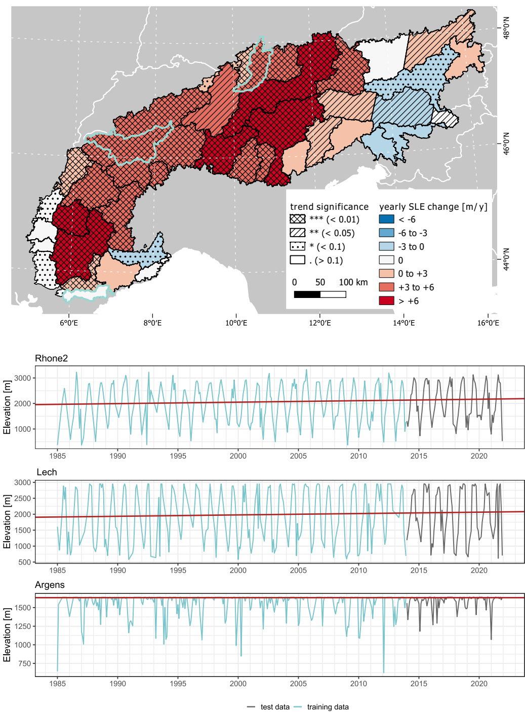
Figure 6. Map showing the calculated long term SLE change trends [m/y] for all analyzed Alpine catchments (above). Three examples of monthly SLE time series from 1985 from the catchments of the rivers Rhone, Lech, and Argens (below). The red line shows the long-term linear trend calculated over the entire time series. The sample catchments are highlighted in the map.
