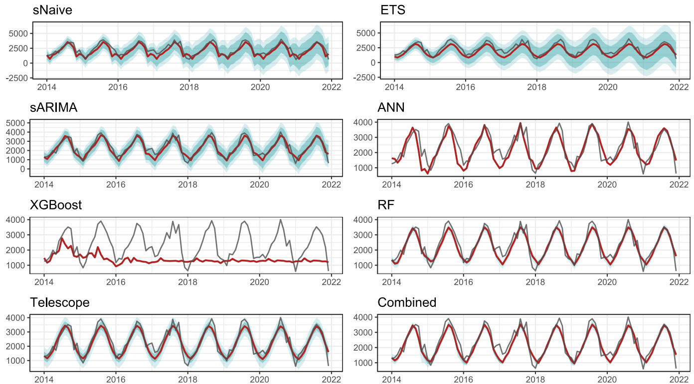
Figure 11. Qualitative comparison of observed (gray) and forecast (red) SLE of the Drac catchment for the time interval 2014-2021. Where applicable, the 80% and 95% confidence interval (blue shades) is provided. The Combined forecast is calculated from ETS, sARIMA, ANN, RF, and Telescope. The weak performance of XGBoost may be a result of the high variance in the input SLE time series.
