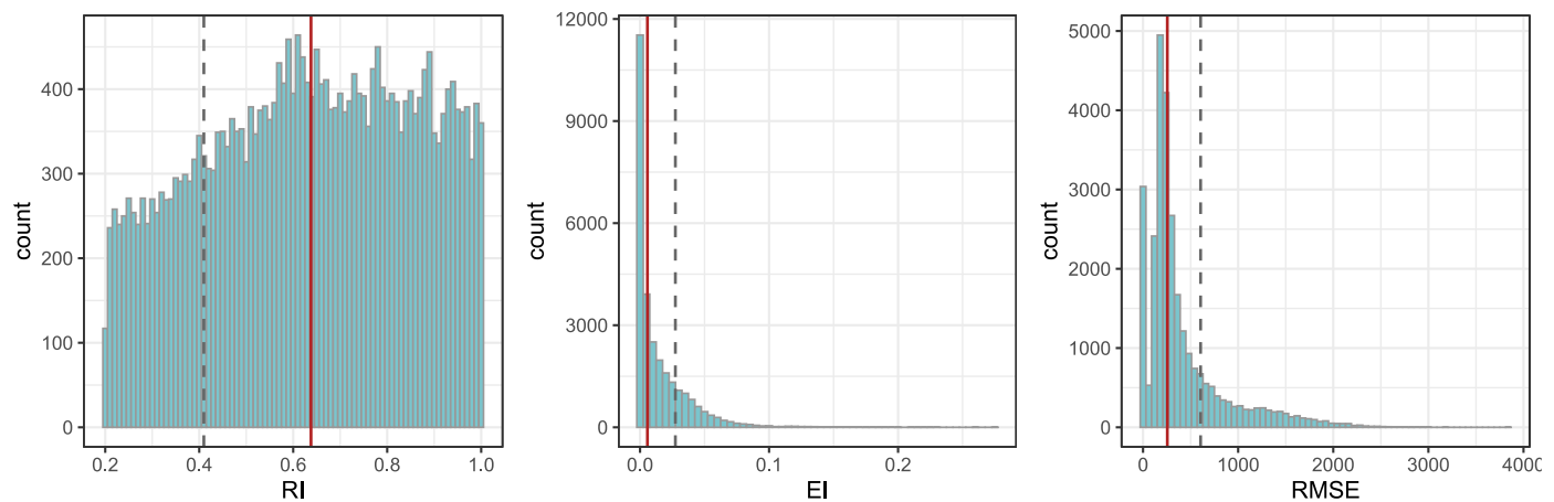
Figure 5. Representative Index (RI), Error Index (EI) and Root Mean Square Error (RMSE) of all derived SLE observations. The red vertical line marks the median value, the dashed line the 20 th (RI) and 80 th (EI, RMSE) percentiles, respectively. RI_{\text{median}} = 0.64 , RI_{20\text{th}} = 0.41 , EI_{\text{median}} = 0.006 , EI_{80\text{th}} = 0.027 , RMSE_{\text{median}} = 255 , RMSE_{80\text{th}} = 605 .
