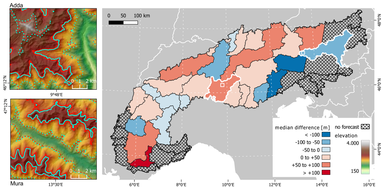
Figure 14. Difference of the medians of the observed time series (1985-2021) and the forecast time series (2002-2029) for each Alpine catchment (map on the right). Positive values indicate that the median SLE in the future is higher than in the observed past. Forecasts are only conducted in catchments without a maxed-out summer SLE. The forecasts were generated using the Combined forecast approach. The panels on the left show two examples of the observed (blue) and forecast (red) SLE in the catchments Adda and Mura. Solid lines indicate the location of the median, the dashed lines of the 20 th and 80 th percentile which correspond to the winter and summer SLE, respectively. Catchments and extents of the details are highlighted in the map.
