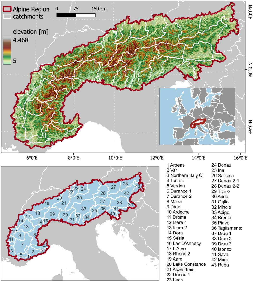
Figure 2. Topography and location of the hydrological catchments in the European Alps. Alpine region delimited by the Alpine convention [30], catchment boundaries according to the HydroSHEDS dataset. Background shows the Copernicus DEM.
