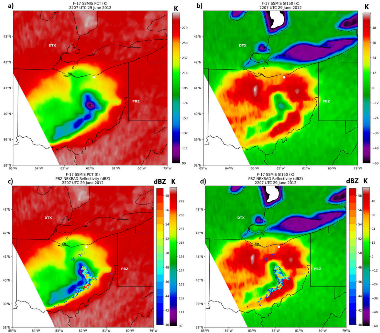
Figure 11. F-17 SSMIS (a) polarization corrected temperature (PCT) and (b) 150 GHz scattering index (SI150), in degrees Kelvin (K), at 2207 UTC 29 June 2012. (c) and (d) display the product imagery with overlying Pittsburgh, Pennsylvania NEXRAD reflectivity (dBZ). White circle marks the location of the Cleveland, Ohio MWRP. “DTX” and “PBZ” mark the location of the Detroit, Michigan and Pittsburgh NEXRAD stations, respectively.
