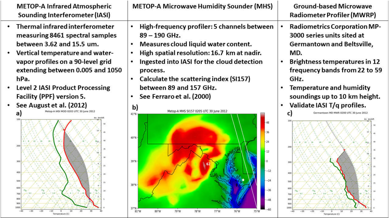
Figure 2. A summary of observational remote sensing data applied for the study and analysis of the June 2012 North American Derecho. (a, c) are examples of vertical sounding profiles generated from IASI and MWRP datasets, respectively, for diagnosing the pre-convective environment, while (b) is an example of a satellite-derived microwave image product that identifies signatures associated with a derecho-producing convective system (DCS).
