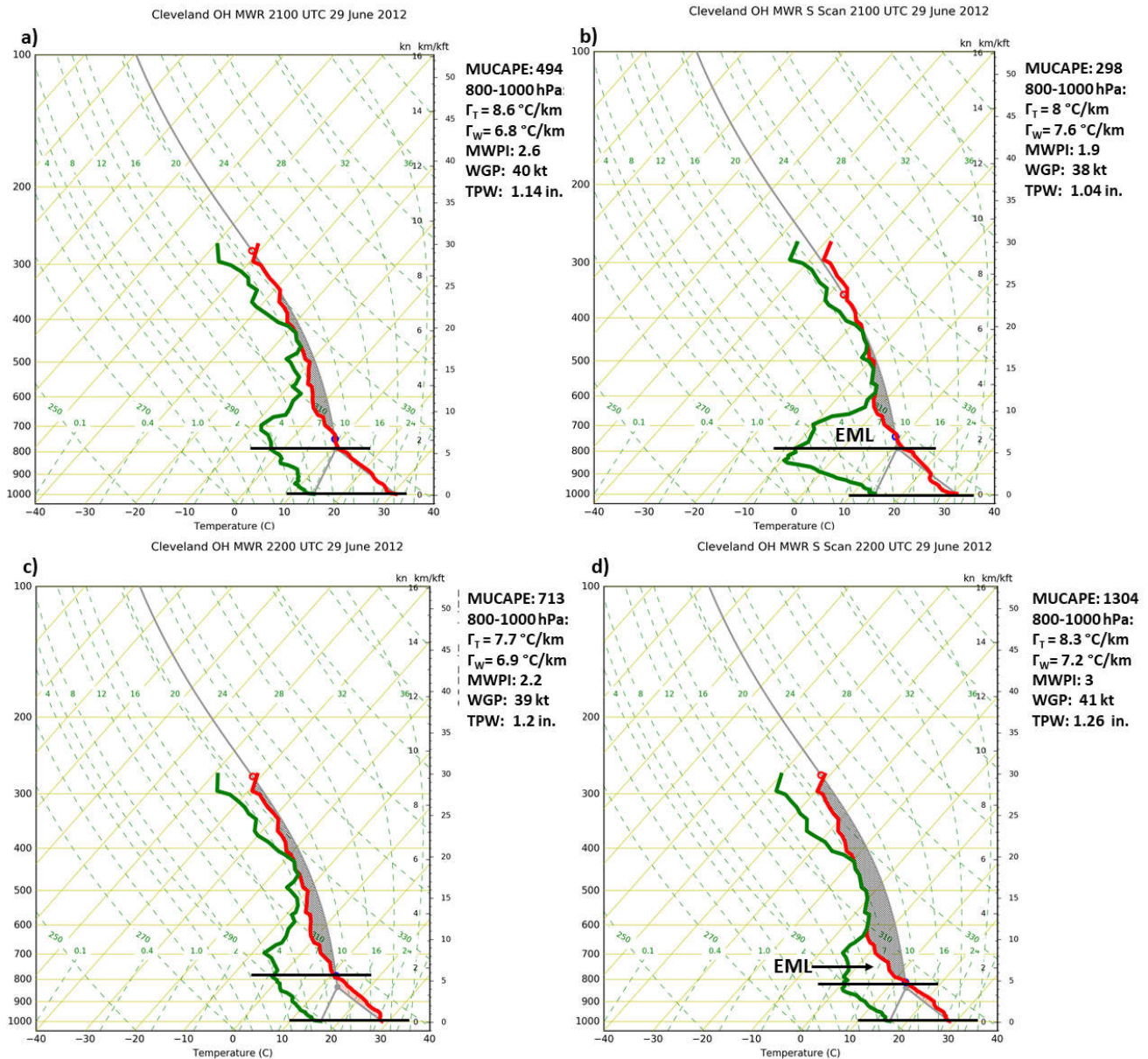
Figure 9. Ground-based sounding profile retrievals from the Cleveland, Ohio microwave radiometer (MWR) on 29 June 2012: (a) zenith at 2100 UTC, (b) south scan at 2100 UTC, (c) zenith at 2200 UTC, and (d) south scan at 2200 UTC. Red curves and green curves represent the temperature and dewpoint soundings in degrees Celsius ( ^\circ\text{C} ), respectively. “MUCAPE” is most unstable parcel CAPE in \text{J kg}^{-1} , “MWPI” represents the Microburst Windspeed Potential Index (Pryor 2015), “WGP” represents wind gust potential derived from the MWPI in knots (kt), and “EML” represents the elevated mixed layer. \Gamma_T and \Gamma_w represent dry-bulb temperature and wet-bulb temperature lapse rates, respectively.
