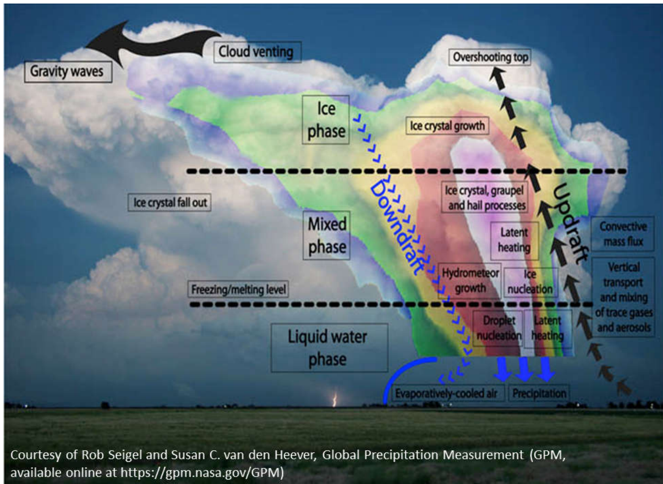
Figure 1. Conceptual model of a deep convective storm with the potential to generate intense downdrafts and damaging downburst winds.
