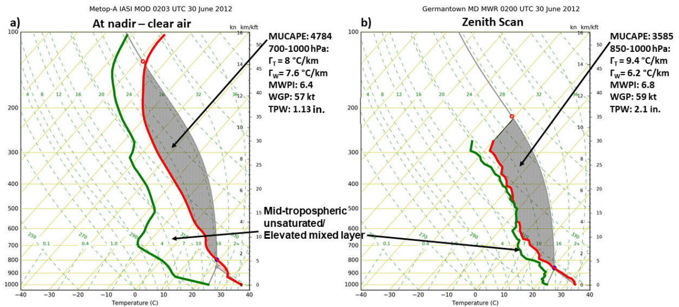
Figure 14. (a) Modified METOP-A IASI IR+MW sounding profile retrieved near Salisbury, Maryland at 0203 UTC 30 June 2012 as compared to (b) a ground-based sounding profile retrieval from the Germantown, Maryland microwave radiometer (MWR). Red curves and green curves represent the temperature and dewpoint soundings in degrees Celsius ( ^{\circ}\text{C} ), respectively. “MUCAPE” is most unstable parcel CAPE in \text{J kg}^{-1} , “MWPI” represents the Microburst Windspeed Potential Index (Pryor 2015), “WGP” represents wind gust potential derived from the MWPI in knots (kt), and “TPW” represents total precipitable water in inches (in). \Gamma_T and \Gamma_w represent dry-bulb temperature and wet-bulb temperature lapse rates, respectively.
