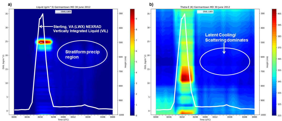
Figure 18. 0200 to 0400 UTC 30 June 2012 Hovmöller diagrams of (a) liquid density (g m -3 ) and (b) equivalent potential temperature (θ e in degrees Kelvin (K)) as derived from Germantown, Maryland MWRP. Sterling, Virginia NEXRAD DVIL is plotted over the diagrams at corresponding MWRP retrieval times.
