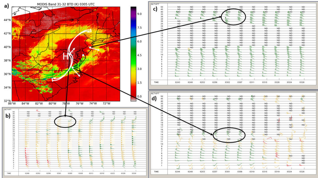
Figure 20. (a) TERRA MODIS split window IR brightness temperature difference product image at 0305 UTC 30 June 2012 compared to VAD wind profiles, in knots (kt), from (b) Sterling, Virginia, (c) Philadelphia, Pennsylvania (Manchester Township, New Jersey, and (d) Norfolk-Richmond, Virginia (Wakefield, Virginia) NEXRAD stations, surrounding the retrieval time of the MODIS image.
