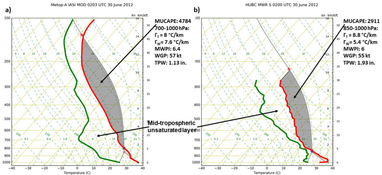
Figure 15. (a) Modified METOP-A IASI IR+MW sounding profile retrieved near Salisbury, Maryland at 0203 UTC 30 June 2012 as compared to (b) a ground-based sounding profile retrieval from the Howard University, Beltsville, Maryland (HUBC) microwave radiometer (MWR). Red curves and green curves represent the temperature and dewpoint soundings in degrees Celsius ( ^{\circ}\text{C} ), respectively. “MUCAPE” is most unstable parcel CAPE in \text{J kg}^{-1} , “MWPI” represents the Microburst Windspeed Potential Index (Pryor 2015), “WGP” represents wind gust potential derived from the MWPI in knots (kt), and “TPW” represents total precipitable water in inches (in). \Gamma_T and \Gamma_W represent dry-bulb temperature and wet-bulb temperature lapse rates, respectively.
