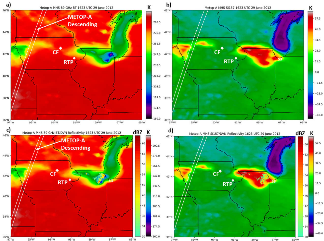
Figure 8. METOP-A MHS (a) 89 GHz channel brightness temperature (TB, degrees Kelvin (K)) image and (b) 157 GHz scattering index (SI157) at 1623 UTC 29 June 2012. (c, d) as in (a, b) with overlying Davenport, Iowa (DVN) NEXRAD reflectivity (dBZ) measurements. “CF” marks the location of the Cedar Falls, Iowa MWRP, “RTP” is the location of the IASI retrieval over Tipton, Iowa, and “53” is the location of the first severe wind report of the event ( 27 \text{ m s}^{-1} (53 kt)) recorded at Burns Harbor, Indiana. White lines mark the 29 June descending node METOP-A orbit (nadir) tracks.
