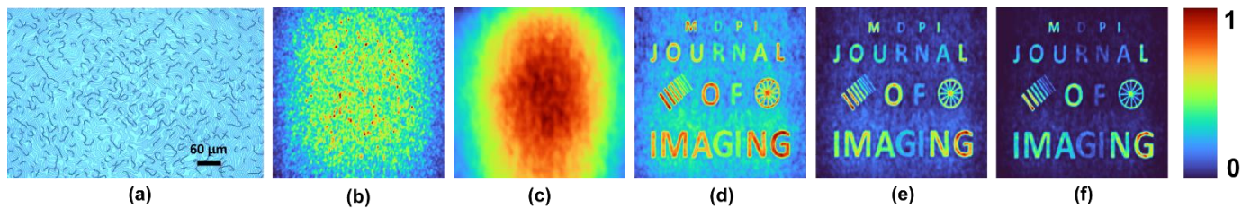
Figure 7. (a) Optical microscope image of the central part of the QRL fabricated using electron beam lithography. (b) Recorded PSF, (c) object's response pattern. Reconstruction results using (d) NLR ( p=1 ), (e) NLR ( p=2 ) and (f) NLR ( p=3 ).
