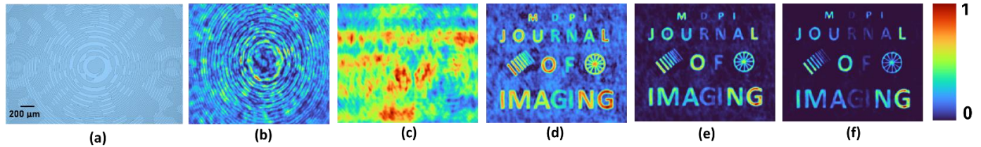
Figure 15. (a) Optical microscope image of the randomly multiplexed bifocal diffractive lenses. (b) Recorded PSF, (c) object's response pattern. Reconstruction results using (d) NLR ( p=1 ), (e) NLR ( p=2 ) and (f) NLR ( p=3 ) for FINCH with spatial random multiplexing configuration.
