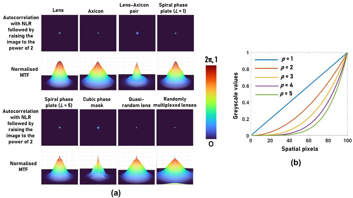
Figure 3. (a) Autocorrelation with NLR followed by raising the image to the power of p = 2 and their respective MTF profiles. (b) The influence of p on a grayscale slope.
