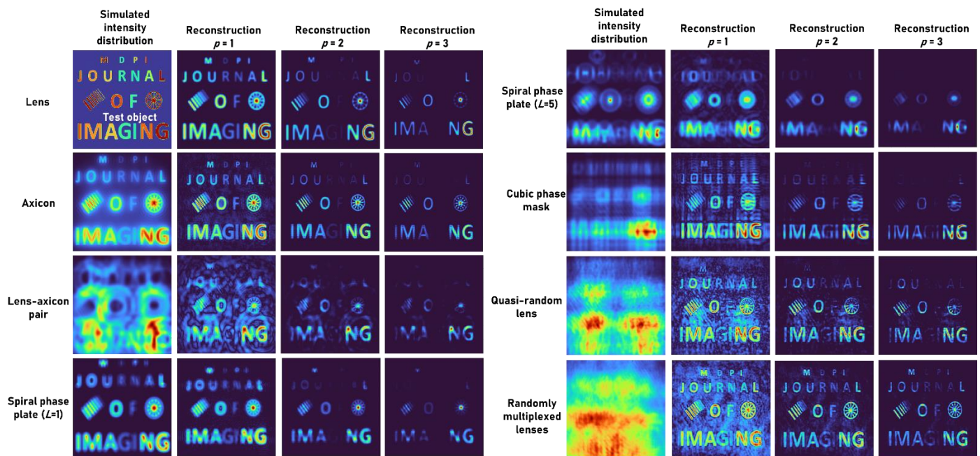
Figure 4. Simulated intensity distribution for a test object and the reconstruction results for p=1, 2 and 3 .
