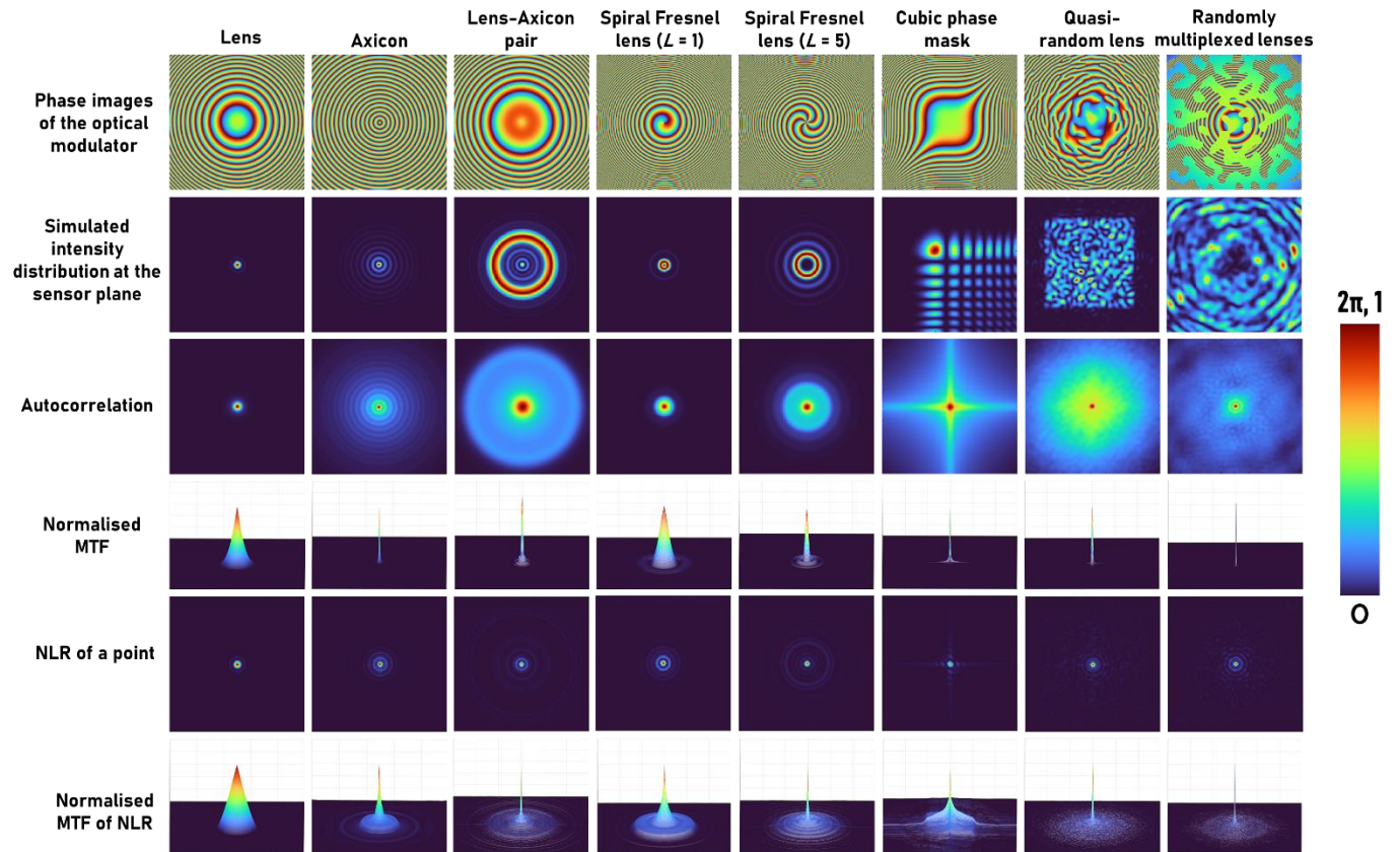
Figure 2. Comparison between different phase modulators according to functions and distributions that related to image reconstruction and resolution.
