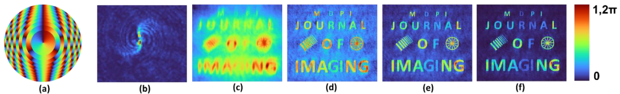
Figure 16. (a) Phase image of the multifunctional DOE. (b) Recorded PSF, (c) object's response pattern. Reconstruction results using (d) NLR ( p=1 ), (e) NLR ( p=2 ) and (f) NLR ( p=3 ) for double-helix beam with rotating PSF.
