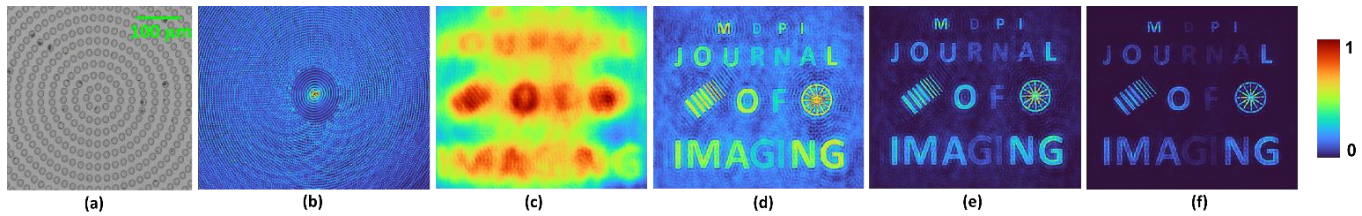
Figure 9. (a) Image of the photon sieve axicon fabricated using femtosecond ablation. (b) Recorded PSF, (c) object's response pattern. Reconstruction results using (d) NLR ( p=1 ), (e) NLR ( p=2 ) and (f) NLR ( p=3 ).
