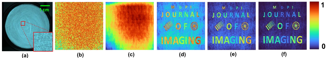
Figure 8. (a) Image of the QRL fabricated using lens grinding with sandpaper. (b) Recorded PSF, (c) object's response pattern. Reconstruction results using (d) NLR ( p=1 ), (e) NLR ( p=2 ) and (f) NLR ( p=3 ).
