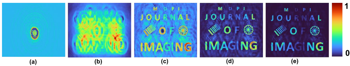
Figure 13. (a) Recorded PSF, (b) object's response pattern. Reconstruction results using (c) NLR ( p=1 ), (d) NLR ( p=2 ) and (e) NLR ( p=3 ) for lens-axicon pair.
