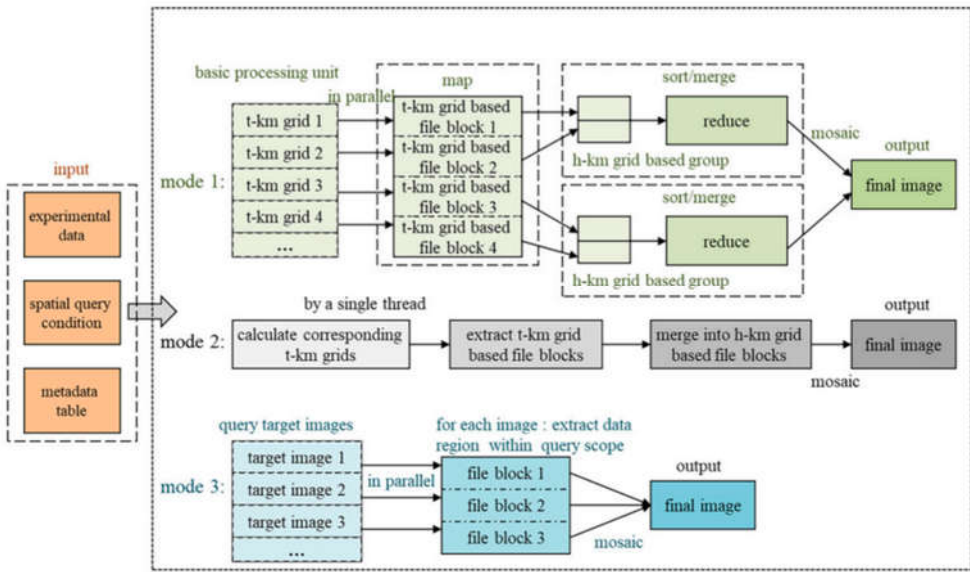
Figure 15. Process of Three Modes for data extraction.
