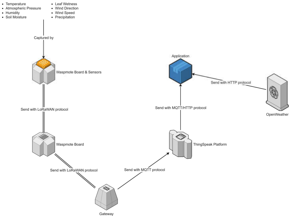
Figure 12. Big Data Architecture and the IoT [52].
