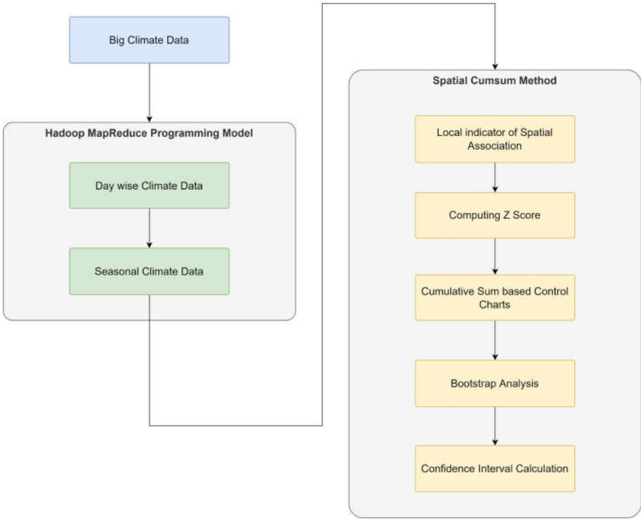
Figure 13. Proposed Big Data Architecture for climate change detection [63].
