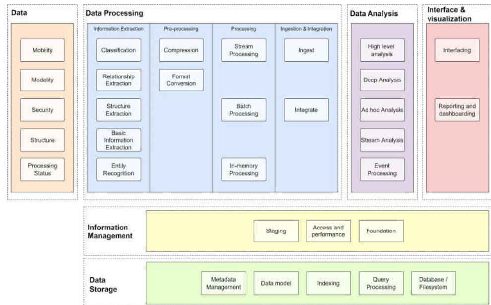
Figure 1. The General architecture of Big Data.
