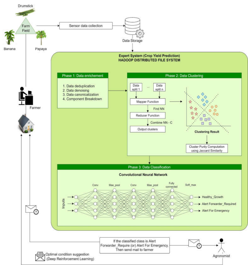
Figure 10. Big Data architecture for crop yield prediction and fertilizer management [49].
