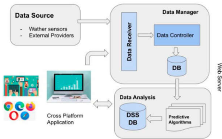
Figure 9. DSS LANDS Architecture for Forecasting Crop Disease [62].
