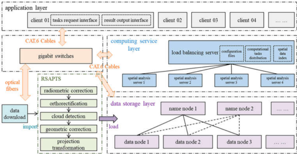
Figure 14. Big Data architecture to monitor dryness [56].
