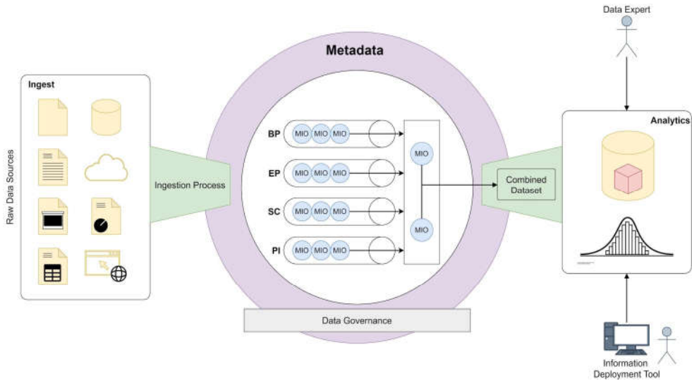
Figure 6. Data Lake is used by CSA [48].
