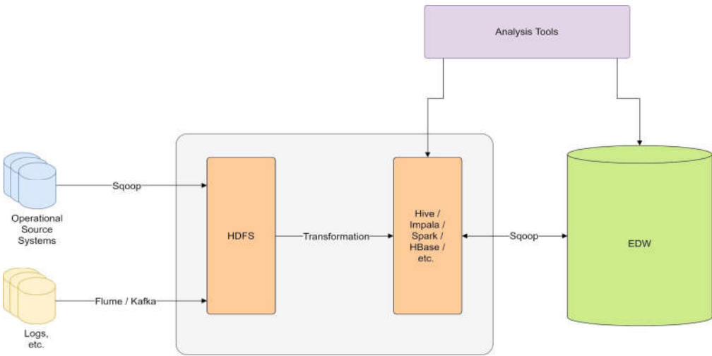
Figure 11. Climate Big Data architecture [44].
