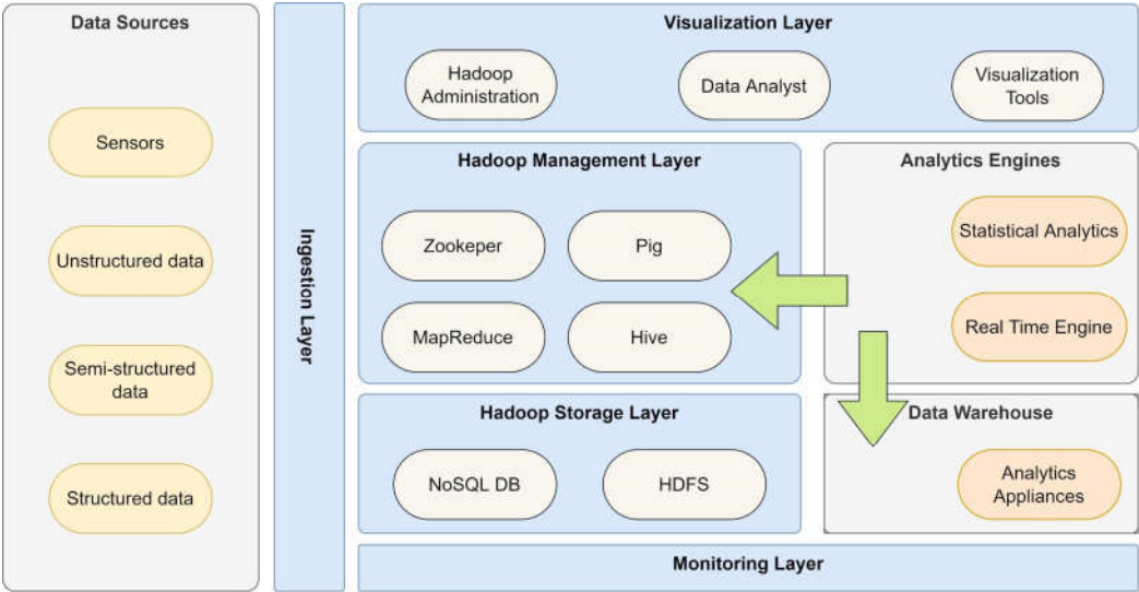
Figure 7. Proposed Big Data architecture for atmospheric composition monitoring [39].
