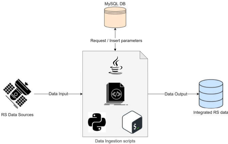
Figure 8. Ingest process for Big Data atmospheric composition monitoring system [39].
