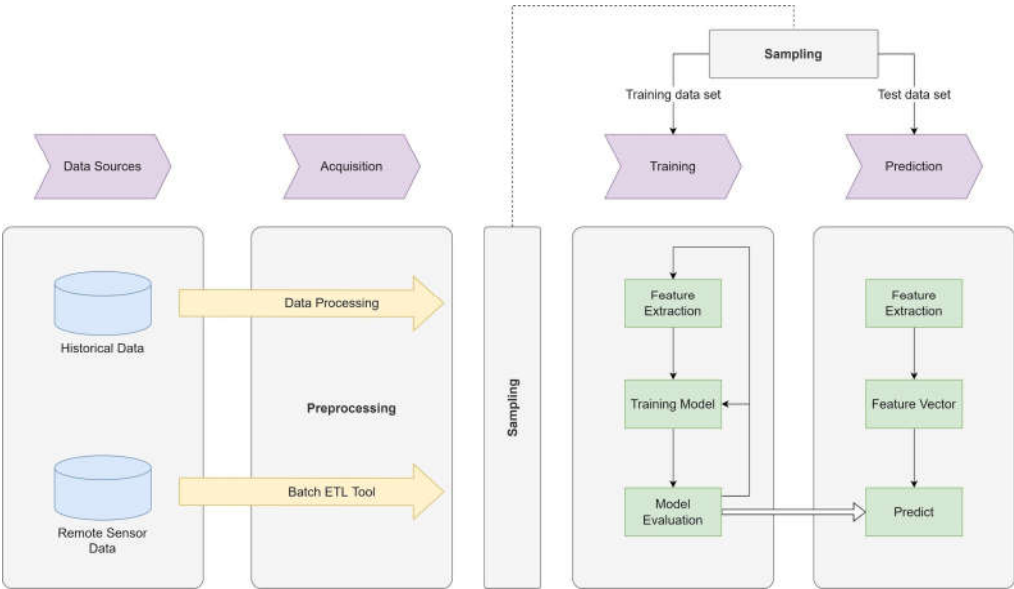
Figure 16. Big Data architecture for vegetation monitoring [64].
