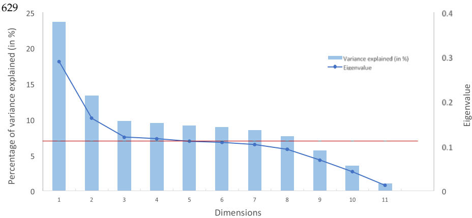
Figure 4. Scree plot of variance explained by dimension from a MCA (In red, eigenvalue of 0.11).
