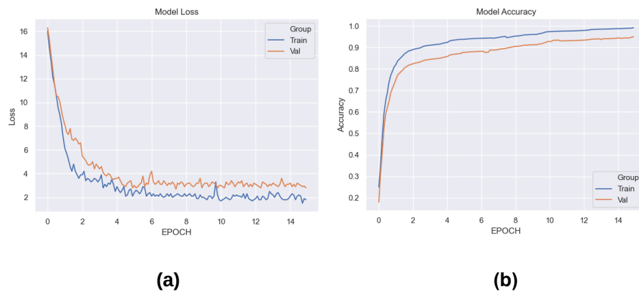
Figure 7. Training and validating process of proposed model:(a)Loss, (b)Accuracy.
