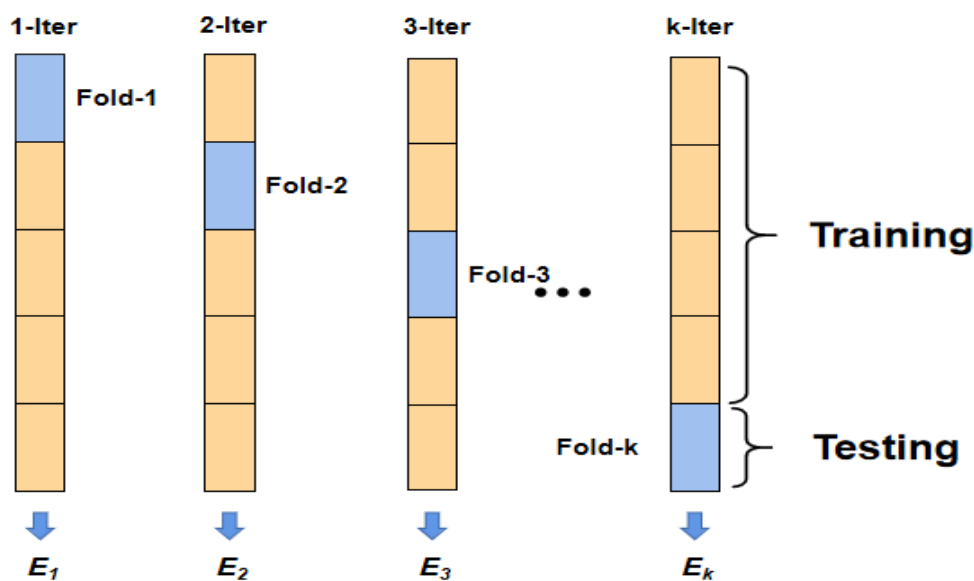
Figure 6. K-fold cross validation.
