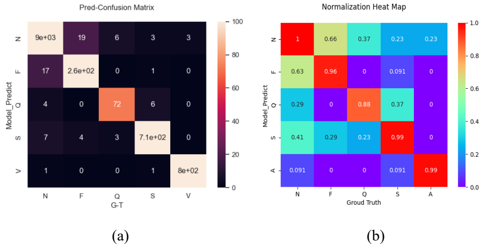
Figure 8. Prediction performance of proposed model in the MIT-BIH arrhythmia test set:(a)Confusion Matrix, (b)Normalization Heat Map
