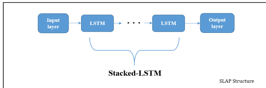
Figure 5. Stacked-LSTM architecture for prediction.
